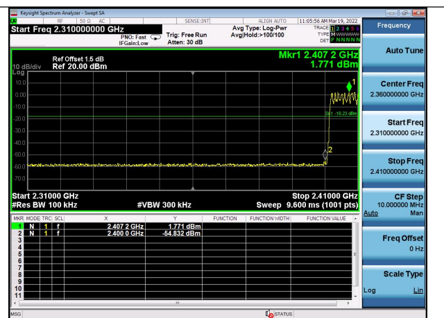
8DPSK Hopping Band edge-Left side
