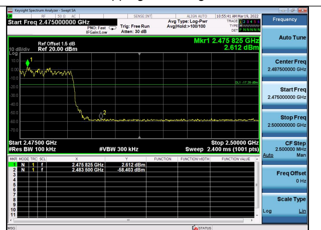
8DPSK Hopping Band edge-Right side
