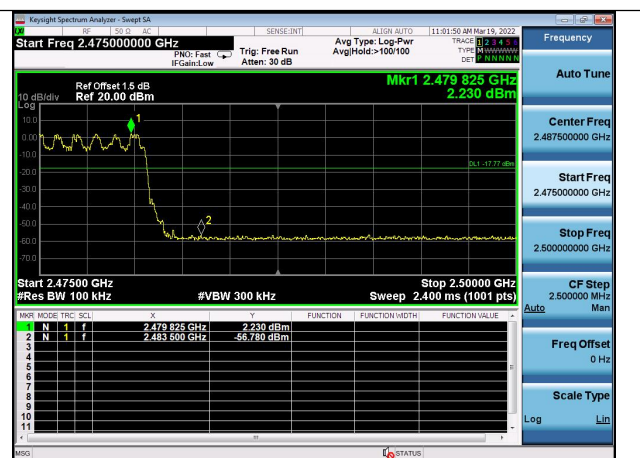
\pi /4-DQPSK Hopping Band edge-Right side
