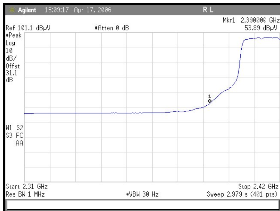
Plot 12. OFDM Radiated Restricted Band 2310 MHz – 2390 MHz Average
