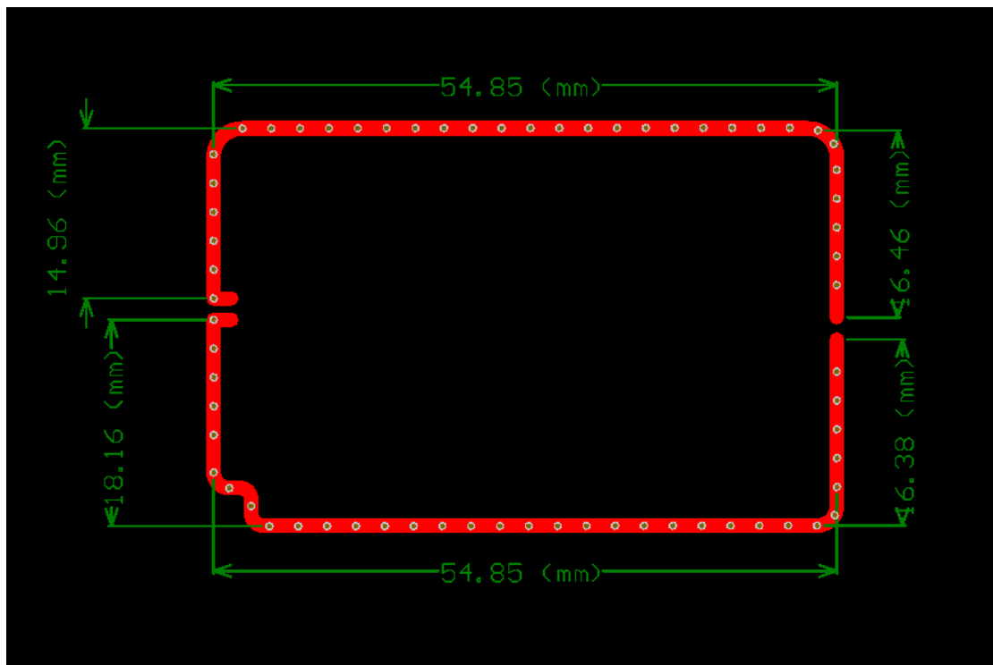
Picture of antenna
