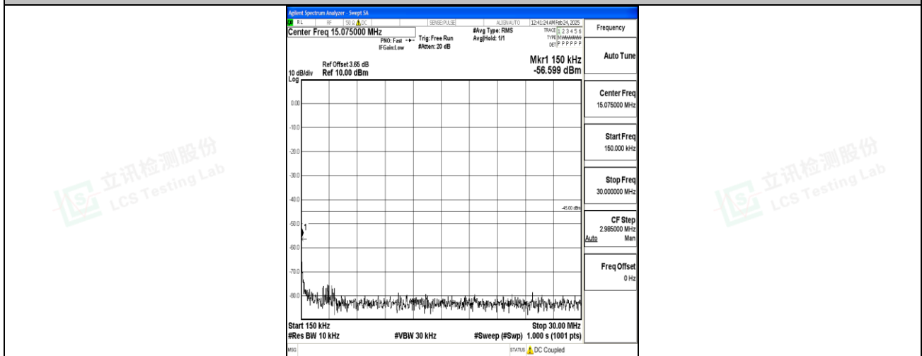
Band7_10MHz_16QAM_21400_1RB#0_0.15~30_0.15~30
