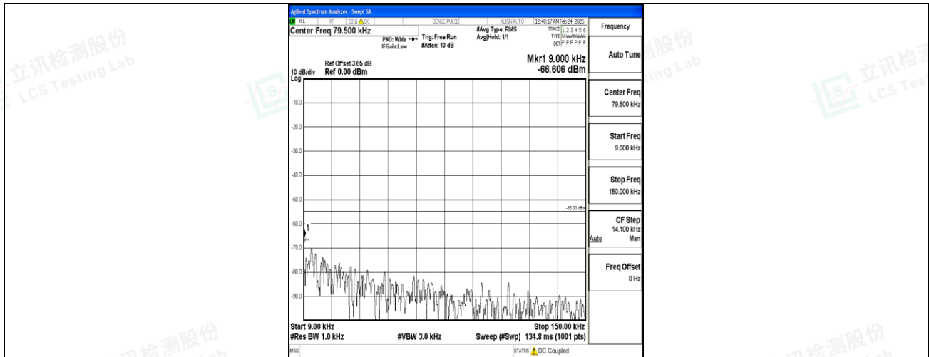
Band7_10MHz_16QAM_21100_1RB#0_0.009~0.15_0.009~0.15
