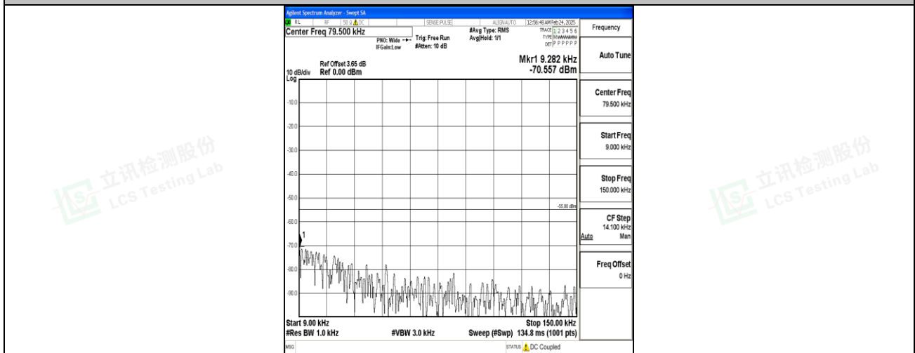
Band7_20MHz_QPSK_21350_1RB#0_0.009~0.15_0.009~0.15
