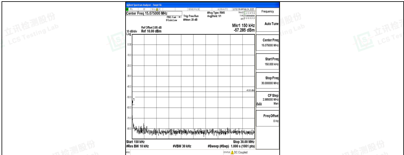
Band7_20MHz_16QAM_20850_1RB#0_0.15~30_0.15~30
