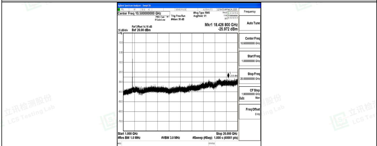
Band7_20MHz_QPSK_21100_1RB#0_1000~20000_1000~20000
