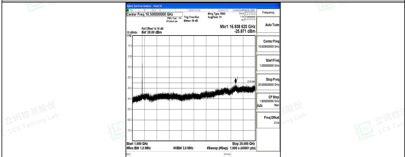
Band7_15MHz_QPSK_21100_1RB#0_1000~20000_1000~20000
