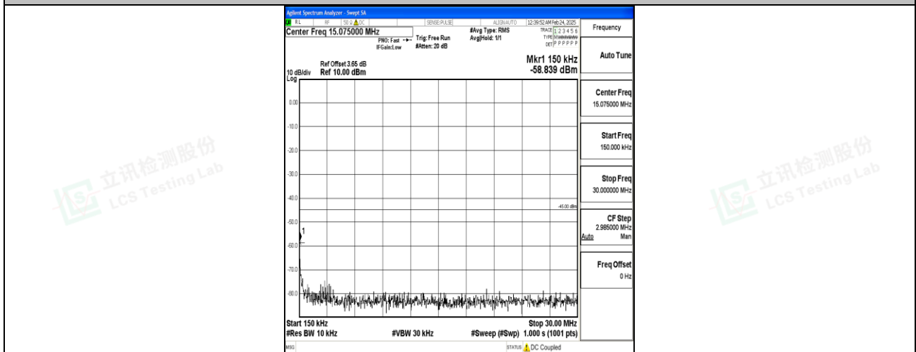
Band7_10MHz_QPSK_21100_1RB#0_0.15~30_0.15~30
