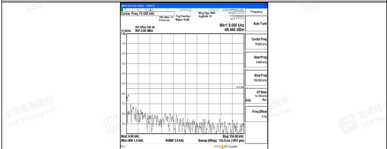
Band7_15MHz_QPSK_21100_1RB#0_0.009~0.15_0.009~0.15
