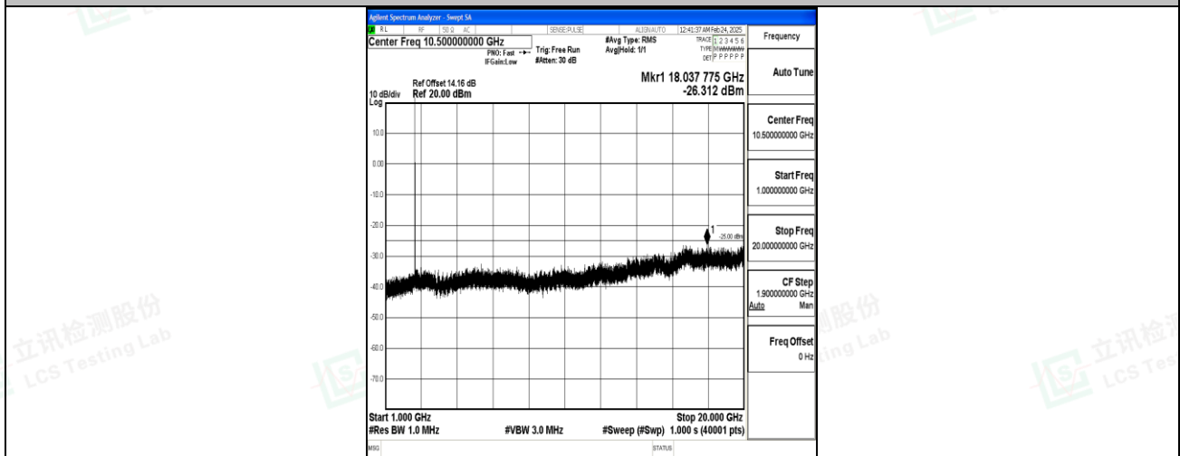
Band7_10MHz_16QAM_21400_1RB#0_1000~20000_1000~20000
