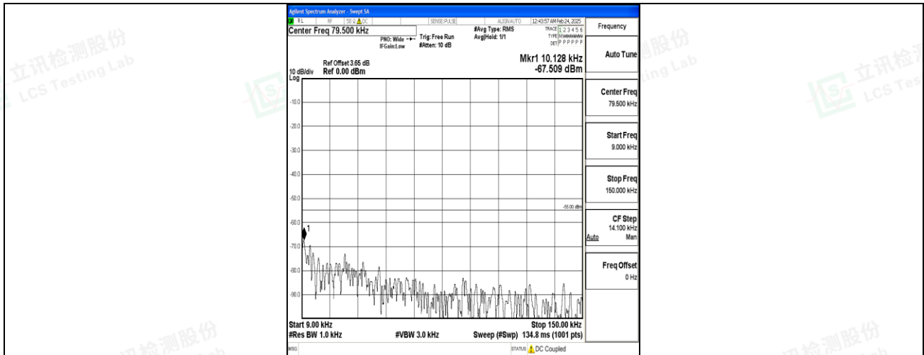
Band7_15MHz_QPSK_20825_1RB#0_0.009~0.15_0.009~0.15
