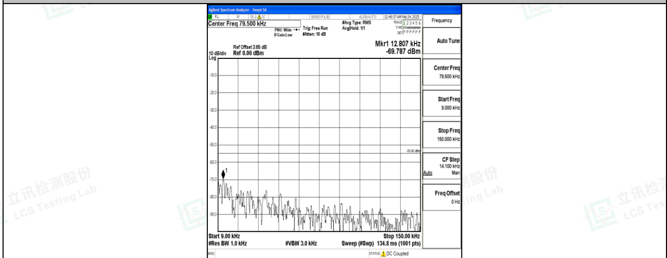
Band7_15MHz_16QAM_21375_1RB#0_0.009~0.15_0.009~0.15
