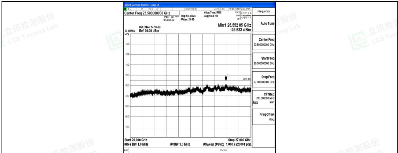
Band7_10MHz_QPSK_21400_1RB#0_20000~27000_20000~27000
