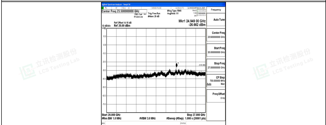
Band7_15MHz_16QAM_21375_1RB#0_20000~27000_20000~27000
