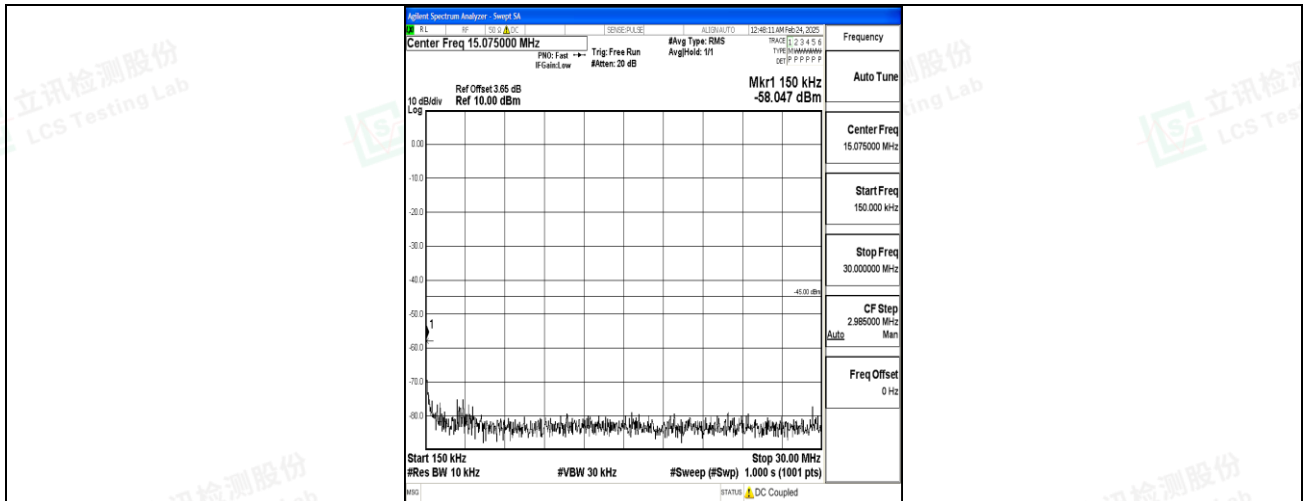
Band7_15MHz_QPSK_21375_1RB#0_0.15~30_0.15~30
