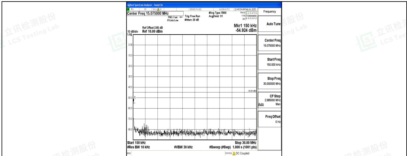
Band7_10MHz_QPSK_21400_1RB#0_0.15~30_0.15~30
