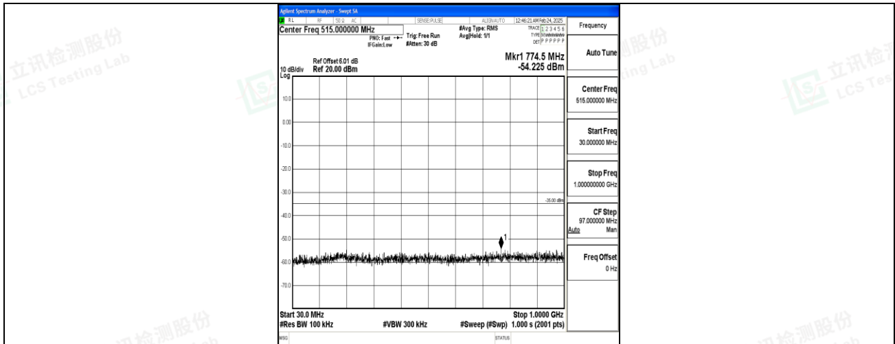
Band7_15MHz_QPSK_21100_1RB#0_30~1000_30~1000
