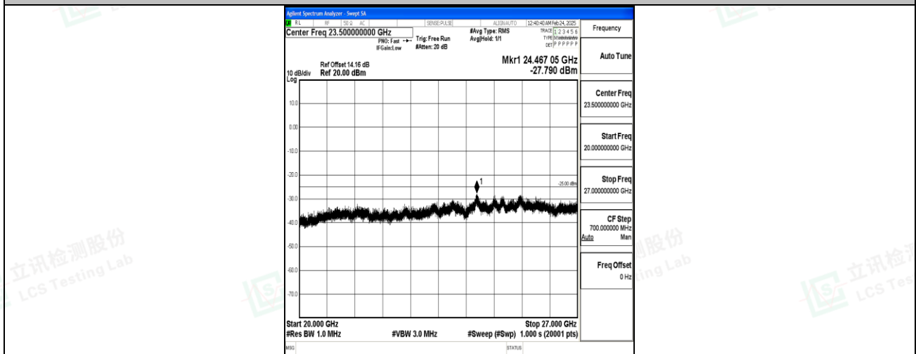
Band7_10MHz_16QAM_21100_1RB#0_20000~27000_20000~27000
