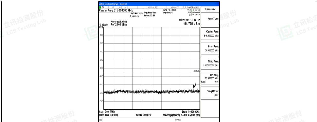
Band7_20MHz_16QAM_21350_1RB#0_30~1000_30~1000
