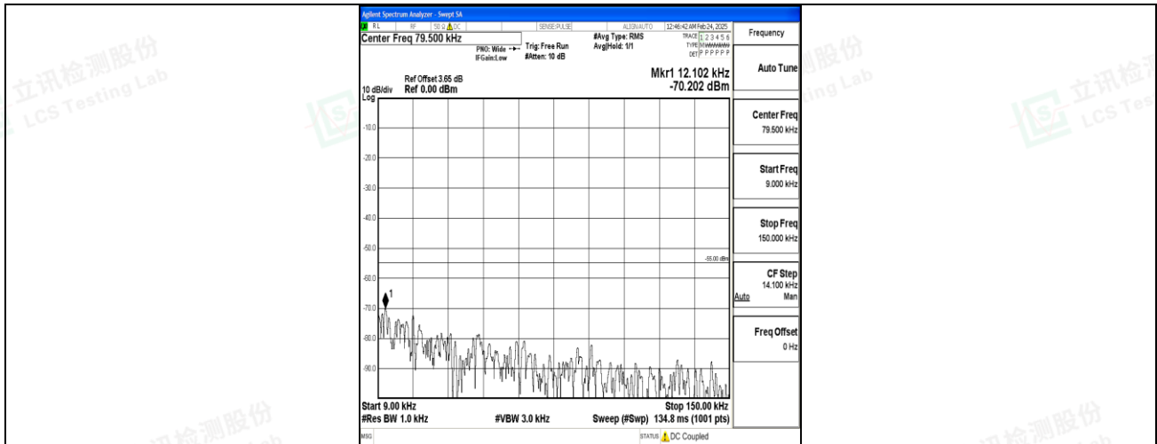
Band7_15MHz_16QAM_21100_1RB#0_0.009~0.15_0.009~0.15
