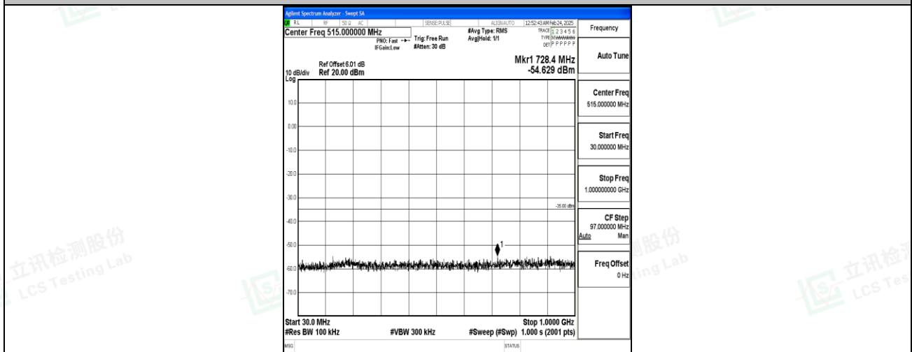
Band7_20MHz_16QAM_20850_1RB#0_30~1000_30~1000
