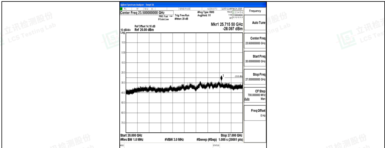
Band7_20MHz_QPSK_21350_1RB#0_20000~27000_20000~27000
