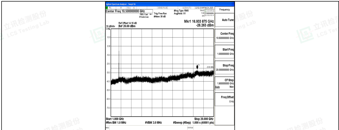
Band7_20MHz_QPSK_20850_1RB#0_1000~20000_1000~20000
