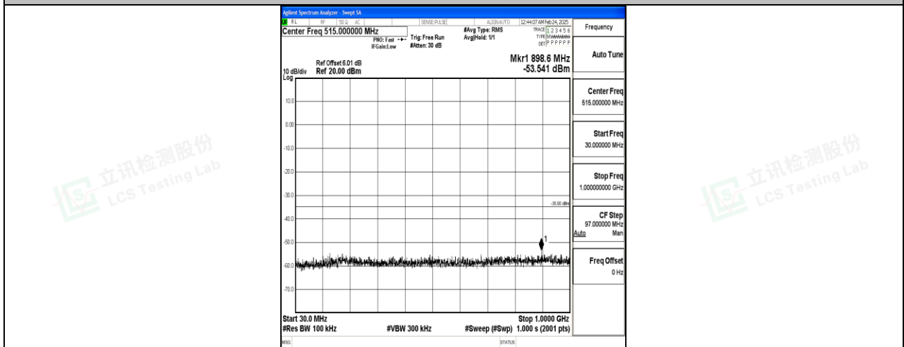
Band7_15MHz_QPSK_20825_1RB#0_30~1000_30~1000
