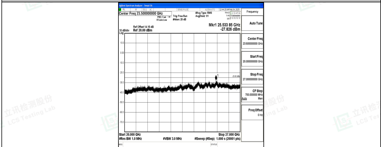
Band7_15MHz_QPSK_20825_1RB#0_20000~27000_20000~27000
