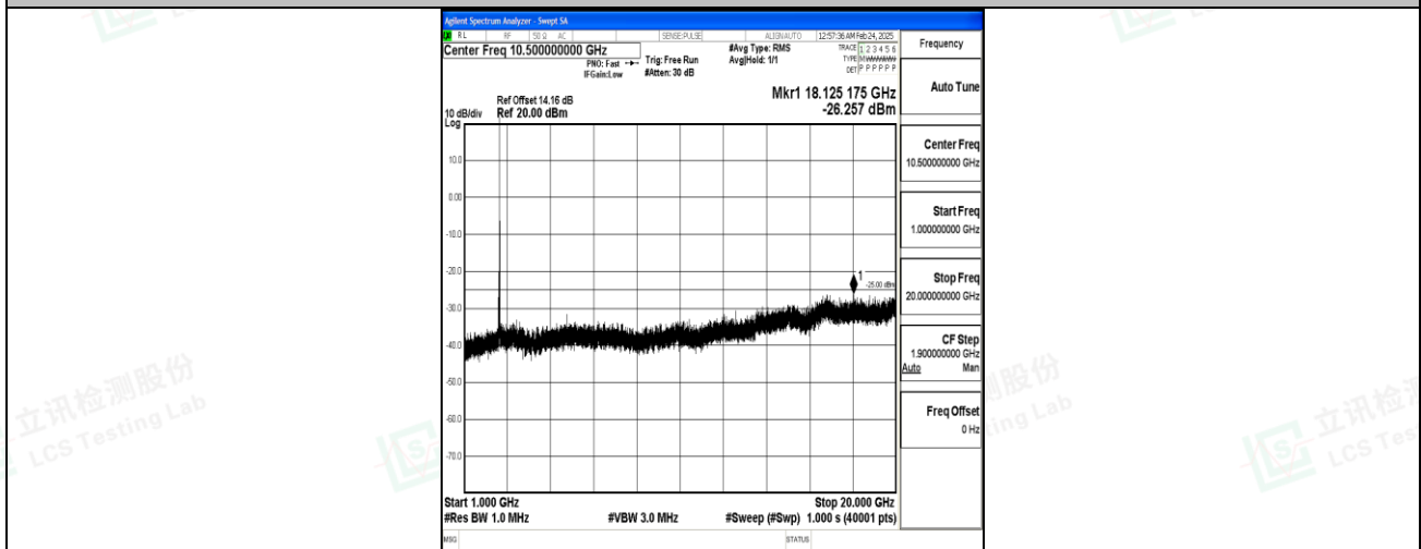
Band7_20MHz_16QAM_21350_1RB#0_1000~20000_1000~20000
