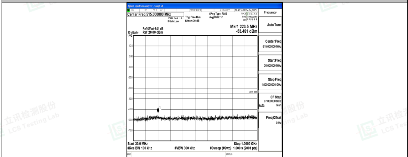
Band7_15MHz_QPSK_21375_1RB#0_30~1000_30~1000
