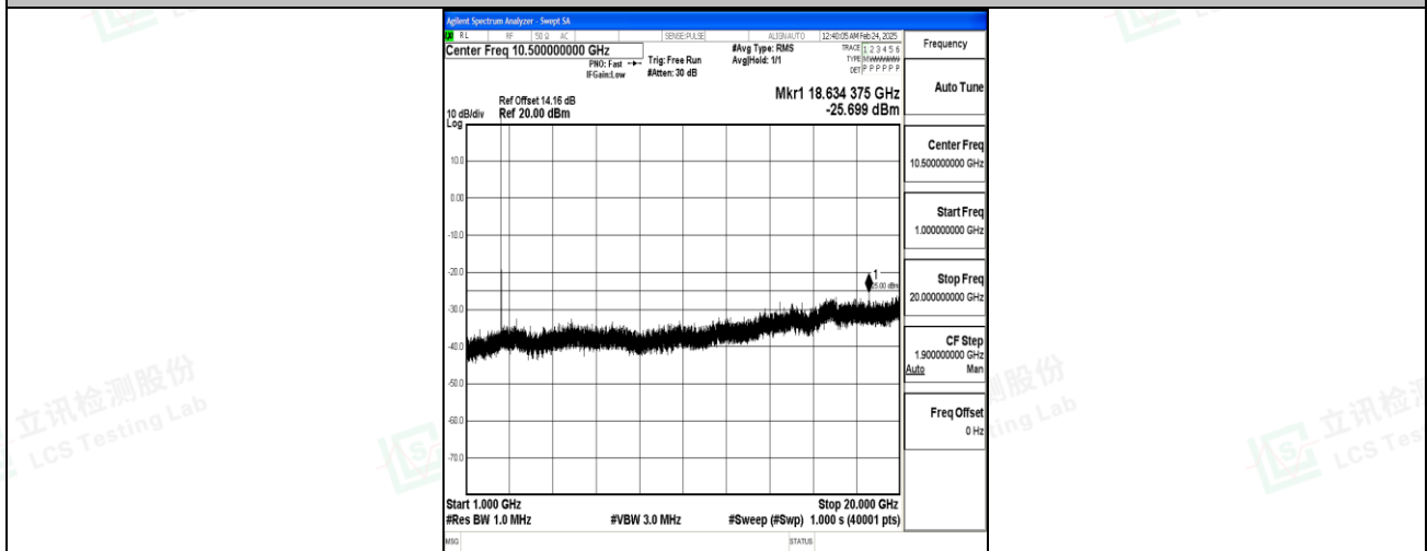
Band7_10MHz_QPSK_21100_1RB#0_1000~20000_1000~20000
