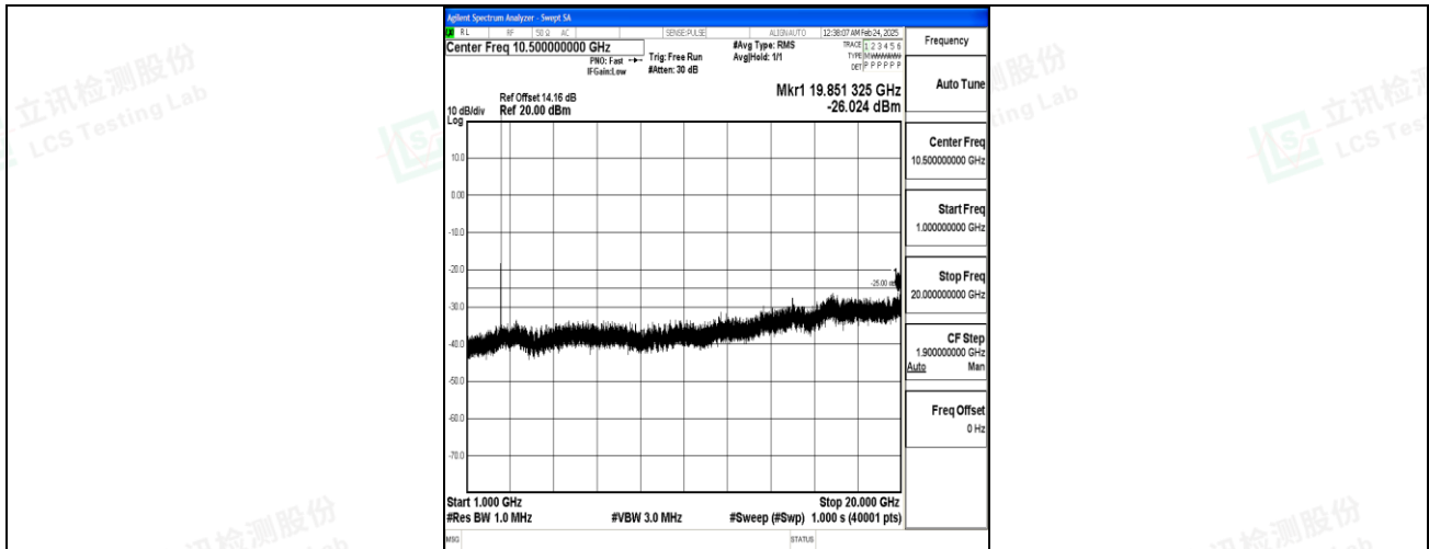
Band7_10MHz_QPSK_20800_1RB#0_1000~20000_1000~20000
