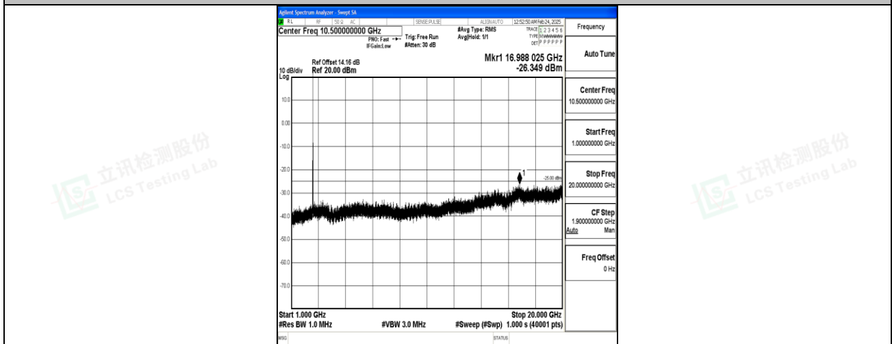
Band7_20MHz_16QAM_20850_1RB#0_1000~20000_1000~20000
