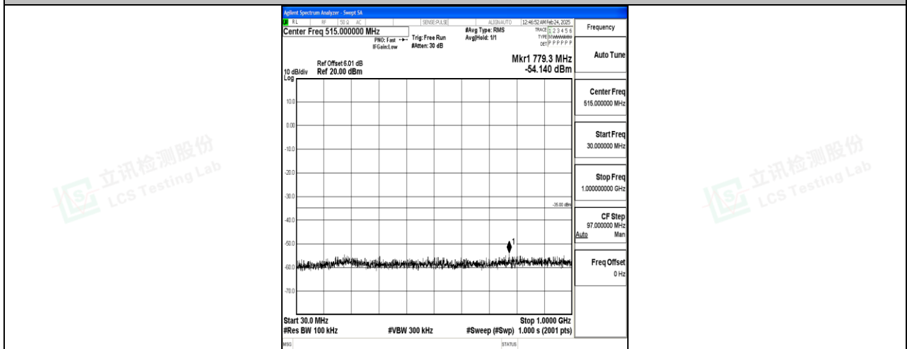
Band7_15MHz_16QAM_21100_1RB#0_30~1000_30~1000
