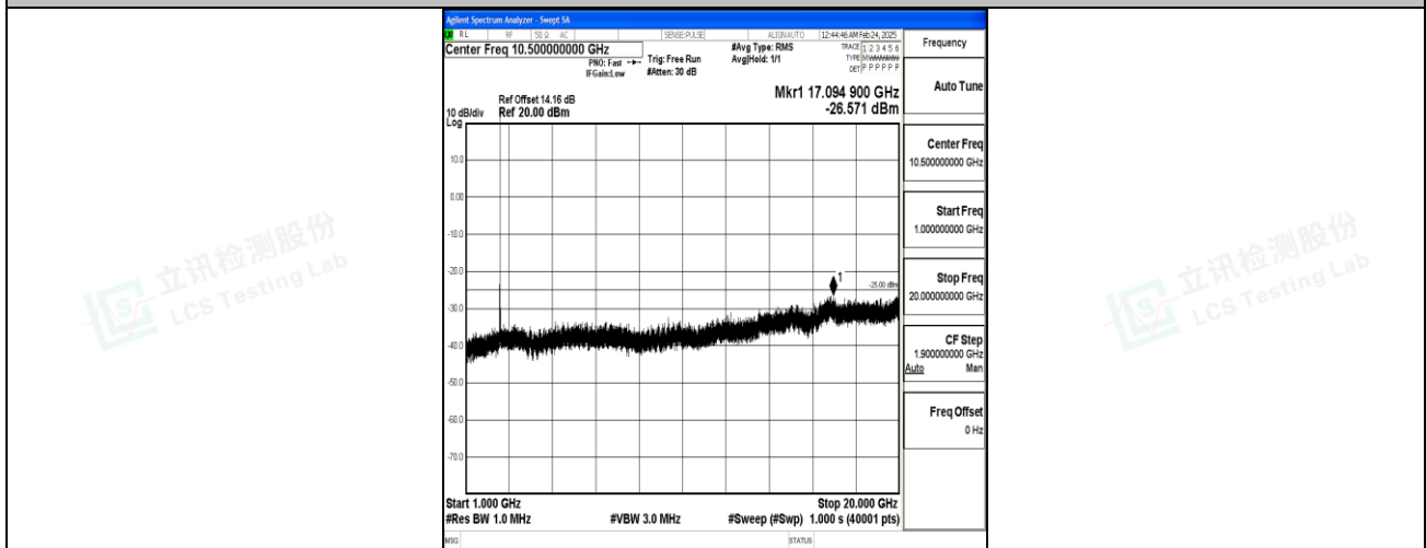
Band7_15MHz_16QAM_20825_1RB#0_1000~20000_1000~20000
