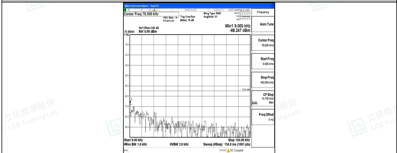
Band7_20MHz_16QAM_21350_1RB#0_0.009~0.15_0.009~0.15
