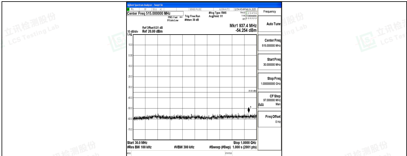
Band7_20MHz_QPSK_21100_1RB#0_30~1000_30~1000
