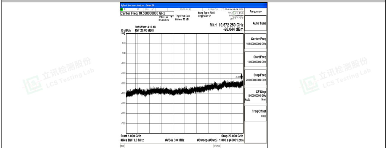
Band7_10MHz_16QAM_20800_1RB#0_1000~20000_1000~20000
