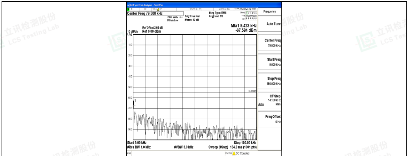
Band7_20MHz_16QAM_21100_1RB#0_0.009~0.15_0.009~0.15
