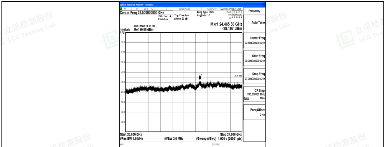
Band7_15MHz_16QAM_20825_1RB#0_20000~27000_20000~27000
