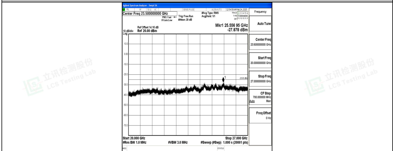
Band7_20MHz_QPSK_21100_1RB#0_20000~27000_20000~27000
