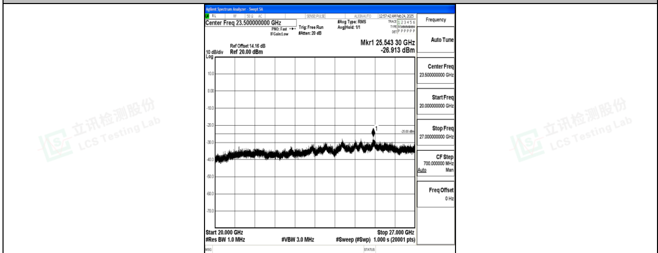
Band7_20MHz_16QAM_21350_1RB#0_20000~27000_20000~27000
