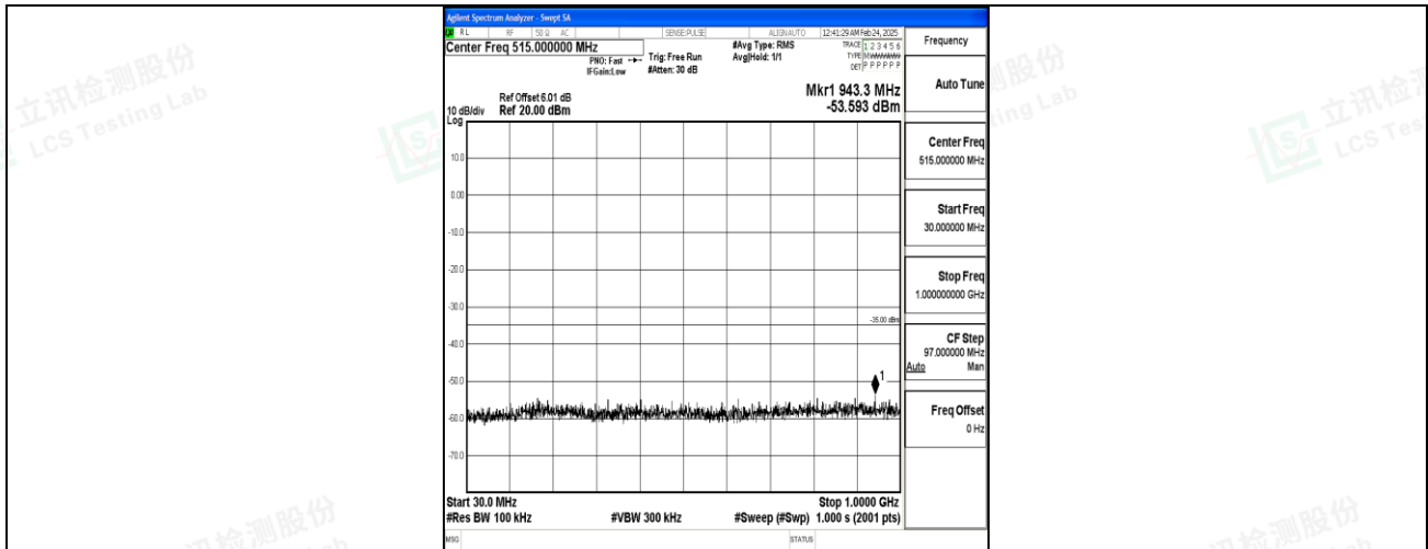
Band7_10MHz_16QAM_21400_1RB#0_30~1000_30~1000
