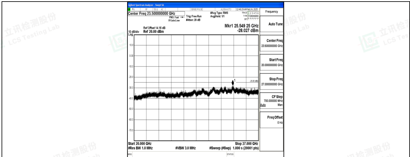
Band7_15MHz_QPSK_21375_1RB#0_20000~27000_20000~27000
