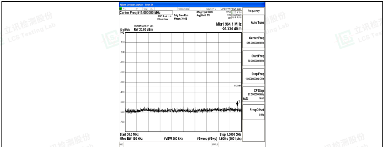
Band7_15MHz_16QAM_21375_1RB#0_30~1000_30~1000
