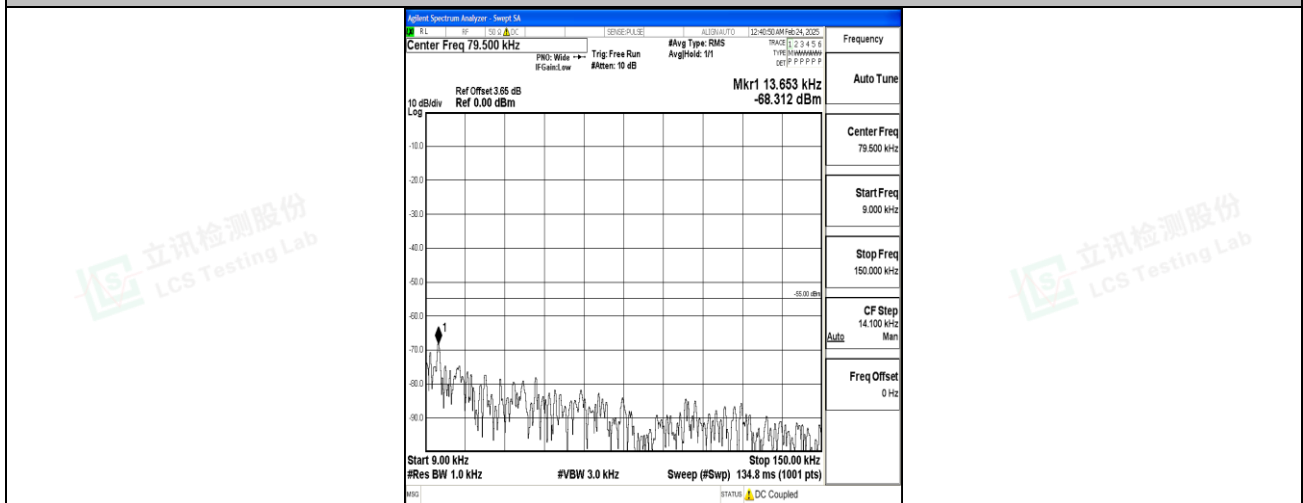
Band7_10MHz_QPSK_21400_1RB#0_0.009~0.15_0.009~0.15
