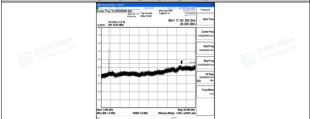
Band7_20MHz_QPSK_21350_1RB#0_1000~20000_1000~20000
