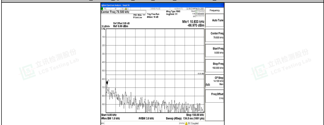
Band7_10MHz_16QAM_20800_1RB#0_0.009~0.15_0.009~0.15
