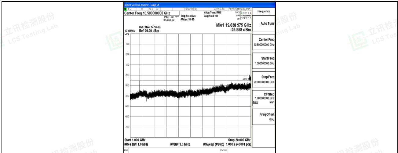
Band7_20MHz_16QAM_21100_1RB#0_1000~20000_1000~20000
