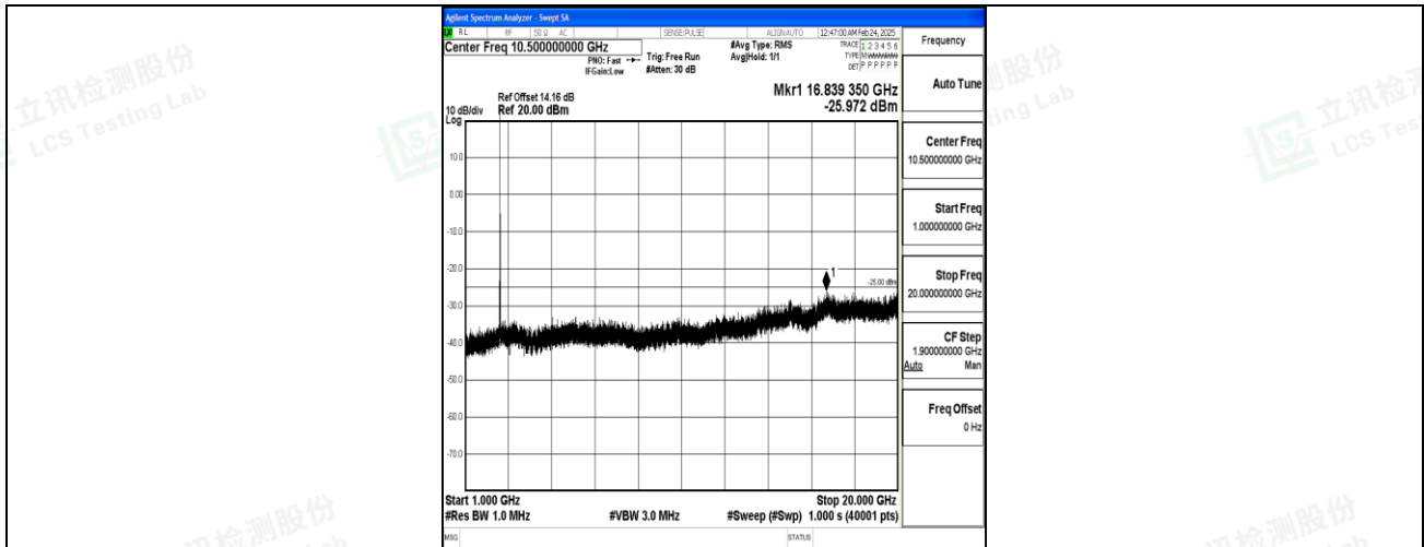
Band7_15MHz_16QAM_21100_1RB#0_1000~20000_1000~20000
