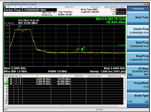
11AC40MIMO-Ant1-5230-PASS
