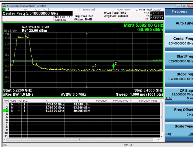
11AX20MIMO-Ant0-5240-PASS
