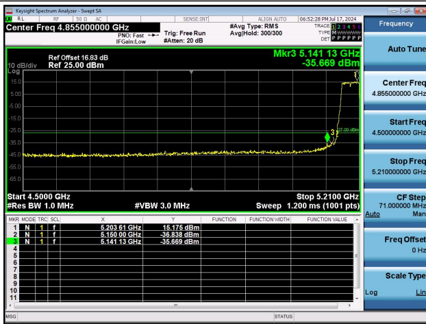
11AC40MIMO-Ant0-5190-PASS
