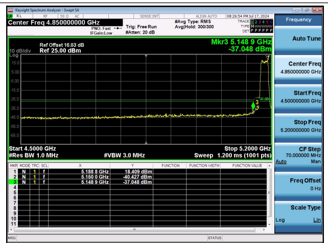
11AX20MIMO-Ant1-5180-PASS
