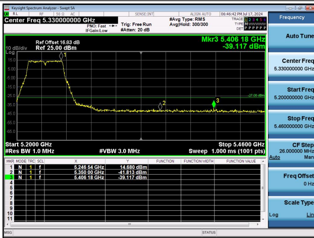
11N40MIMO-Ant0-5230-PASS
