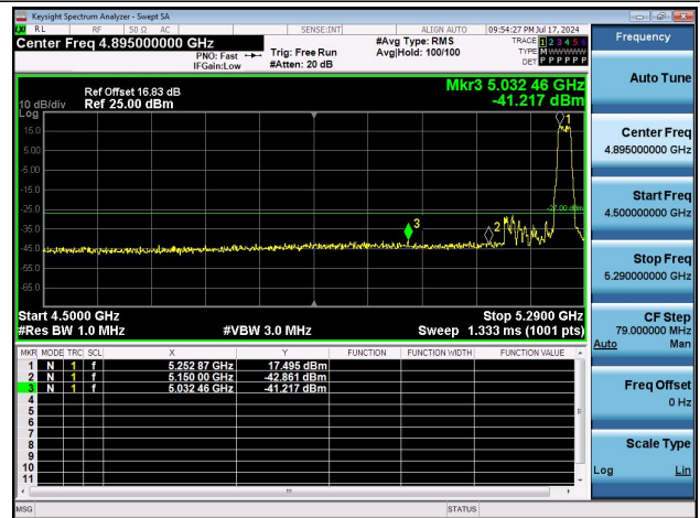
11N20MIMO-Ant1-5320-PASS
