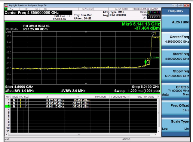
11AX40MIMO-Ant1-5190-PASS
