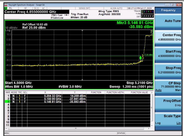
11N40MIMO-Ant1-5190-PASS
