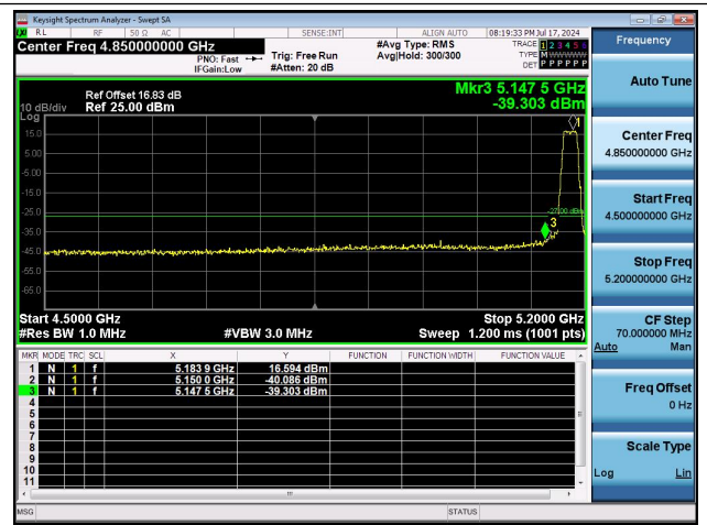
11AC20MIMO-Ant1-5180-PASS
