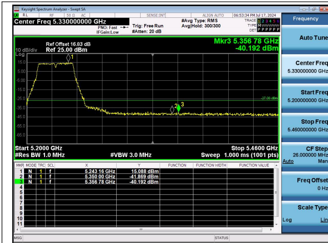
11AC40MIMO-Ant0-5230-PASS
