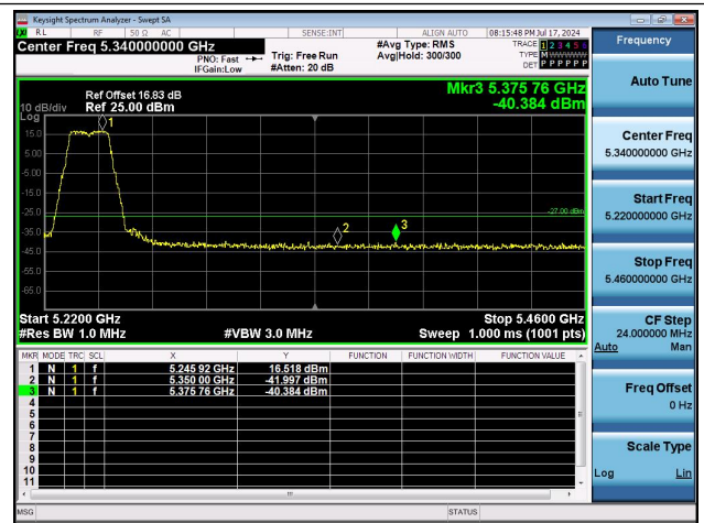
11N20MIMO-Ant1-5240-PASS
