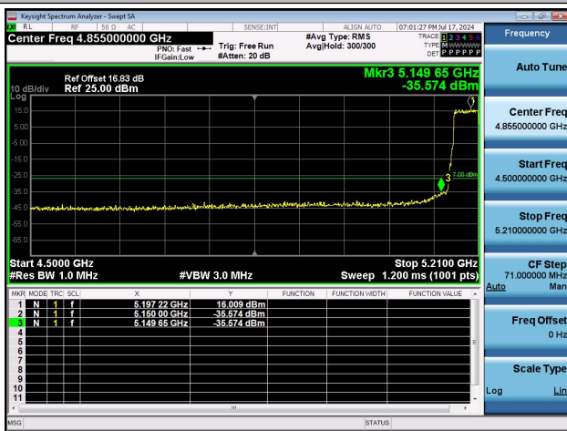
11AX40MIMO-Ant0-5190-PASS
