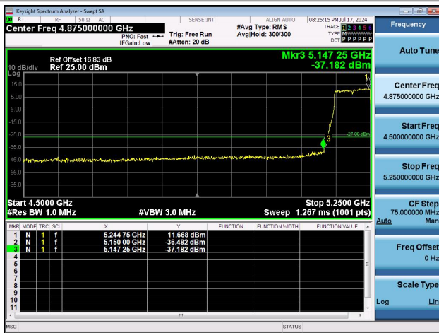
11AC80MIMO-Ant0-5210-PASS
