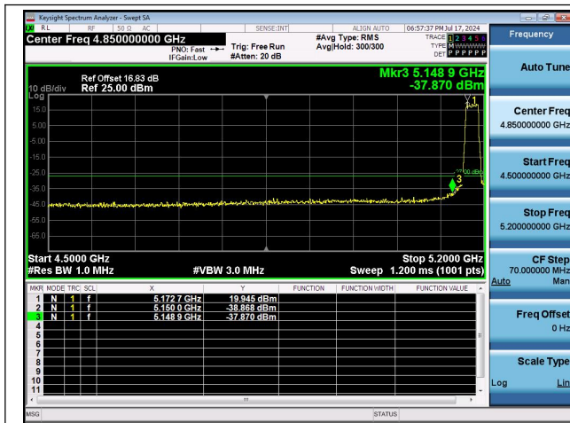
11AX20MIMO-Ant0-5180-PASS
