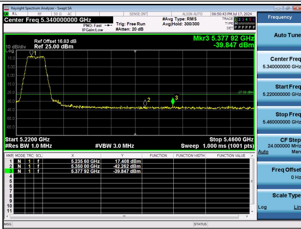
11AC20MIMO-Ant0-5240-PASS
