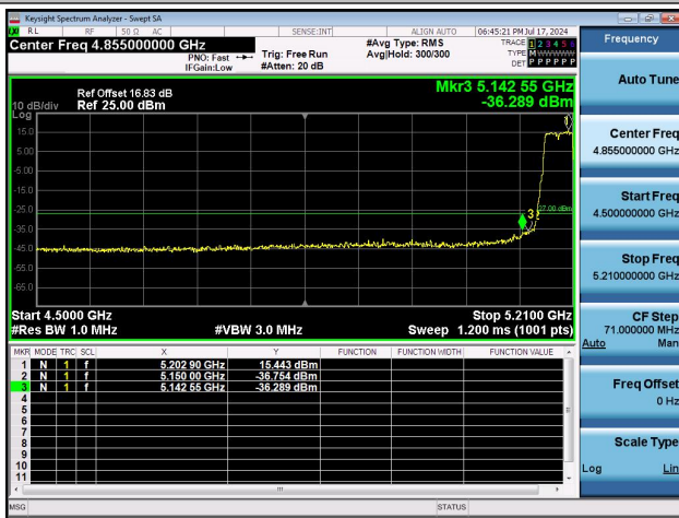
11N40MIMO-Ant0-5190-PASS
