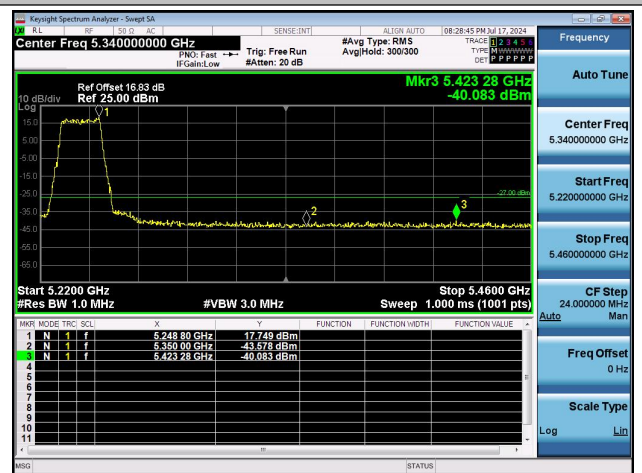
11AX20MIMO-Ant1-5240-PASS
