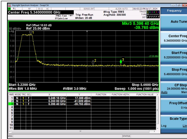
11N20MIMO-Ant0-5240-PASS
