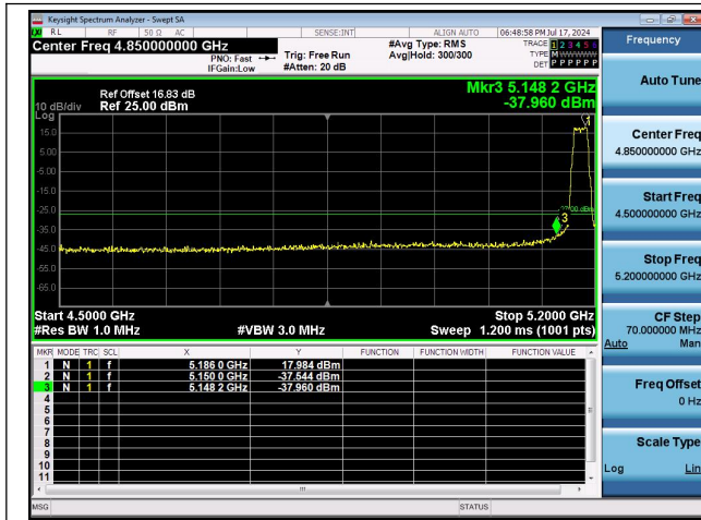
11AC20MIMO-Ant0-5180-PASS
