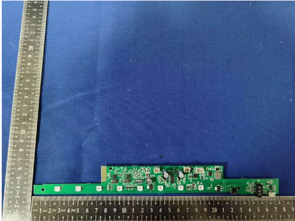
PCB Mainboard 1:
