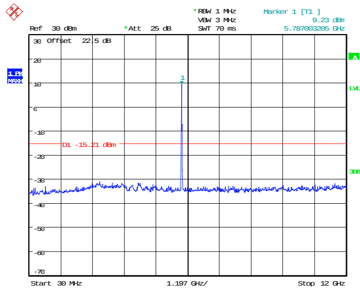
Fig. 13 Conducted Spurious Emission (802.11a, Ch157, Center Frequency)
