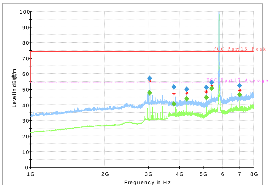
Fig. 63 Radiated Spurious Emission (802.11ac-HT20, Ch165, 1 GHz-8 GHz)
