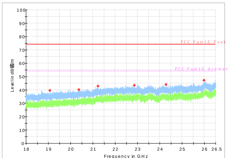
Fig. 65 Radiated Spurious Emission (802.11ac-HT20, Ch165, 18 GHz-26.5 GHz)
