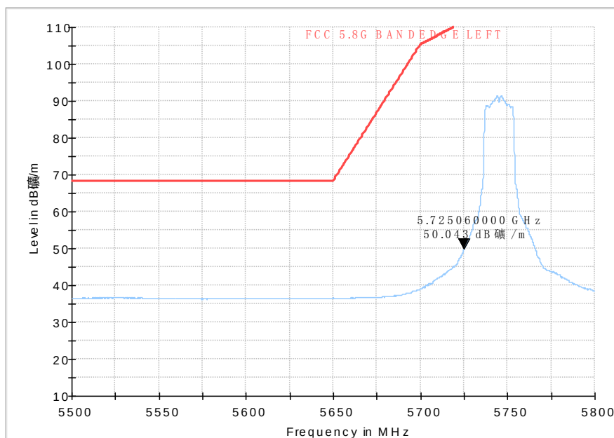
Average Fig. 78 Band Edges (802.11a, 5745MHz)
