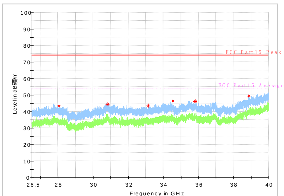
Fig. 76 Radiated emission: 802.11n, (802.11ac-HT80, Ch155, 26.5 GHz - 40 GHz)
