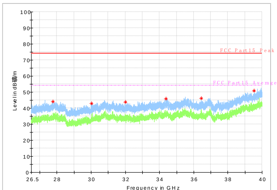
Fig. 71 Radiated emission: 802.11n, (802.11ac-HT40, Ch151, 26.5 GHz - 40 GHz)
