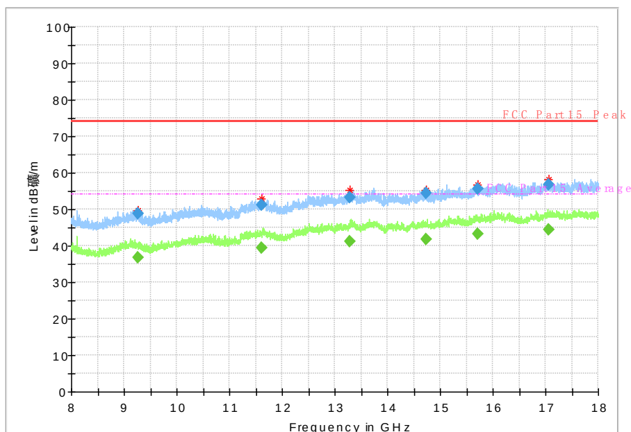
Fig. 59 Radiated Spurious Emission (802.11n-HT40, Ch151, 8 GHz-18 GHz)
