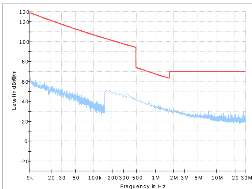
Fig. 77 Radiated Spurious Emission (9kHz-30MHz)
