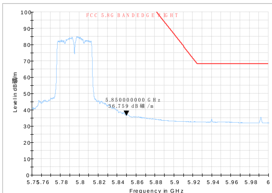
Fig. 83 Band Edges (802.11n-HT40, 5795MHz)
