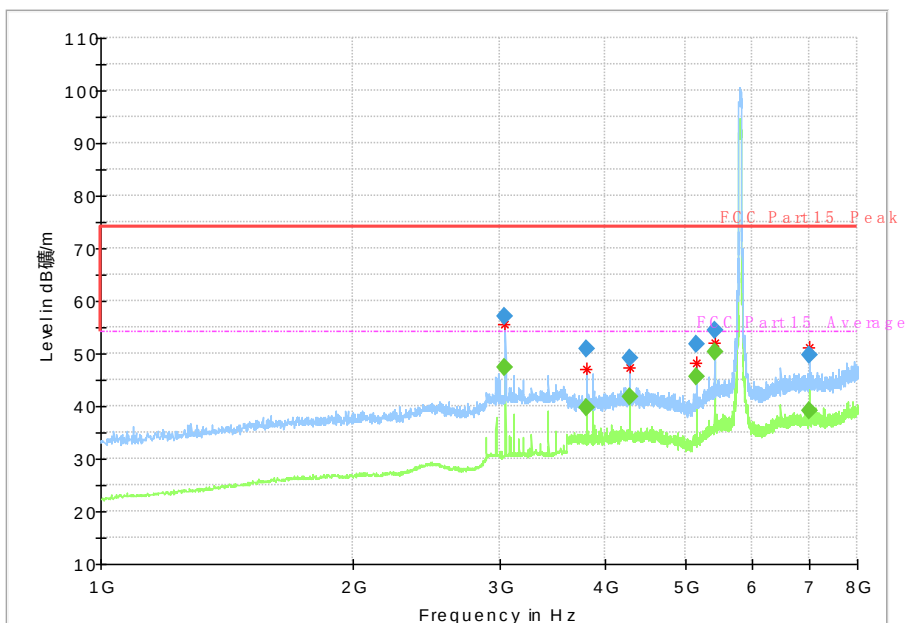
Fig. 58 Radiated Spurious Emission (802.11n-HT40, Ch151, 1 GHz-8 GHz)
