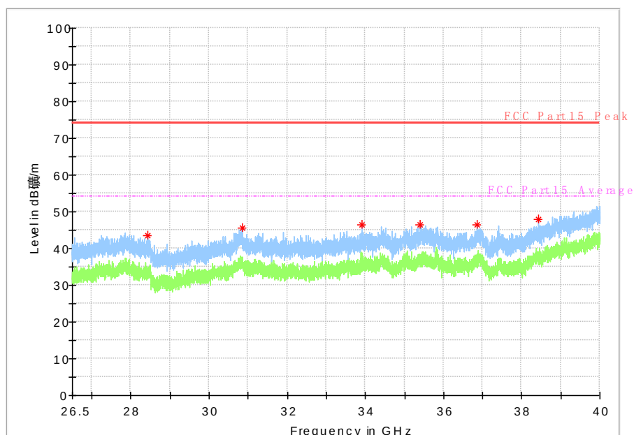
Fig. 66 Radiated emission: 802.11n, (802.11ac-HT20, Ch165, 26.5 GHz - 40 GHz)
