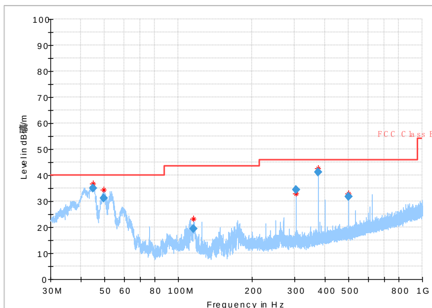
Fig. 57 Radiated Spurious Emission (802.11n-HT40, Ch151, 30 MHz-1 GHz)
