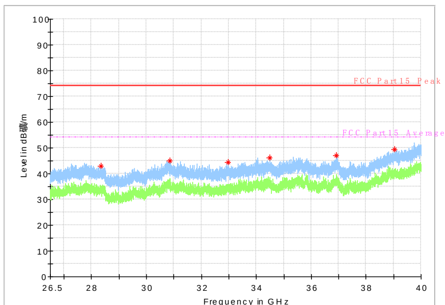
Fig. 61 Radiated emission: 802.11n, (802.11n-HT40, Ch151, 26.5 GHz - 40 GHz)
