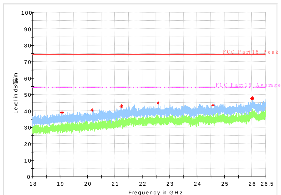
Fig. 70 Radiated Spurious Emission (802.11ac-HT40, Ch151, 18 GHz-26.5 GHz)
