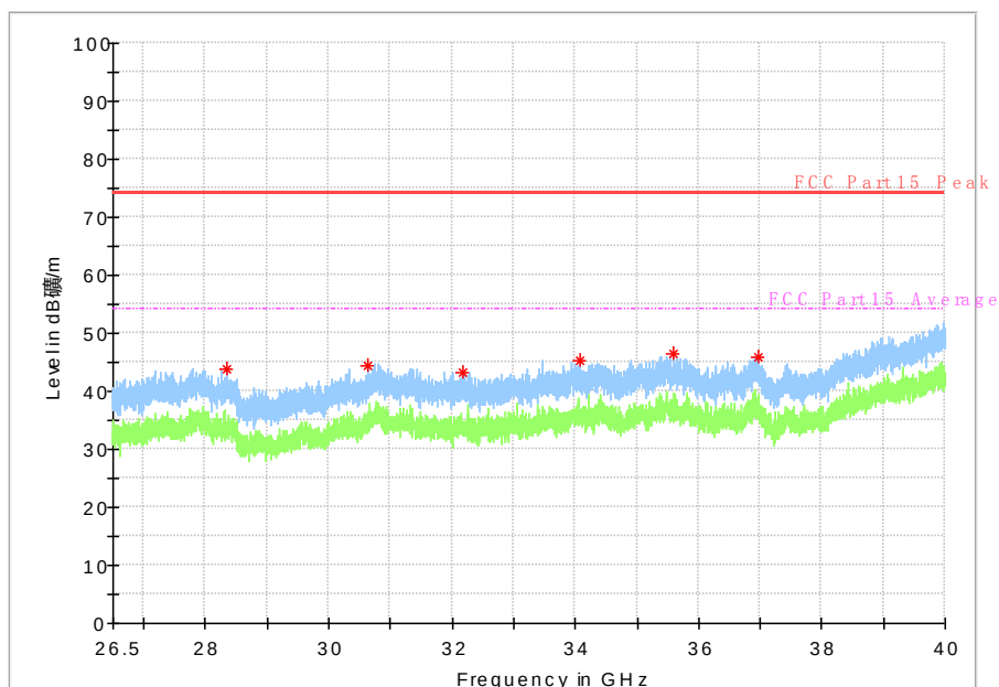
Fig. 51 Radiated emission: 802.11n, (802.11a, Ch149, 26.5 GHz - 40 GHz)
