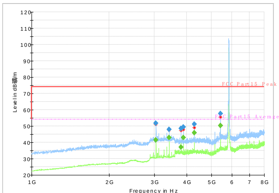
Fig. 53 Radiated Spurious Emission (802.11n-HT20, Ch165, 1 GHz-8 GHz)
