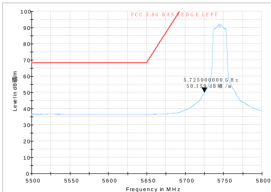
Fig. 80 Band Edges (802.11n-HT20, 5745MHz)
