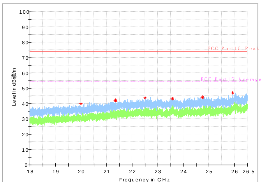
Fig. 60 Radiated Spurious Emission (802.11n-HT40, Ch151, 18 GHz-26.5 GHz)
