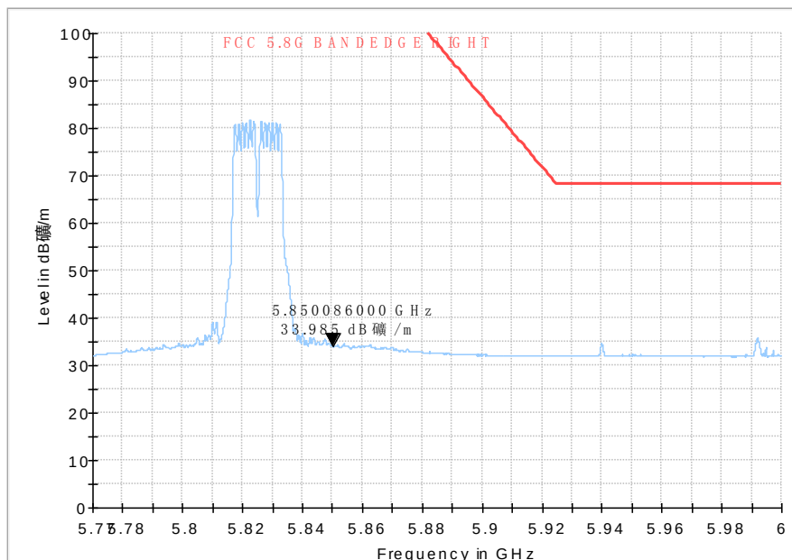
Fig. 85 Band Edges (802.11ac-HT20, 5825MHz)
