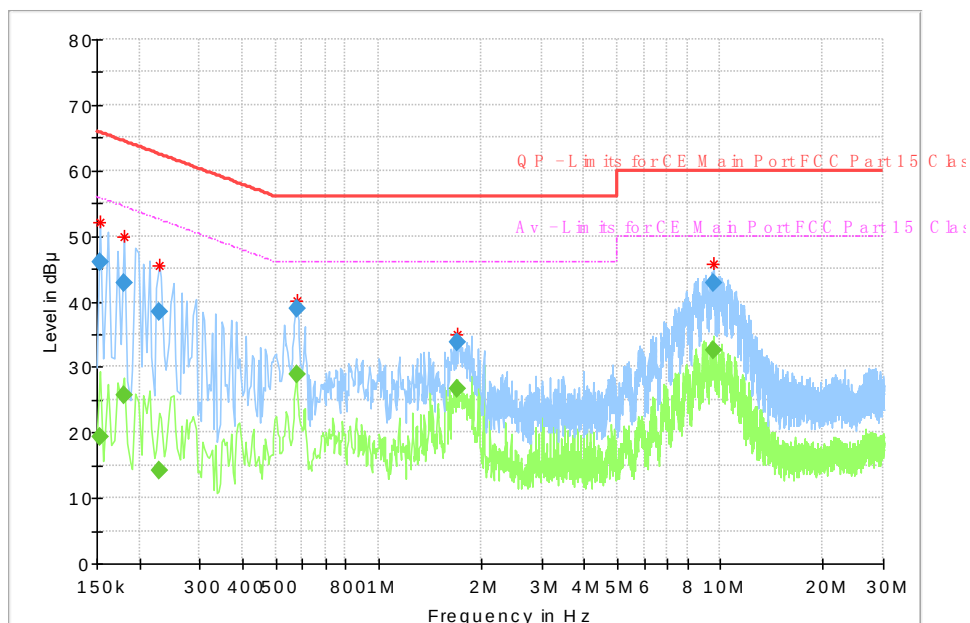
Fig. 89 AC Powerline Conducted Emission-802.11a
