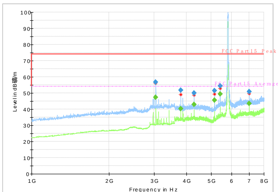
Fig. 68 Radiated Spurious Emission (802.11ac-HT40, Ch151, 1 GHz-8 GHz)
