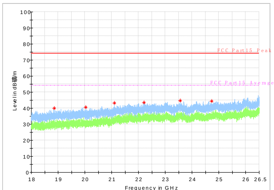
Fig. 75 Radiated Spurious Emission (802.11ac-HT80, Ch155, 18 GHz-26.5 GHz)
