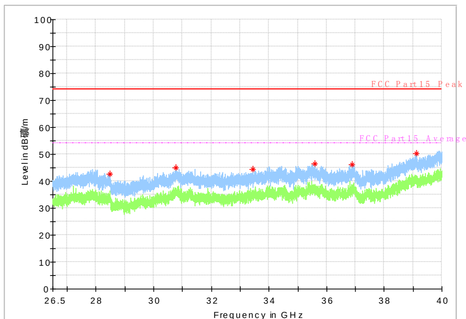
Fig. 56 Radiated emission: 802.11n, (802.11n-HT20, Ch165, 26.5 GHz - 40 GHz)
