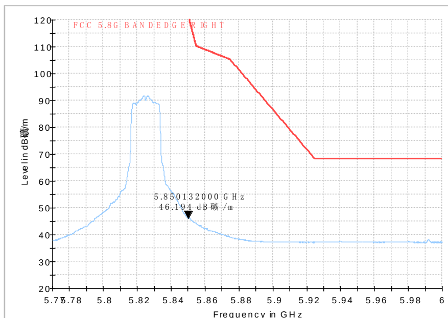
Average Fig. 79 Band Edges (802.11a, 5825MHz)
