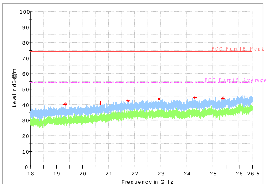
Fig. 55 Radiated Spurious Emission (802.11n-HT20, Ch165, 18 GHz-26.5 GHz)
