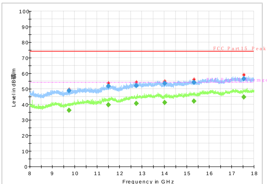
Fig. 54 Radiated Spurious Emission (802.11n-HT20, Ch165, 8 GHz-18 GHz)
