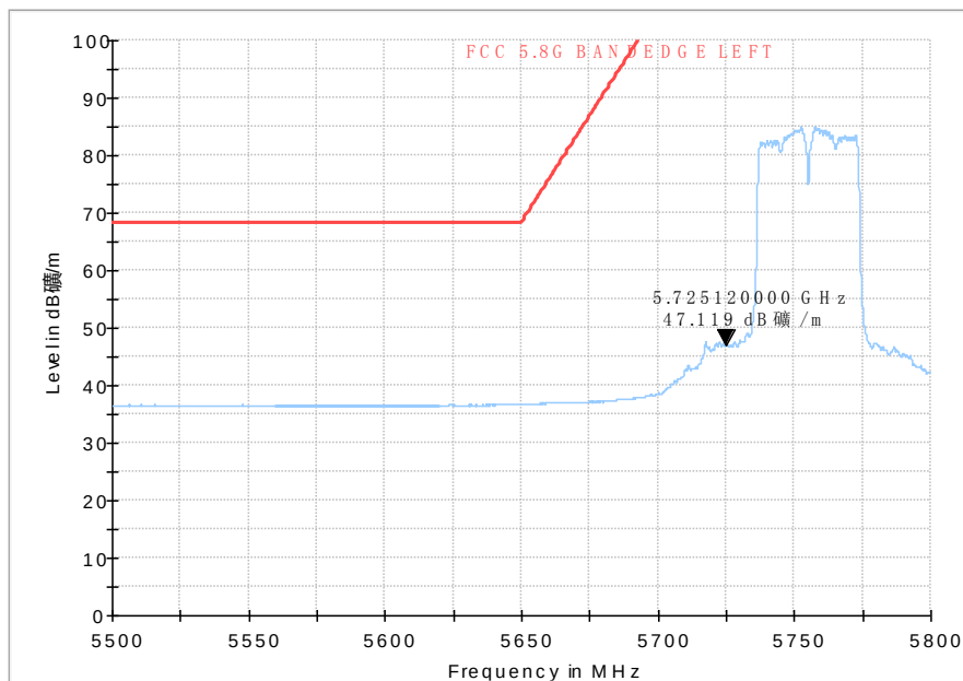
Fig. 86 Band Edges (802.11ac-HT40, 5755MHz)
