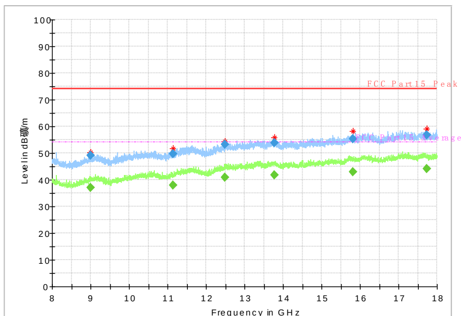
Fig. 69 Radiated Spurious Emission (802.11ac-HT40, Ch151, 8 GHz-18 GHz)
