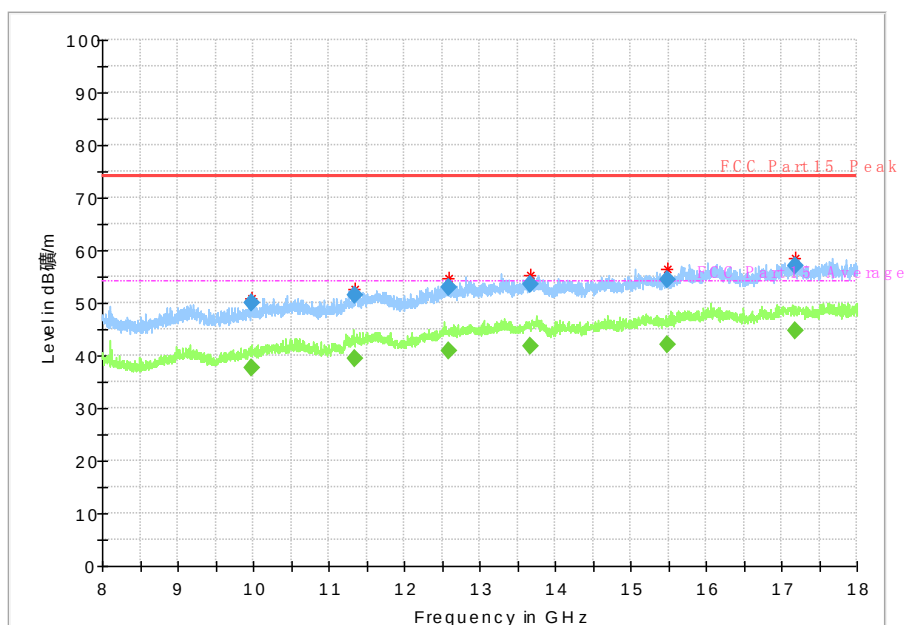
Fig. 74 Radiated Spurious Emission (802.11ac-HT80, Ch155, 8 GHz-18 GHz)
