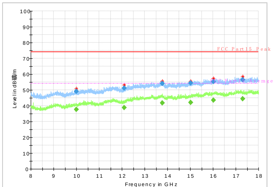
Fig. 49 Radiated Spurious Emission (802.11a, Ch149, 8 GHz-18 GHz)
