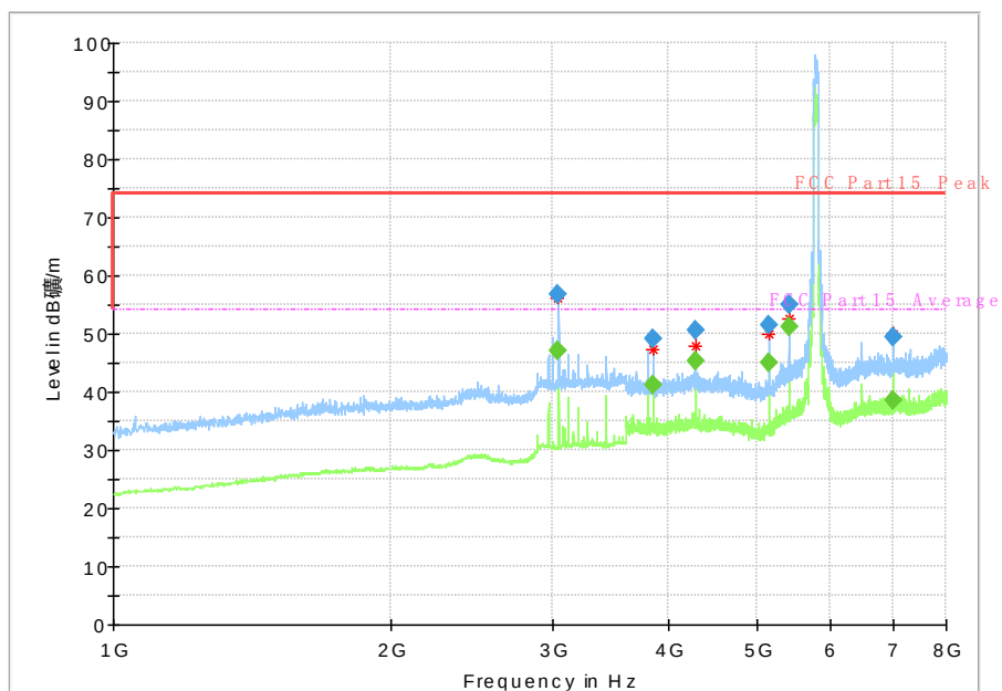
Fig. 73 Radiated Spurious Emission (802.11ac-HT80, Ch155, 1 GHz-8 GHz)
