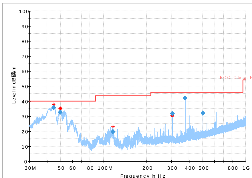
Fig. 67 Radiated Spurious Emission (802.11ac-HT40, Ch151, 30 MHz-1 GHz)
