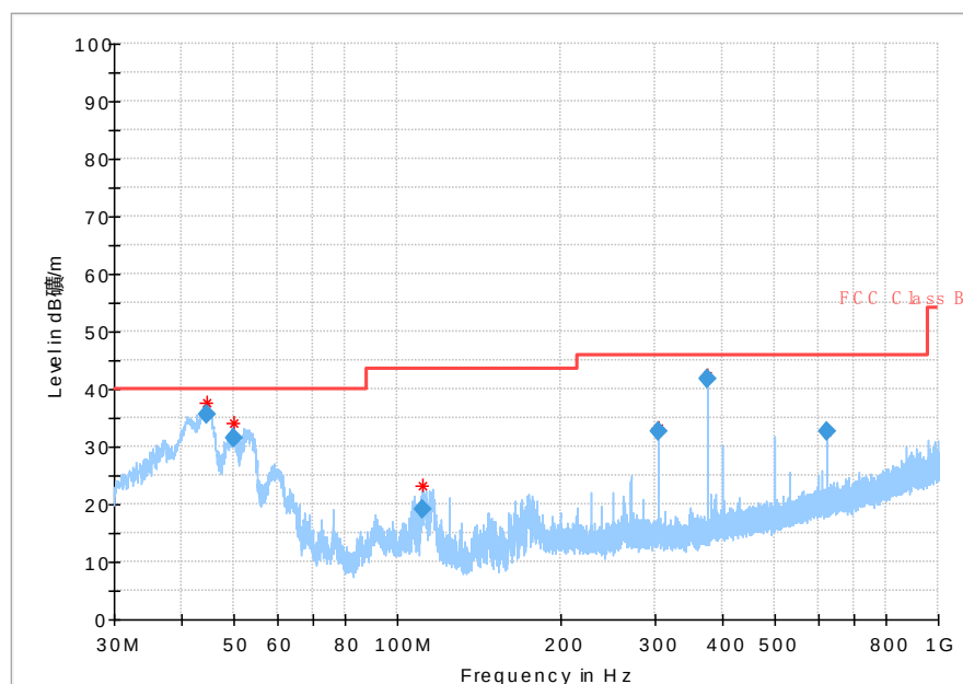
Fig. 62 Radiated Spurious Emission (802.11ac-HT20, Ch165, 30 MHz-1 GHz)
