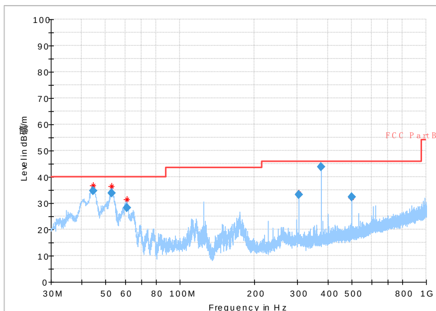
Fig. 47 Radiated Spurious Emission (802.11a, Ch149, 30 MHz-1 GHz)
