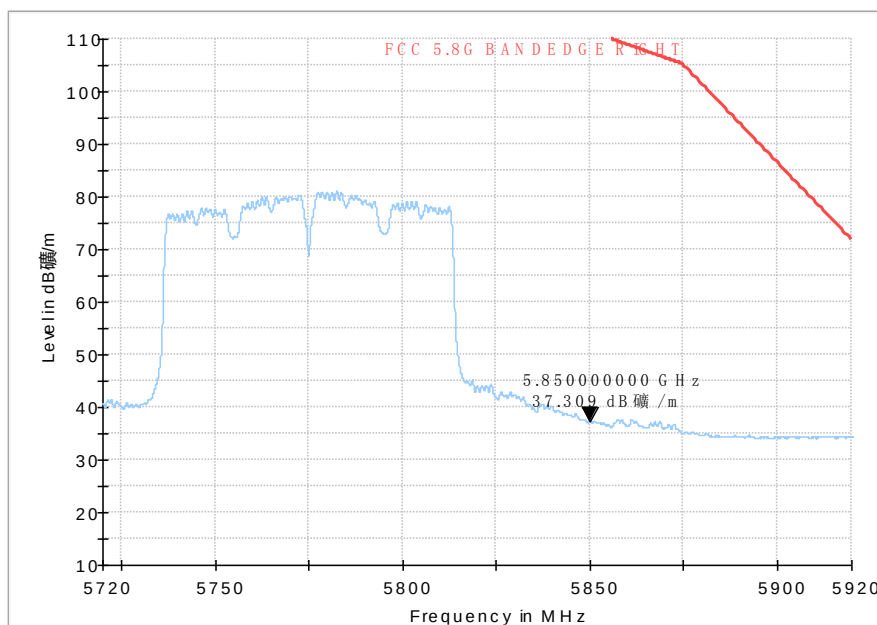
Fig. 88 Band Edges (802.11ac-HT80, 5775MHz)
