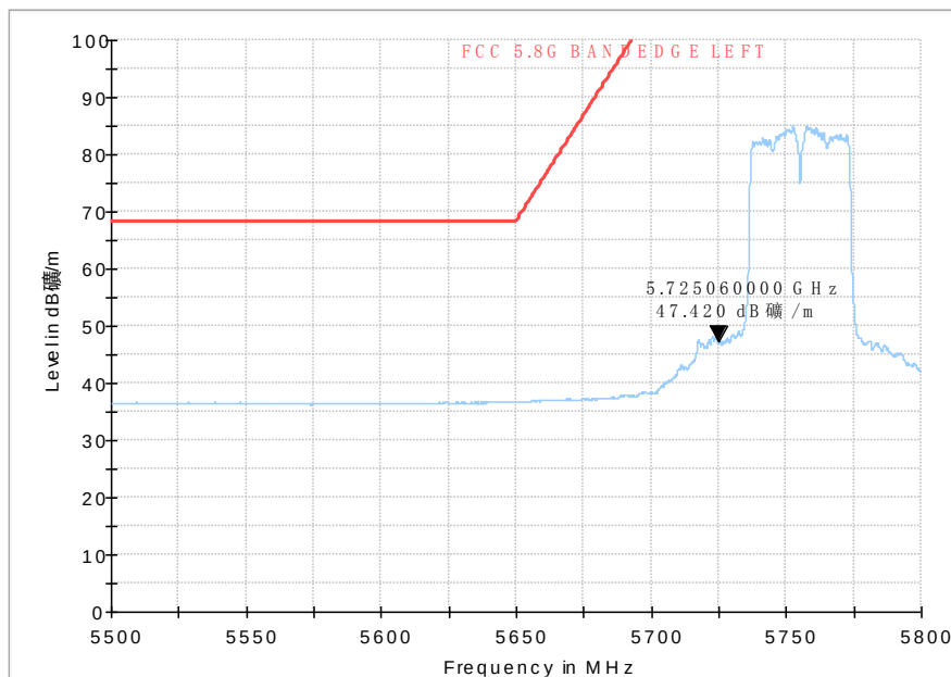
Fig. 82 Band Edges (802.11n-HT40, 5755MHz)
