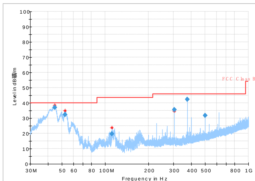
Fig. 72 Radiated Spurious Emission (802.11ac-HT80, Ch155, 30 MHz-1 GHz)
