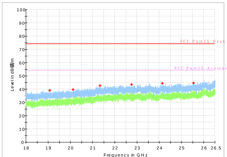
Fig. 50 Radiated Spurious Emission (802.11a, Ch149, 18 GHz-26.5 GHz)
