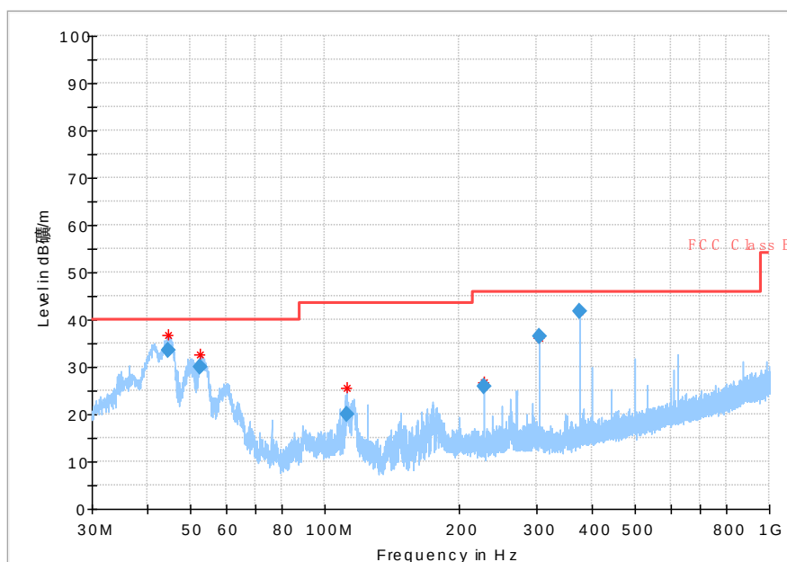
Fig. 52 Radiated Spurious Emission (802.11n-HT20, Ch165, 30 MHz-1 GHz)
