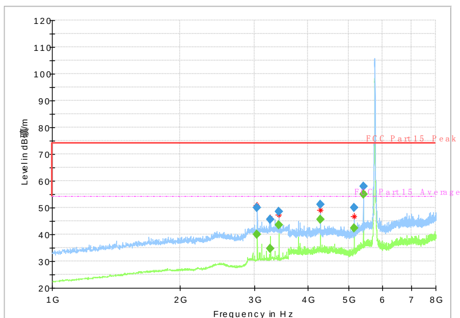
Fig. 48 Radiated Spurious Emission (802.11a, Ch149, 1 GHz-8 GHz)
