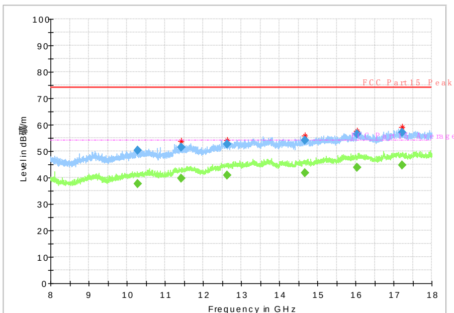
Fig. 64 Radiated Spurious Emission (802.11ac-HT20, Ch165, 8 GHz-18 GHz)
