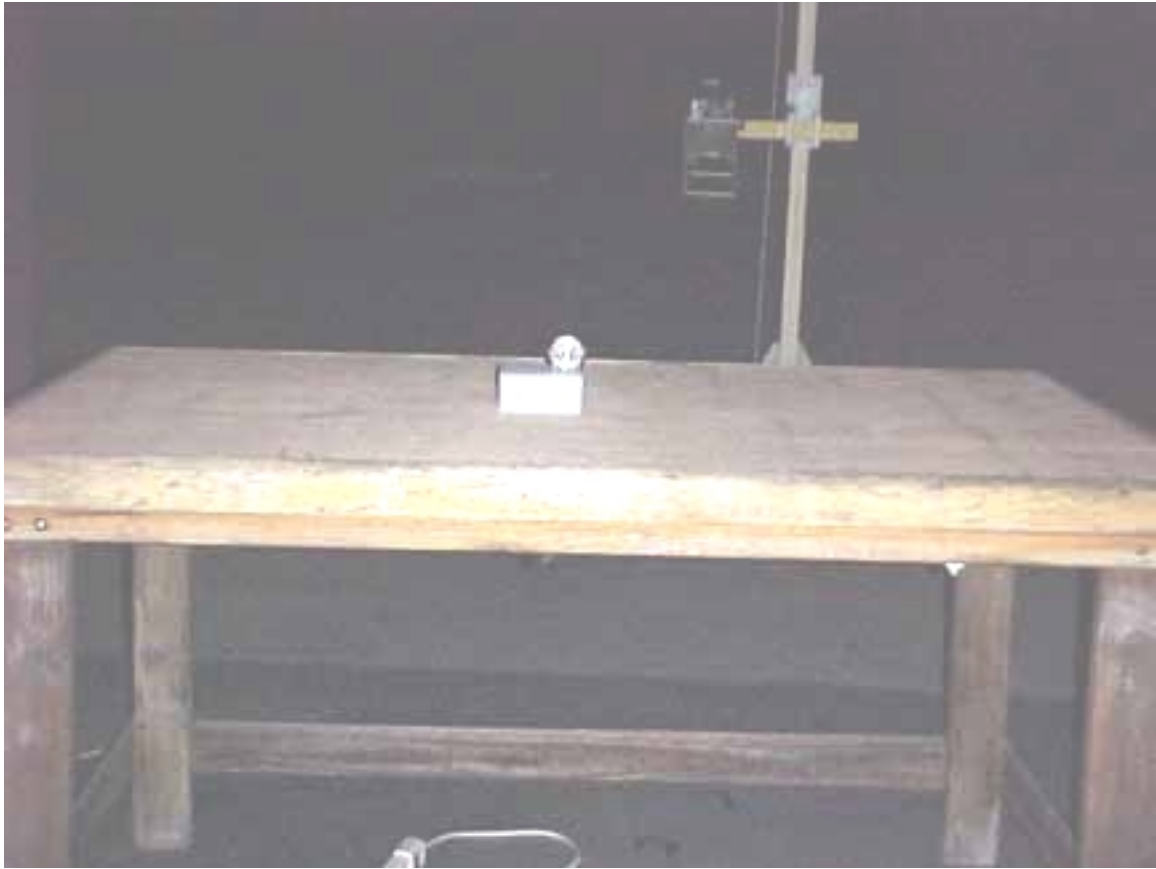
Front View of the Radiated Emissions Test Setup
