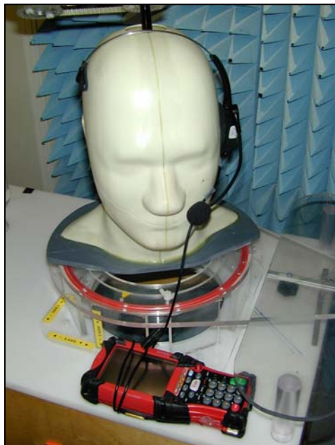
Figure 27. Positional photograph of the MC9060 with Headset connected and placed against the SAM Phantom in the left-hand Cheek Position.
