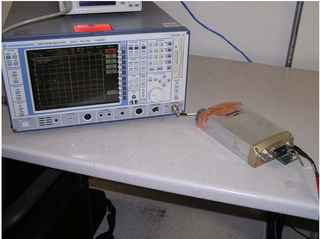
ANTENNA PORT MEASUREMENTS
