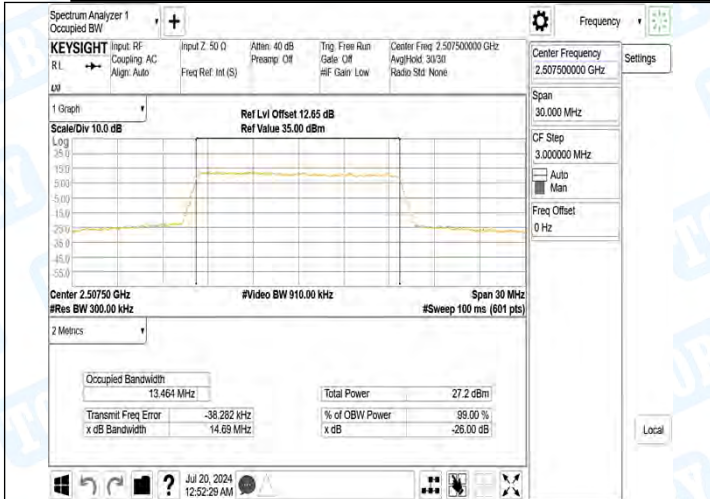
Band7-15MHz-QPSK-21375-75RB#0-PASS
