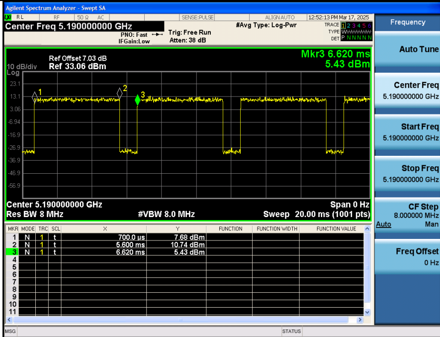
Duty Cycle NVNT ANT1_802_11ac(VHT40)_5190
