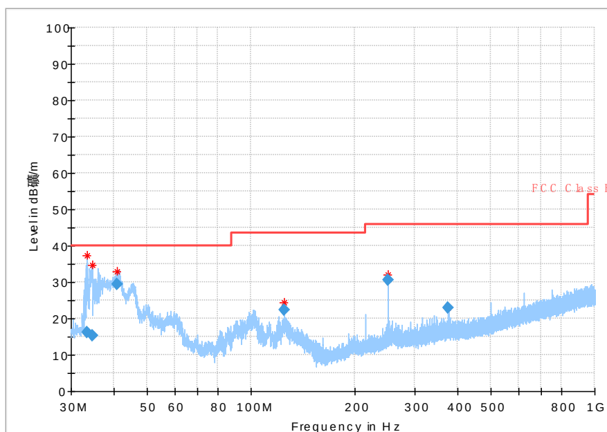
Fig. 42 Radiated Spurious Emission (802.11n-HT20, Ch165, 30 MHz-1 GHz)
