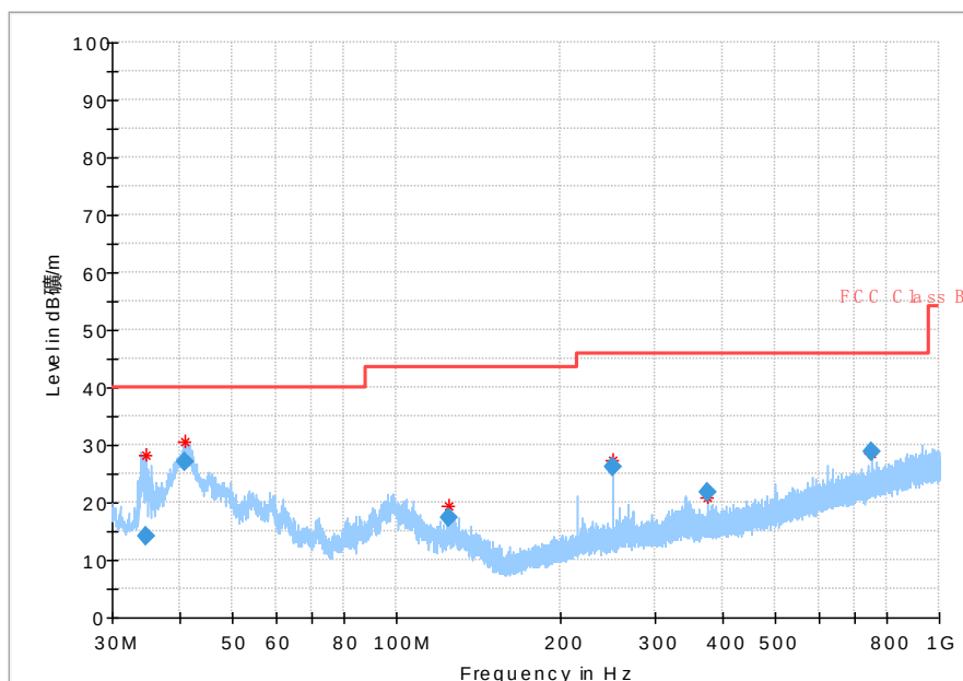
Fig. 47 Radiated Spurious Emission (802.11ac-HT20, Ch165, 30 MHz-1 GHz)
