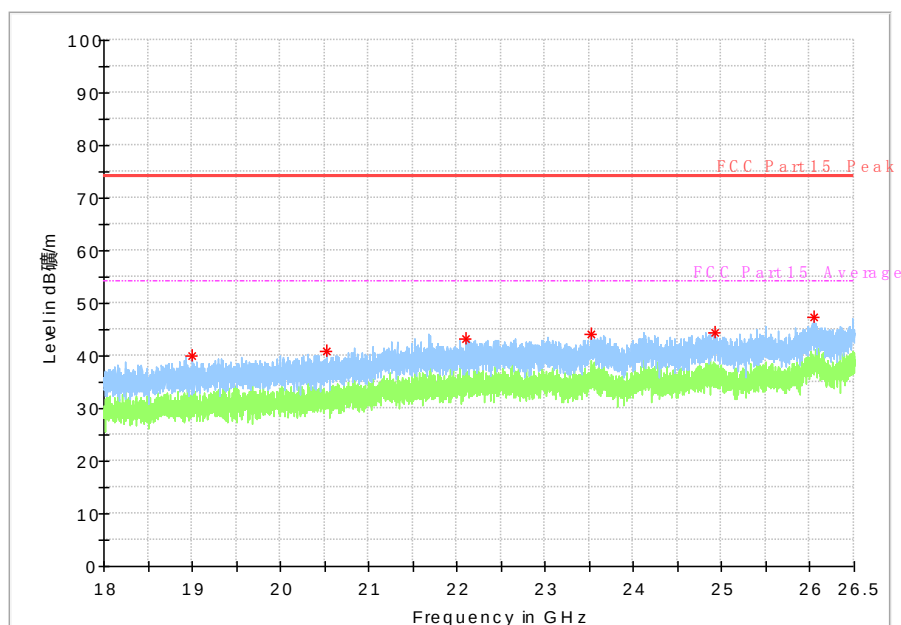
Fig. 40 Radiated Spurious Emission (802.11a, Ch149, 18 GHz-26.5 GHz)
