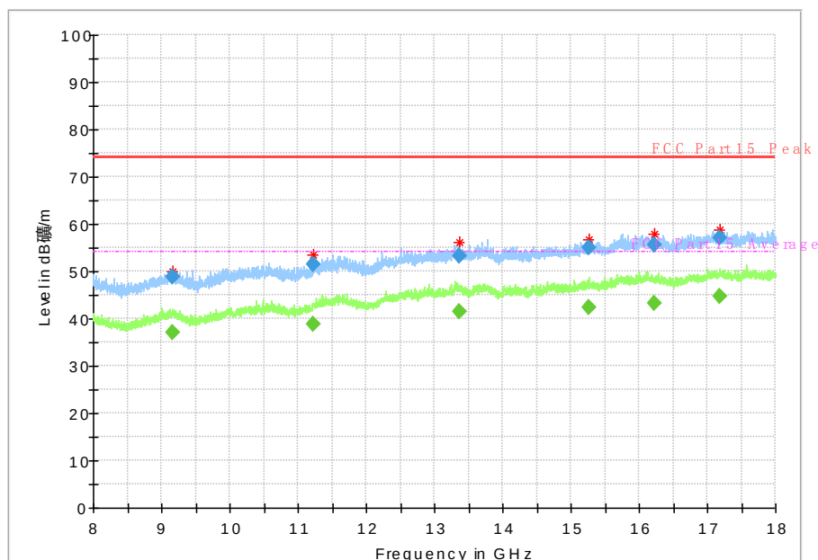
Fig. 39 Radiated Spurious Emission (802.11a, Ch149, 8 GHz-18 GHz)
