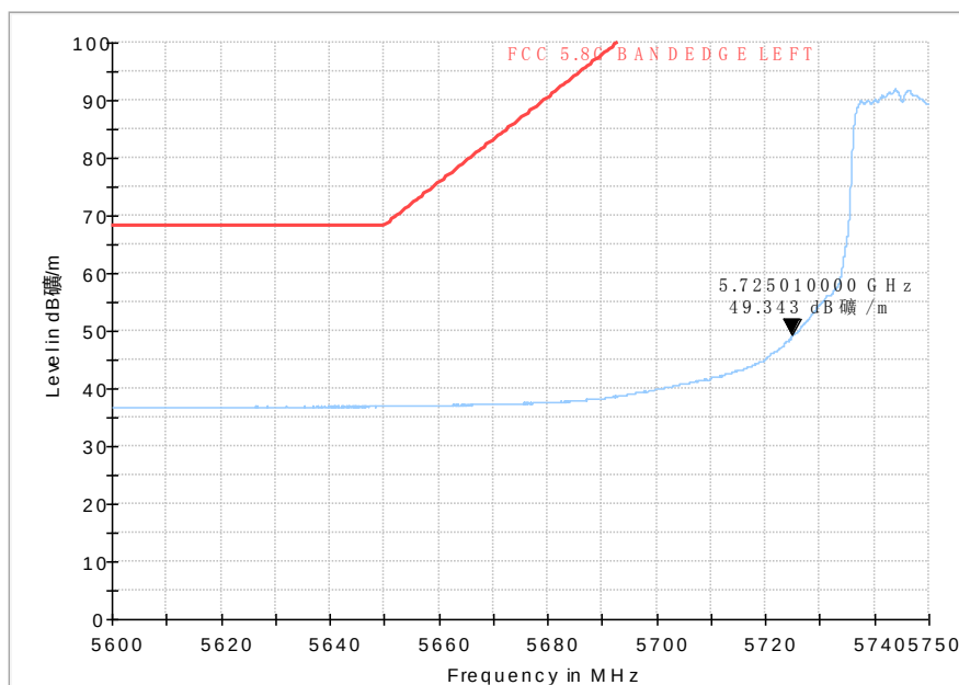
Fig. 56 Band Edges (802.11ac-HT20, 5745MHz)
