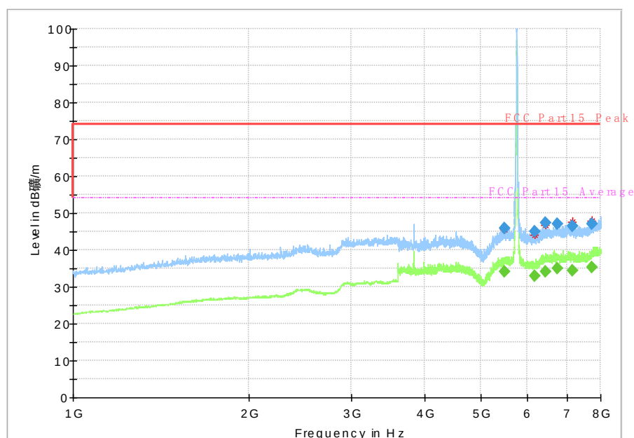
Fig. 38 Radiated Spurious Emission (802.11a, Ch149, 1 GHz-8 GHz)
