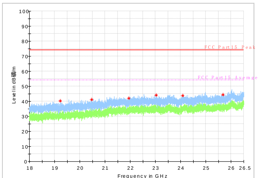
Fig. 45 Radiated Spurious Emission (802.11n-HT20, Ch165, 18 GHz-26.5 GHz)
