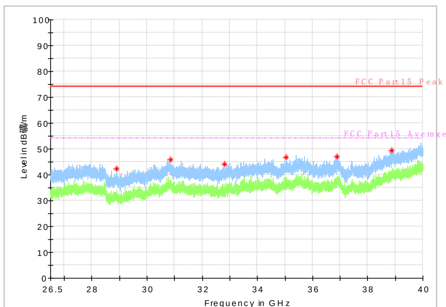
Fig. 46 Radiated emission: 802.11n, (802.11n-HT20, Ch165, 26.5 GHz - 40 GHz)
