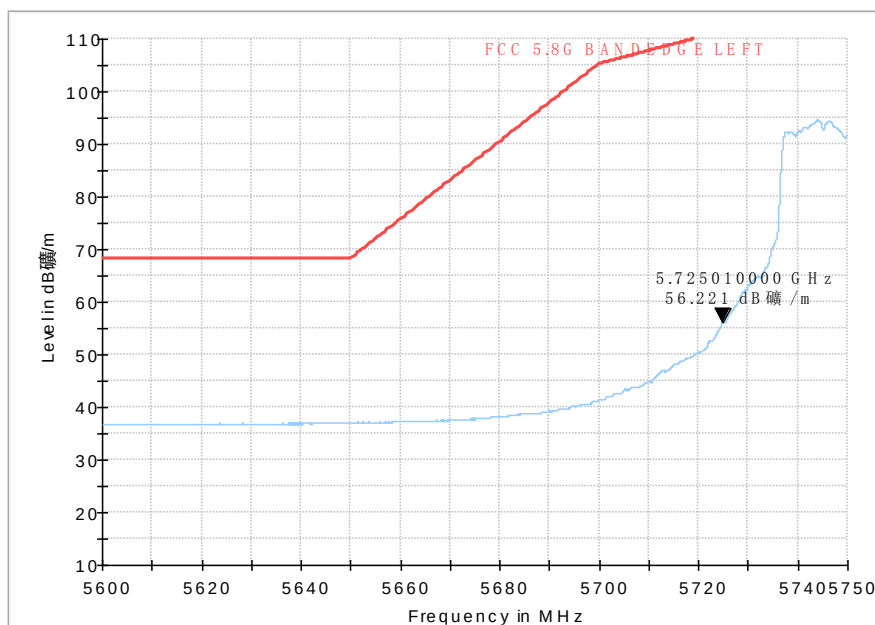
Average Fig. 52 Band Edges (802.11a, 5745MHz)
