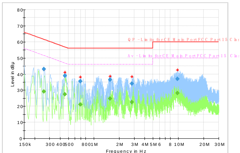
Fig. 58 AC Powerline Conducted Emission-802.11a
