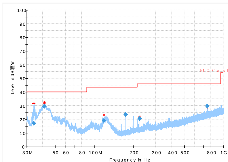
Fig. 37 Radiated Spurious Emission (802.11a, Ch149, 30 MHz-1 GHz)
