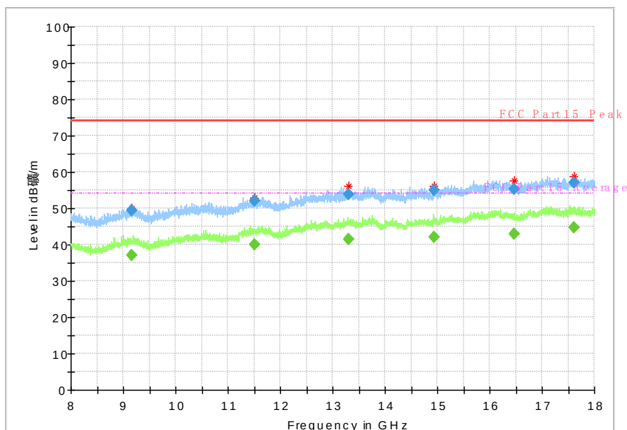
Fig. 49 Radiated Spurious Emission (802.11ac-HT20, Ch165, 8 GHz-18 GHz)
