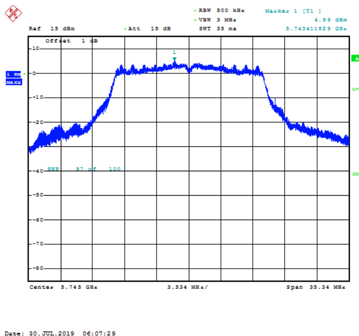
Fig. 1 Power Spectral Density (802.11a, Ch 149)
