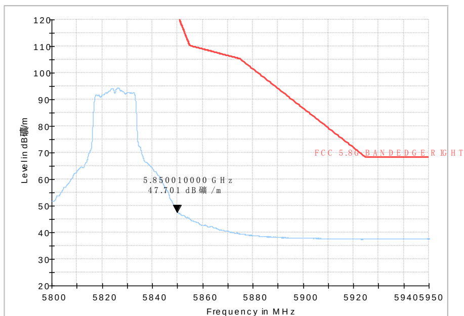
Fig. 53 Band Edges (802.11a, 5825MHz)
