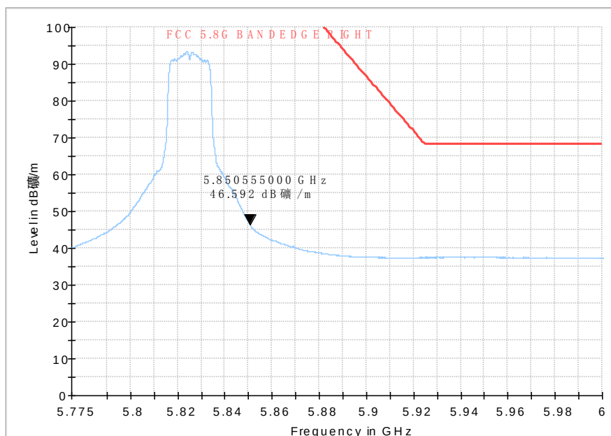
Fig. 55 Band Edges (802.11n-HT20, 5825MHz)
