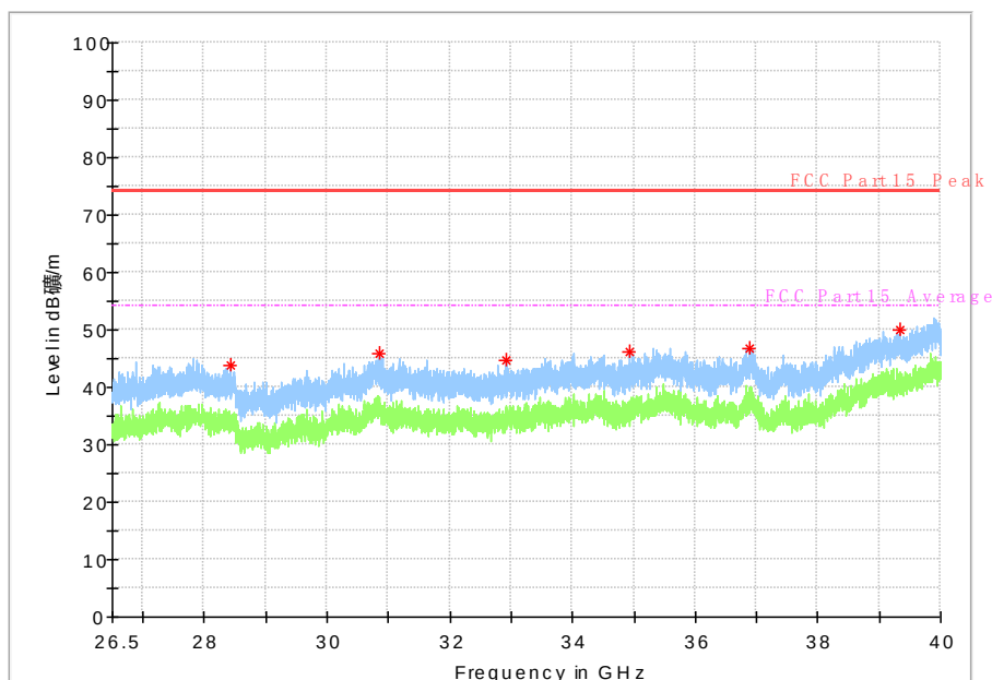
Fig. 41 Radiated emission: 802.11n, (802.11a, Ch149, 26.5 GHz - 40 GHz)
