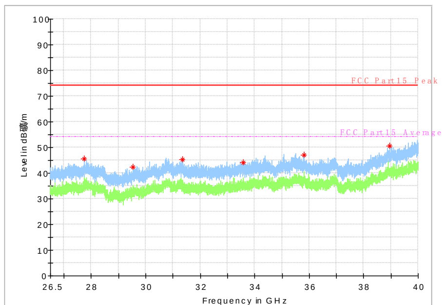
Fig. 51 Radiated emission: 802.11n, (802.11ac-HT20, Ch165, 26.5 GHz - 40 GHz)
