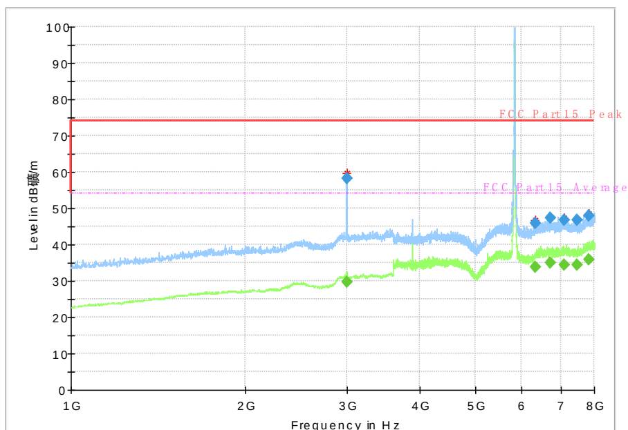
Fig. 43 Radiated Spurious Emission (802.11n-HT20, Ch165, 1 GHz-8 GHz)
