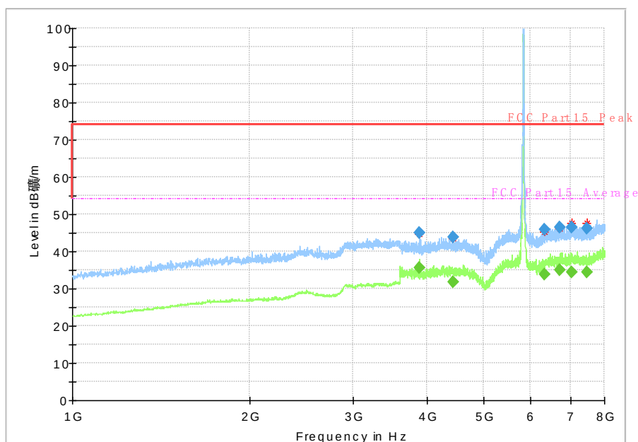
Fig. 48 Radiated Spurious Emission (802.11ac-HT20, Ch165, 1 GHz-8 GHz)
