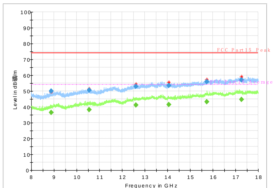
Fig. 44 Radiated Spurious Emission (802.11n-HT20, Ch165, 8 GHz-18 GHz)
