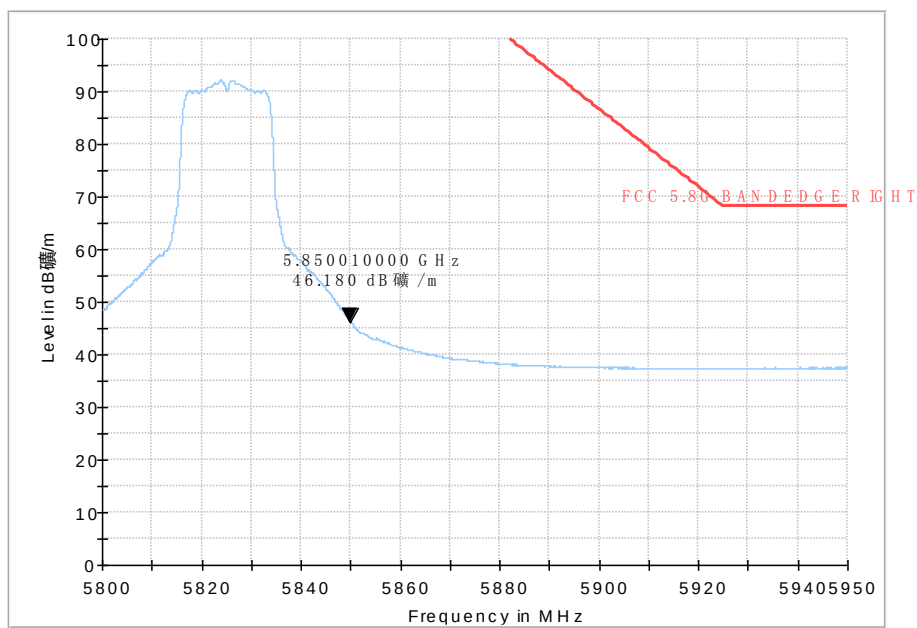
Fig. 57 Band Edges (802.11ac-HT20, 5825MHz)
