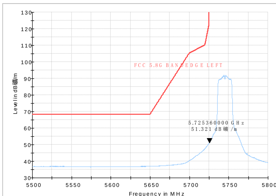
Fig. 54 Band Edges (802.11n-HT20, 5745MHz)
