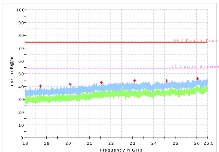
Fig. 50 Radiated Spurious Emission (802.11ac-HT20, Ch165, 18 GHz-26.5 GHz)
