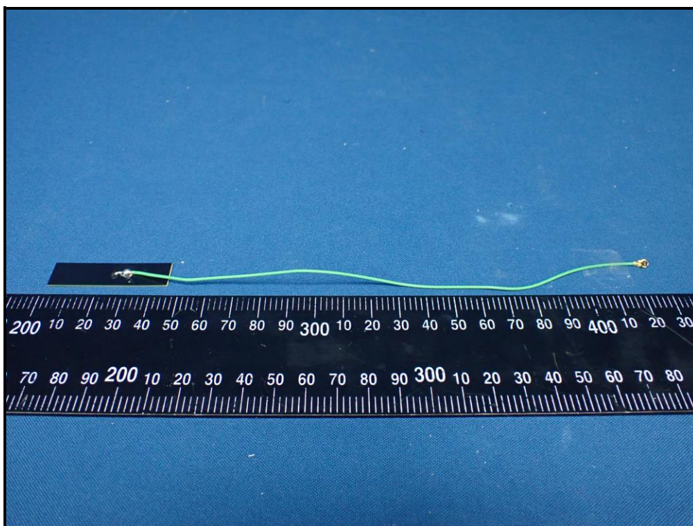
WLAN_2G-1 Antenna
