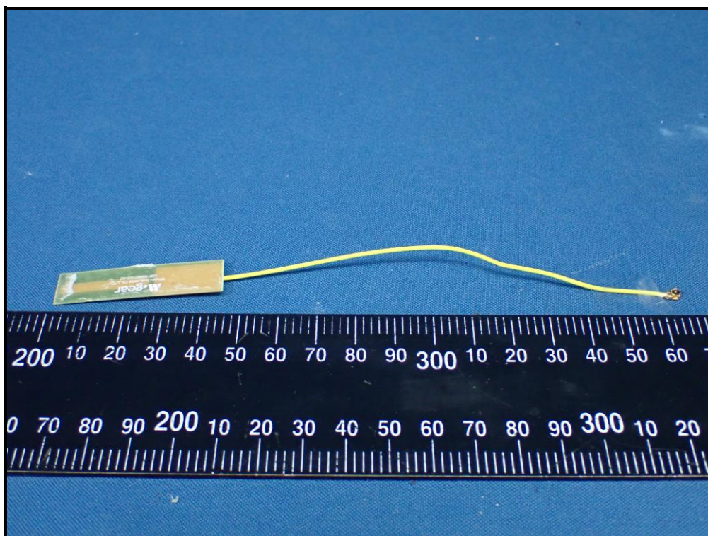
WLAN_2G-0 Antenna
