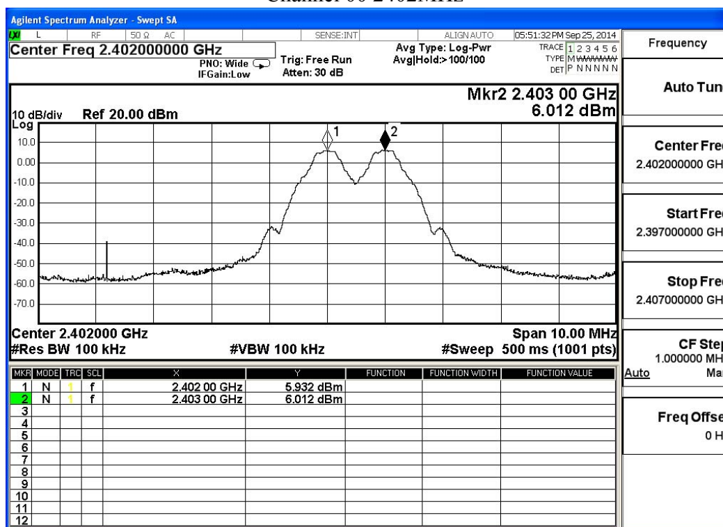
Channel 00 2402MHz
