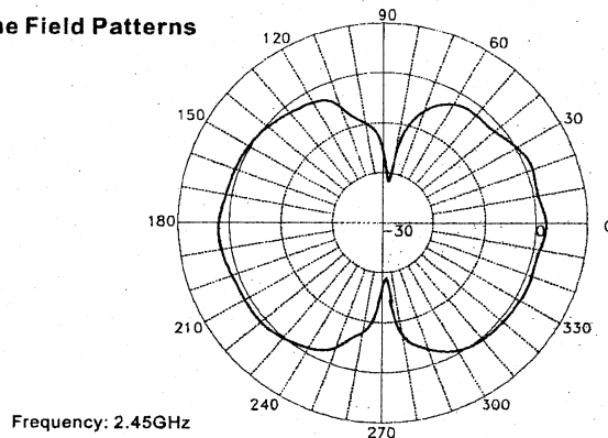
H-Plane Field Patterns
