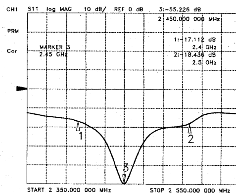
Return Loss
