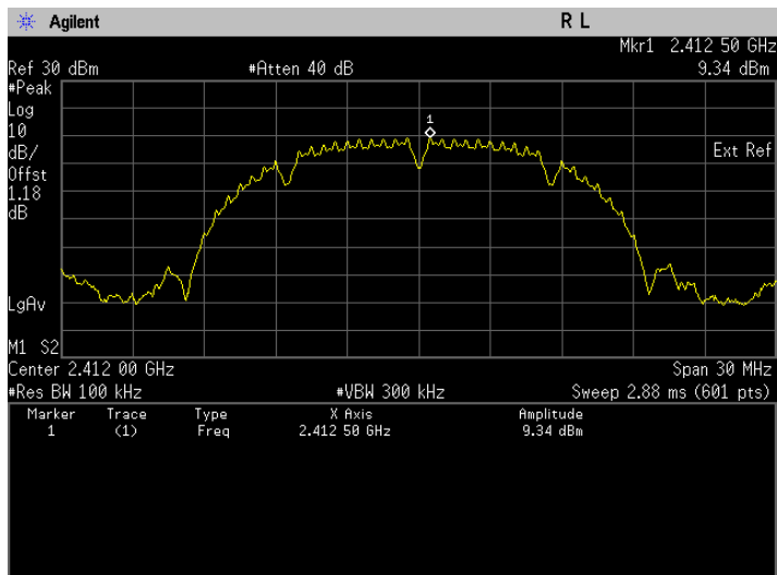
Conducted Emissions. 802.11b, Frequency 2412 MHz Reference Level
