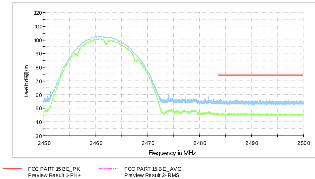
Fig.A.5.2.2 Radiated band Edges (802.11b, Ch 11)
