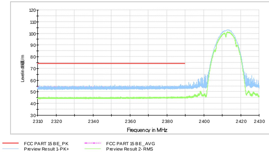
Fig.A.5.2.1 Radiated band Edges (802.11b, Ch 1)
