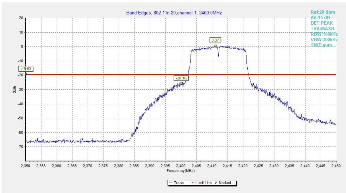
Fig.A.5.1.5 Band Edges (802.11n-HT20, Ch 1)
