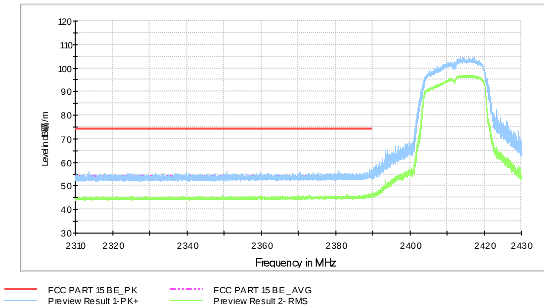
Fig.A.5.2.3 Radiated band Edges (802.11g, Ch 1)
