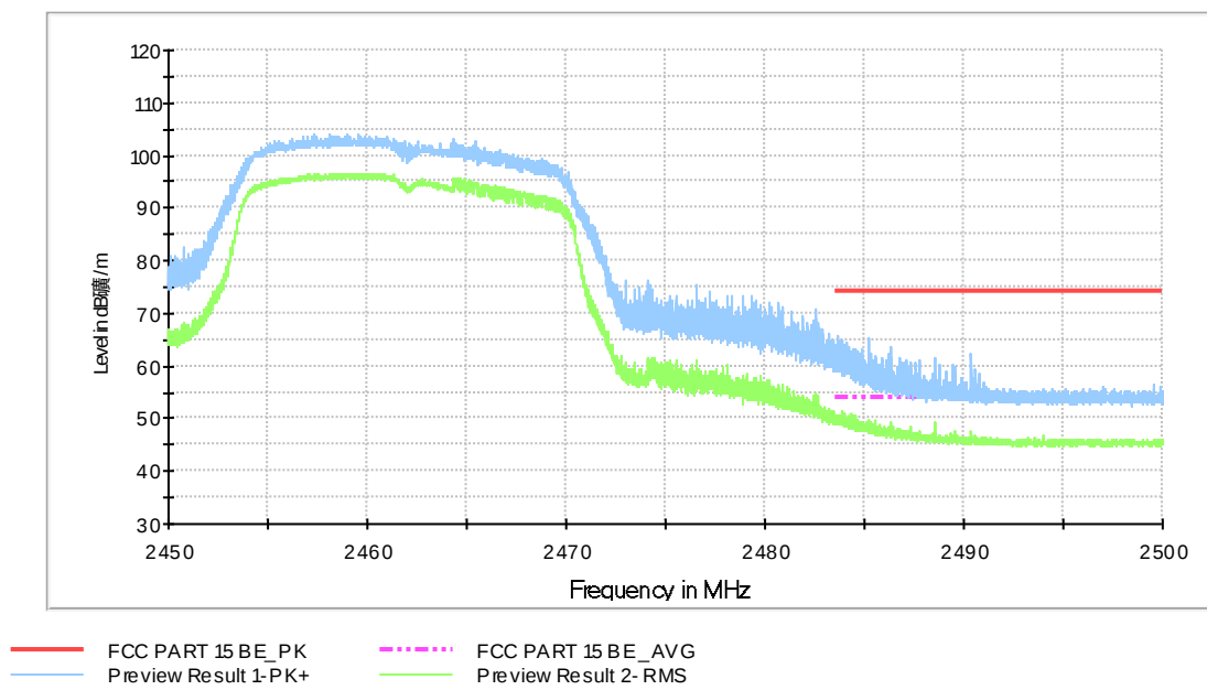
Fig.A.5.2.4 Radiated band Edges (802.11g, Ch 11)
