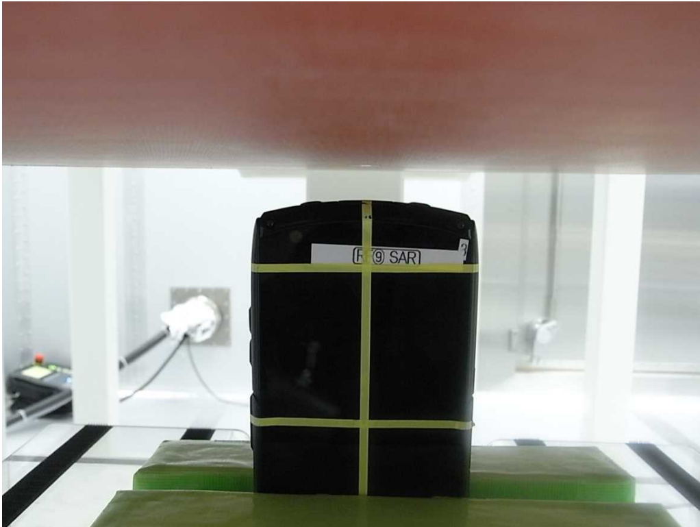
Test setup photo (Top)
