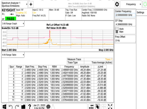
Band7_20MHz_DFT_s_OFDM_SCS15kHz_BPSK_RB1_0_CH507000
