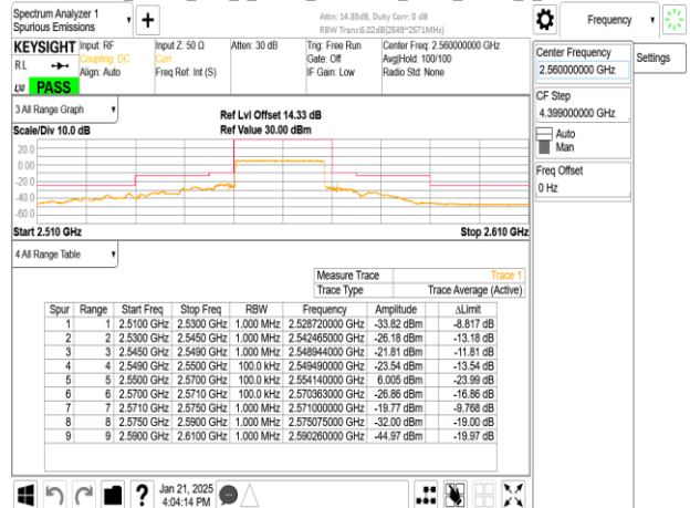
Band7_20MHz_DFT_s_OFDM_SCS15kHz_BPSK_RB1_0_CH512000
