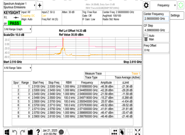
Band7_20MHz_DFT_s_OFDM_SCS15kHz_BPSK_RB1_0_CH512000
