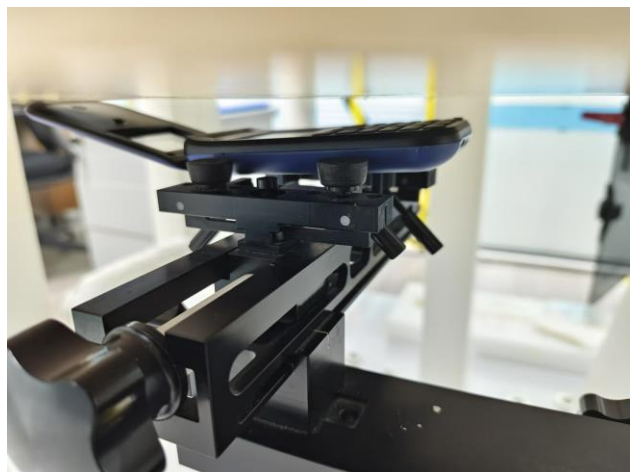
Front side-Open mode (10mm)
