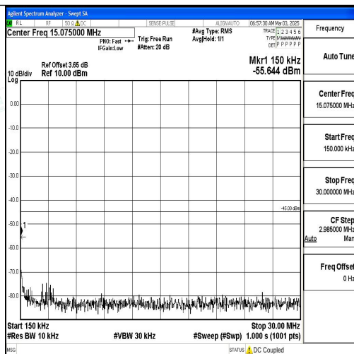
Band7_20MHz_QPSK_21350_1RB#0_0.15~30_0.15~30
