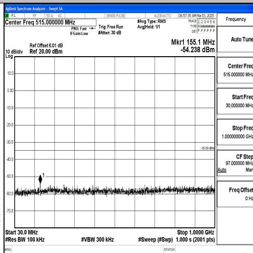
Band7_20MHz_QPSK_21350_1RB#0_30~1000_30~1000
