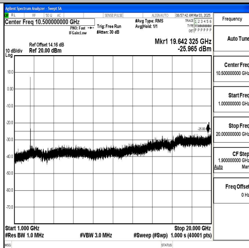
Band7_20MHz_QPSK_21350_1RB#0_1000~20000_1000~20000
