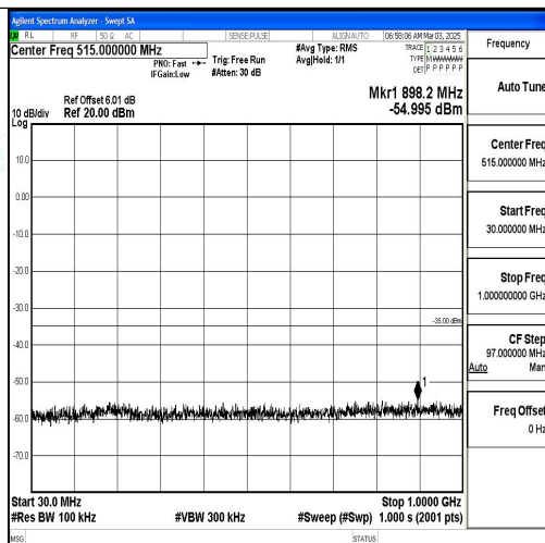
Band7_20MHz_16QAM_21350_1RB#0_30~1000_30~1000
