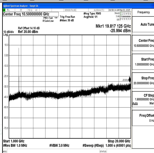
Band7_20MHz_16QAM_21350_1RB#0_1000~20000_1000~20000
