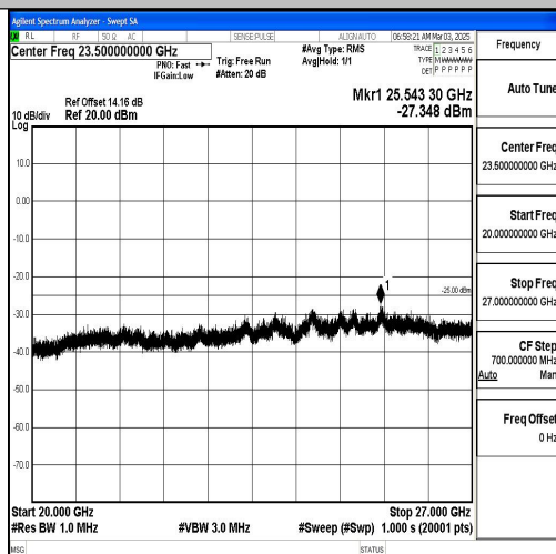
Band7_20MHz_16QAM_21350_1RB#0_20000~27000_20000~27000
