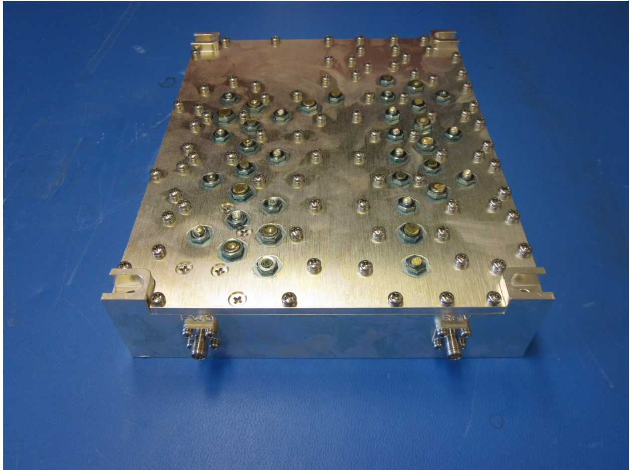
Duplexer #1
