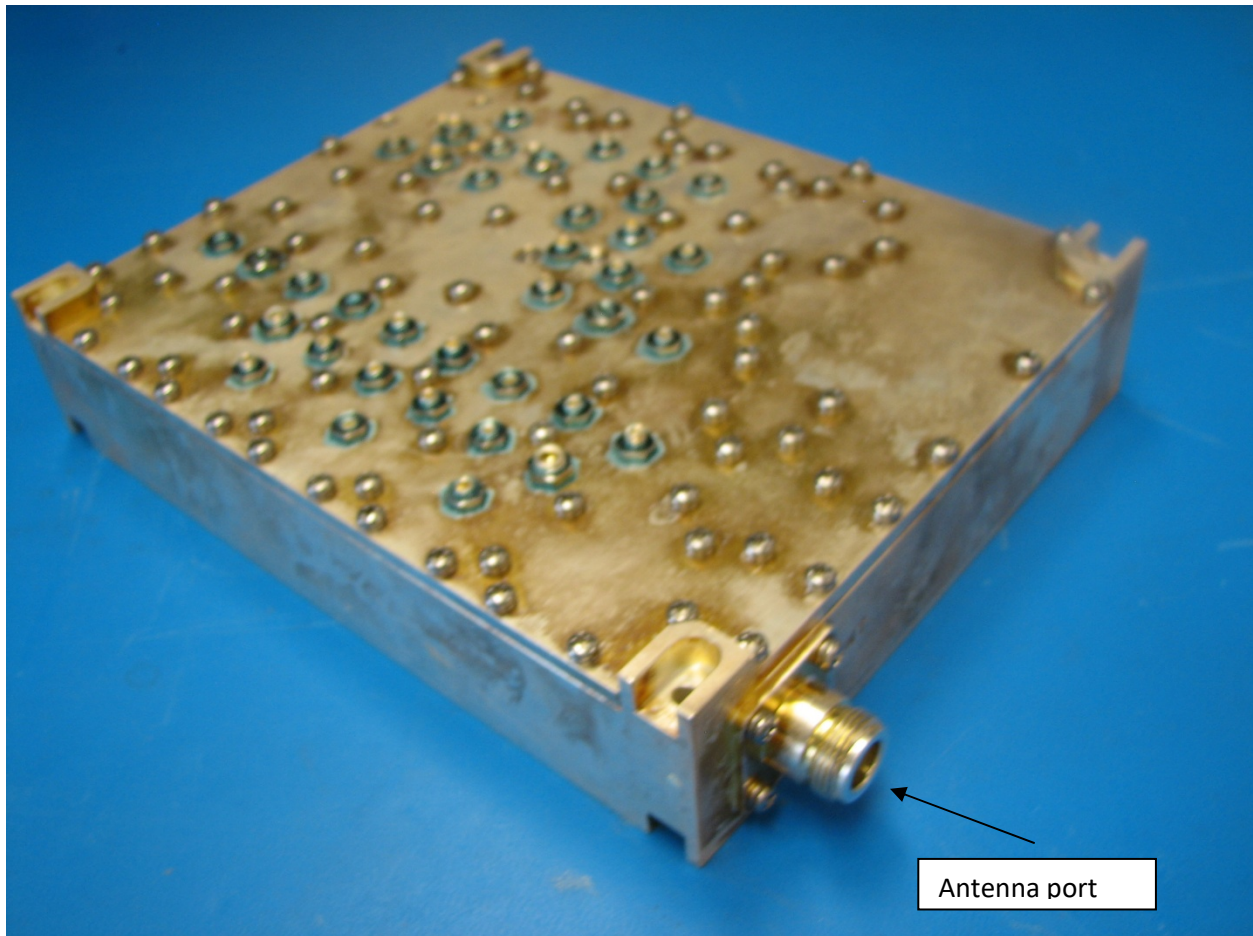
Duplexer #2
