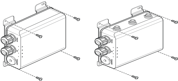
Figure 4 AP7662i and AP7662 Wall Mount "H" Bracket
