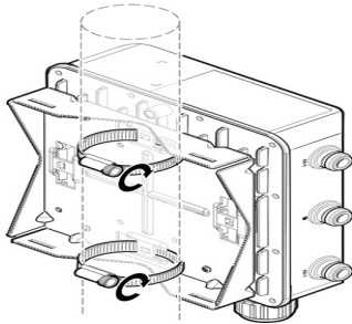
Figure 6 AP with Mounting Bracket—Vertical Pole
