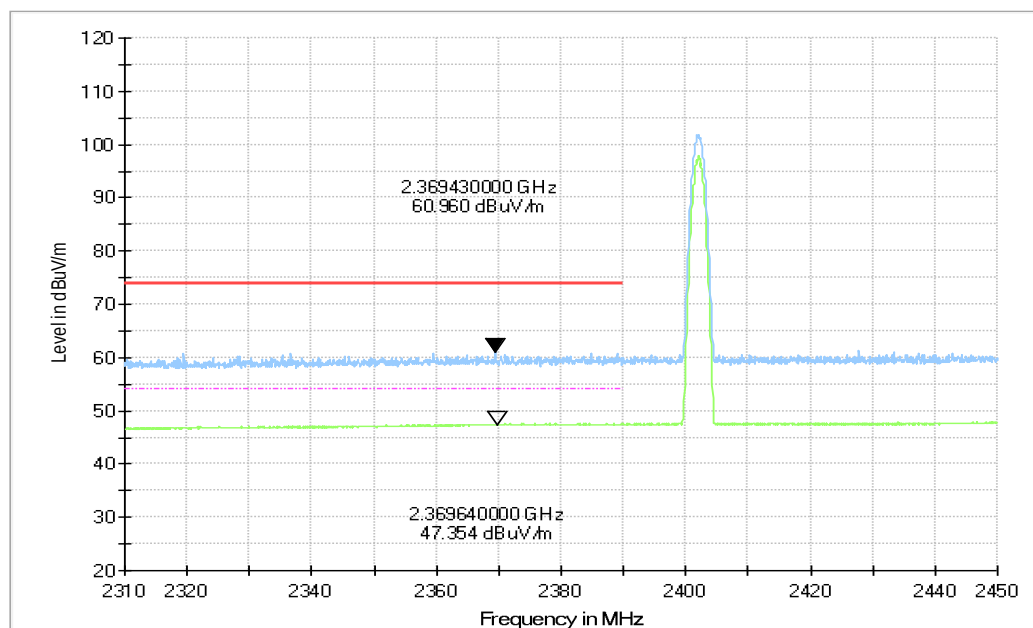
Fig.62. Frequency Band Edges: 8DPSK, Channel 0, 2.31 GHz - 2.45GHz
