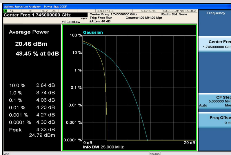
Band66-3MHz-16QAM-132322-1RB#0
