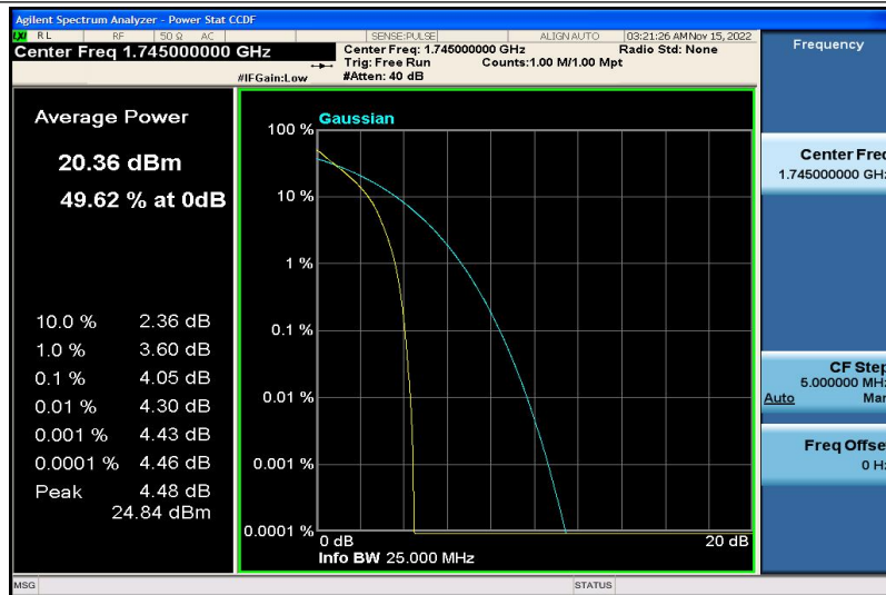
Band66-3MHz-QPSK-132322-15RB#0
