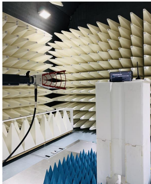
Figure F2. Radiated Setup – High Range
