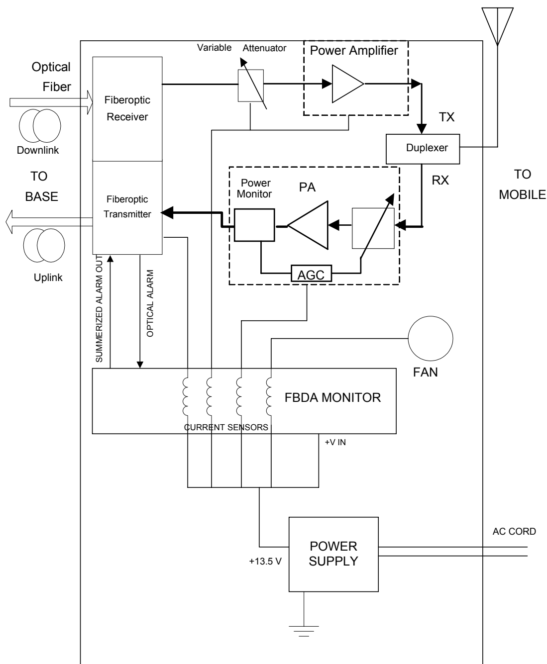
FBDA-PCS-AC-10W ELELCTRICAL SCHEMATICS
