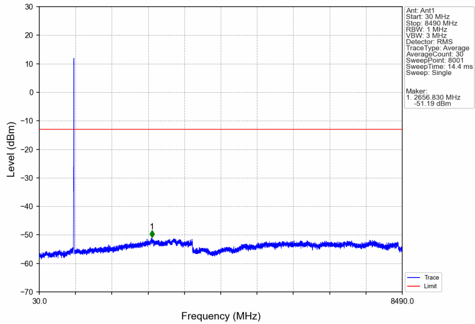
Band5 HSDPA HCH 846.6MHz Subtest 1 NTV
