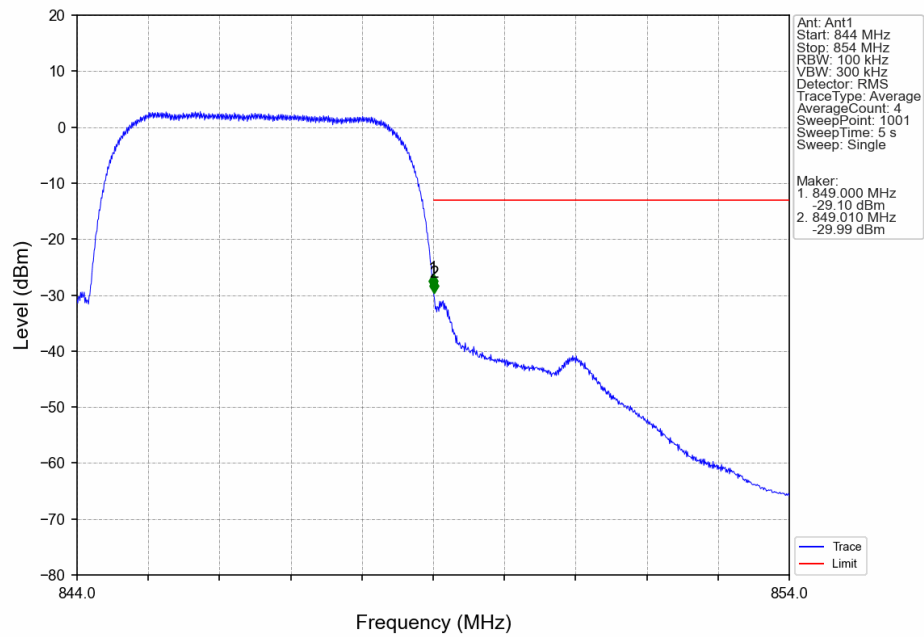
Band5 HSDPA HCH 846.6MHz Subtest 1 NTV
