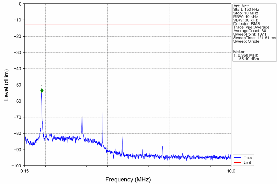
Band5 HSDPA MCH 836.6MHz Subtest 1 NTN
