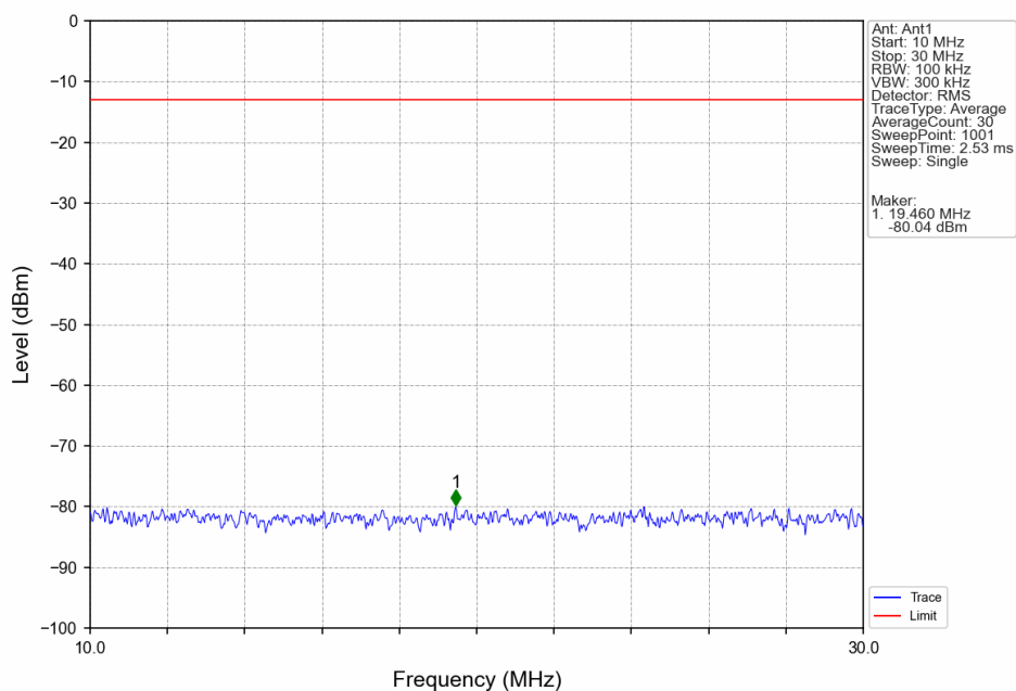
Band5_RMC_LCH_826.4MHz_12.2kbps_RMC_NTNV
