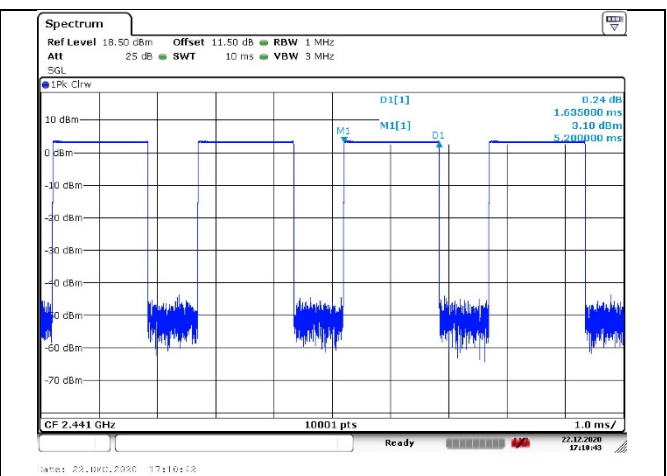
Modulation type: GFSK DH3 2441MHz
