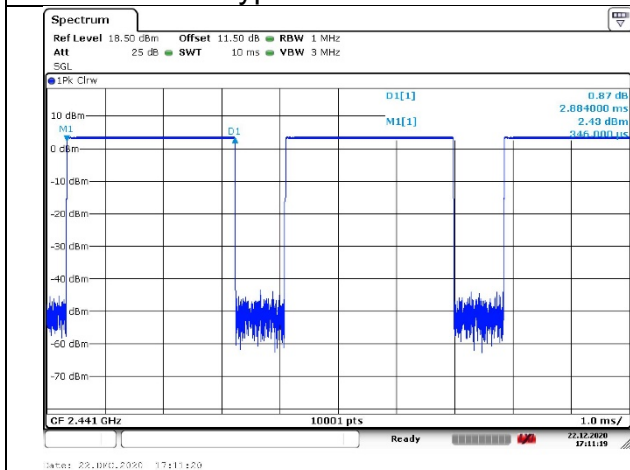
Modulation type: GFSK DH5 2441MHz
