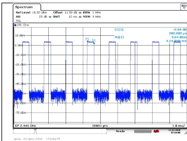
Modulation type: GFSK DH1 2441MHz
