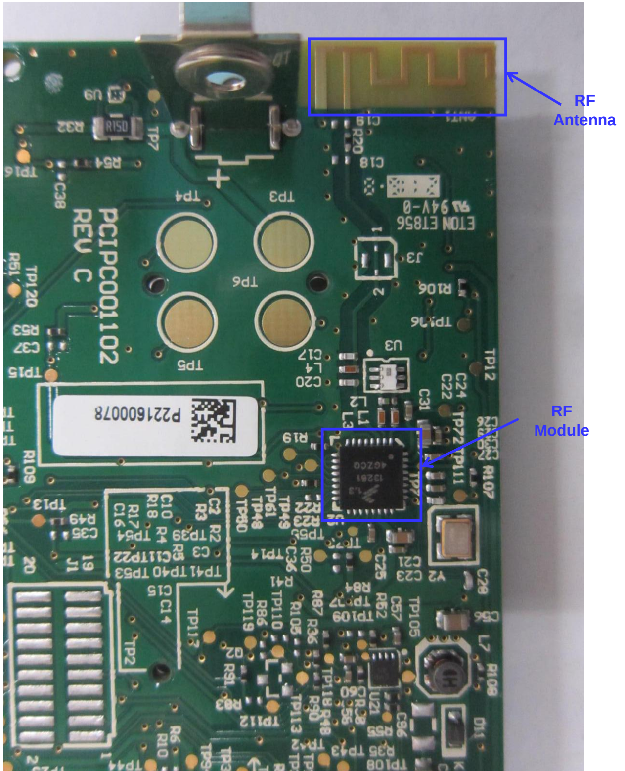
RF Module Circuit with RF Shield Removed
