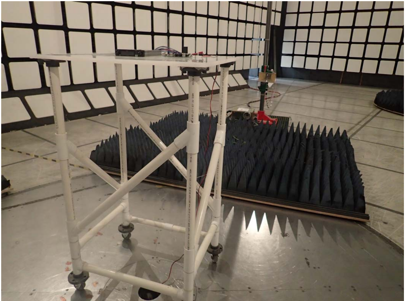
Radiated Emission at 3m Distance (Above 1 GHz)
