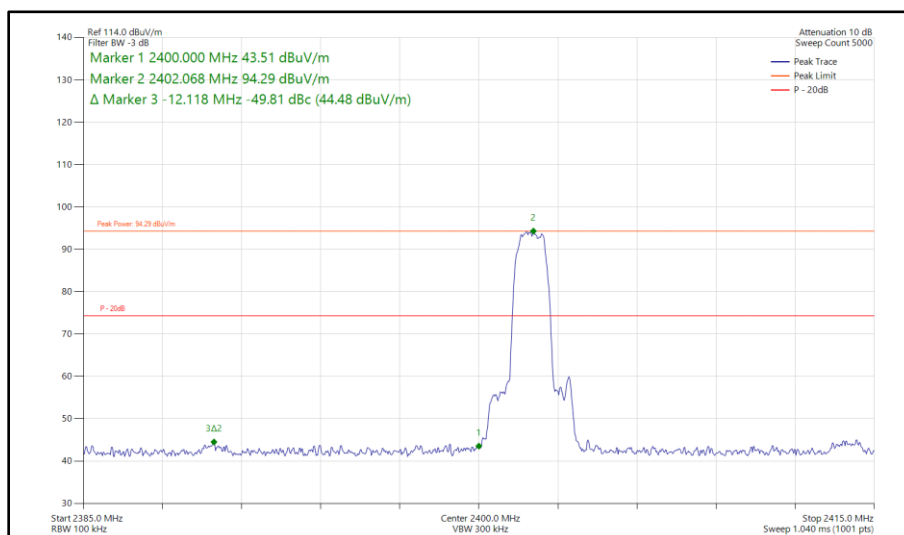
Figure 36 - Bluetooth 3-DH5, SISO, Core 0 - 2402 MHz Band Edge Frequency 2400 MHz
