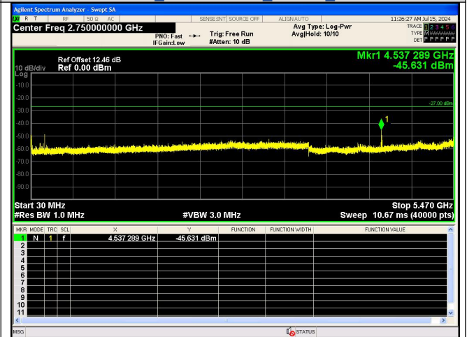
Spurious Emission:30.0~5470 MHz IEEE 802.11n_Channel 134_40MHz_Antenna 0
