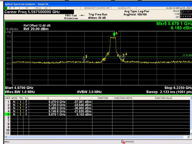
Out Of Band Emission IEEE 802.11n_Channel 134_40MHz_Antenna 0
