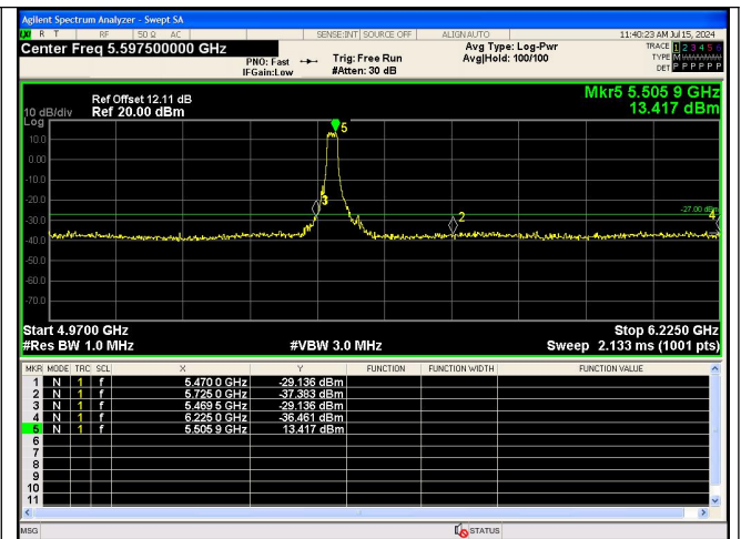
Out Of Band Emission IEEE 802.11ac_Channel 100_20MHz_Antenna 0
