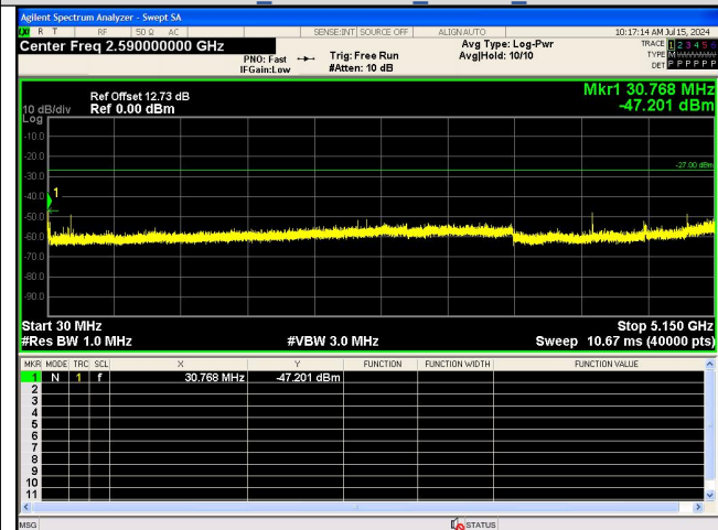
Spurious Emission:30.0~5150 MHz IEEE 802.11ac_Channel 52_20MHz_Antenna 0
