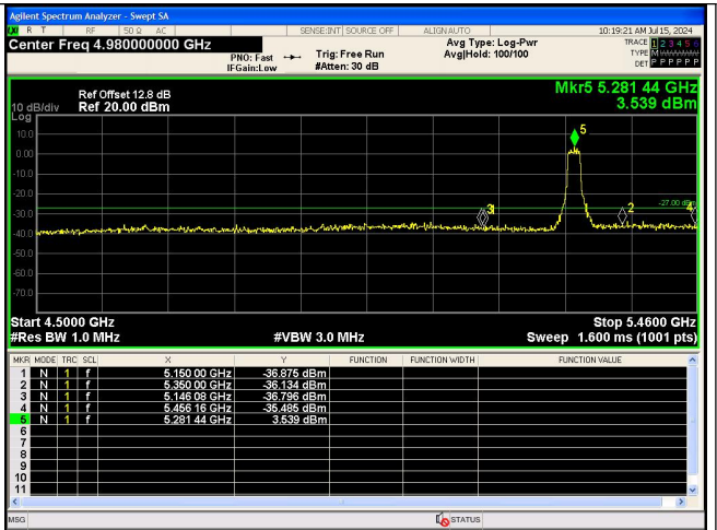
Out Of Band Emission IEEE 802.11ac_Channel 56_20MHz_Antenna 0
