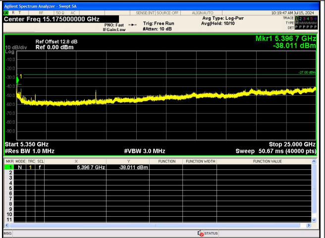
Spurious Emission:5350~25000.0 MHz IEEE 802.11ac_Channel 56_20MHz_Antenna 0
