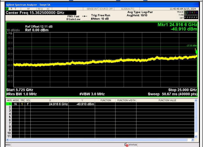
Spurious Emission:5725~25000.0 MHz IEEE 802.11ac_Channel 100_20MHz_Antenna 0
