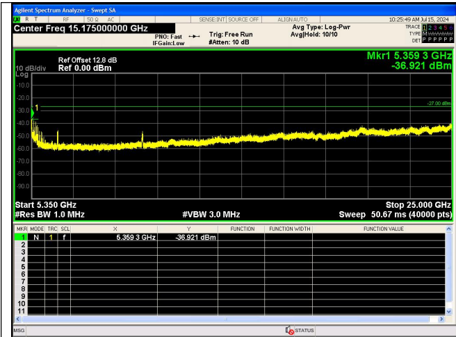
Spurious Emission:5350~25000.0 MHz IEEE 802.11n_Channel 54_40MHz_Antenna 0
