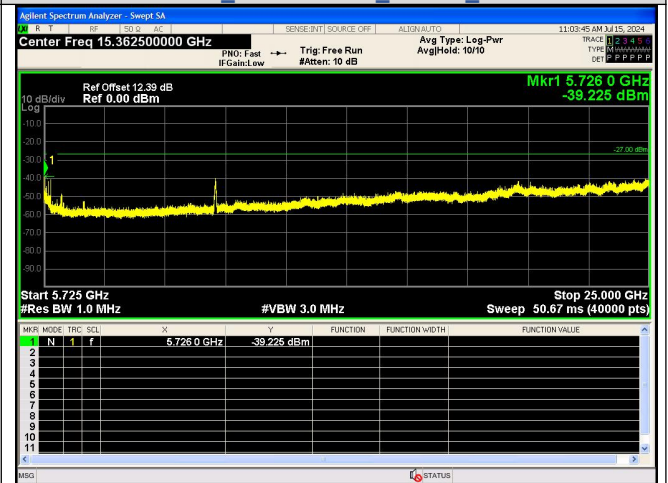
Spurious Emission:5725~25000.0 MHz IEEE 802.11n_Channel 118_40MHz_Antenna 0
