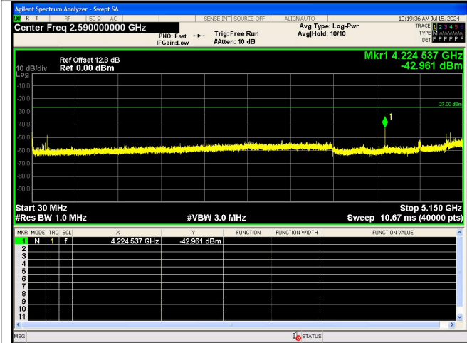
Spurious Emission:30.0~5150 MHz IEEE 802.11ac_Channel 56_20MHz_Antenna 0
