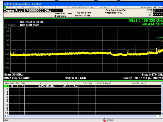
Spurious Emission:30.0~5470 MHz IEEE 802.11n_Channel 118_40MHz_Antenna 0
