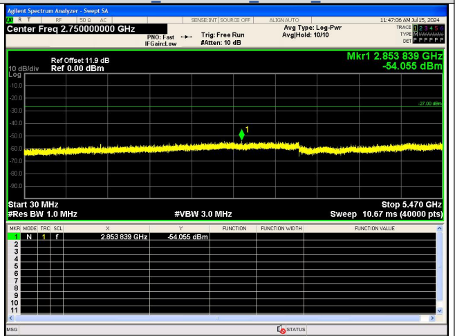
Spurious Emission:30.0~5470 MHz IEEE 802.11n_Channel 102_40MHz_Antenna 0
