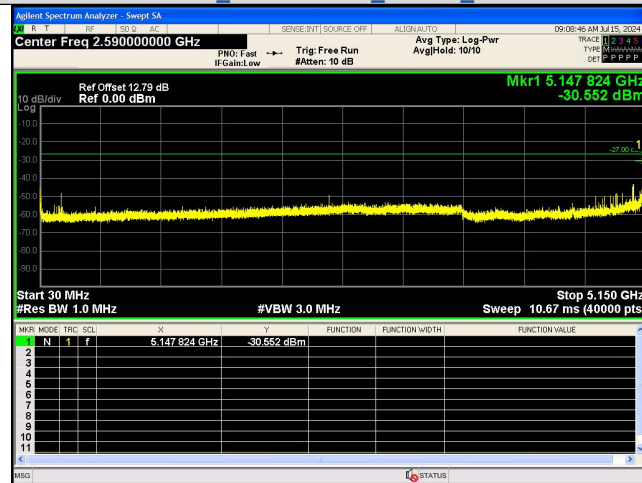
Spurious Emission:30.0~5150 MHz IEEE 802.11ac_Channel 36_20MHz_Antenna 0
