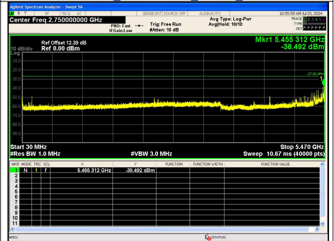
Spurious Emission:30.0~5470 MHz IEEE 802.11ac_Channel 120_20MHz_Antenna 0
