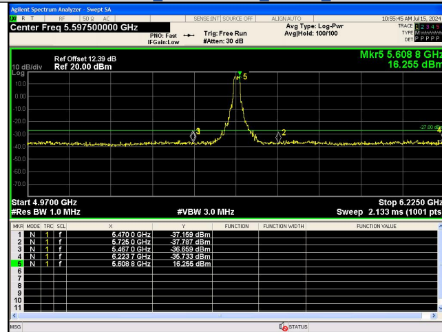
Out Of Band Emission IEEE 802.11ac_Channel 120_20MHz_Antenna 0
