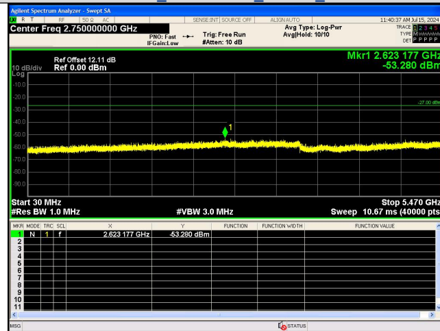
Spurious Emission:30.0~5470 MHz IEEE 802.11ac_Channel 100_20MHz_Antenna 0
