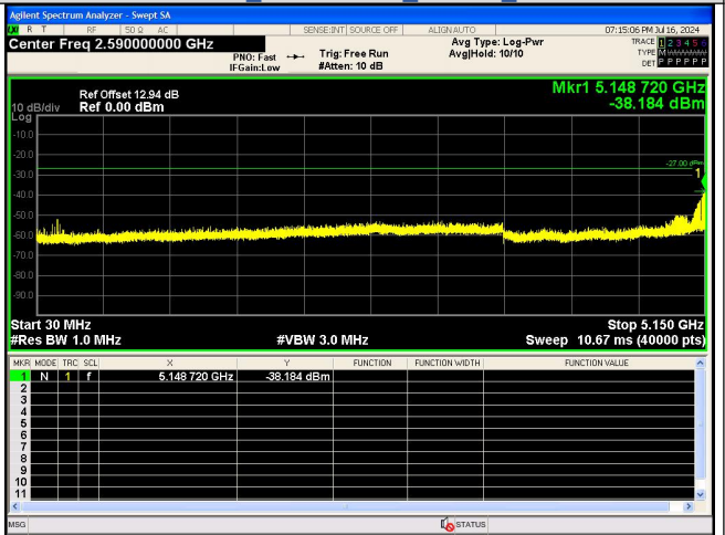
Spurious Emission:30.0~5150 MHz IEEE 802.11ac_Channel 64_20MHz_Antenna 0
