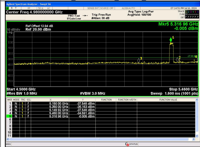
Out Of Band Emission IEEE 802.11ac_Channel 64_20MHz_Antenna 0
