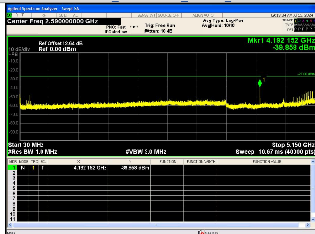
Spurious Emission:30.0~5150 MHz IEEE 802.11ac_Channel 48_20MHz_Antenna 0
