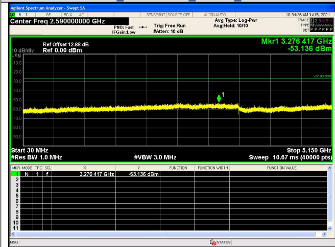
Spurious Emission:30.0~5150 MHz IEEE 802.11n_Channel 62_40MHz_Antenna 0
