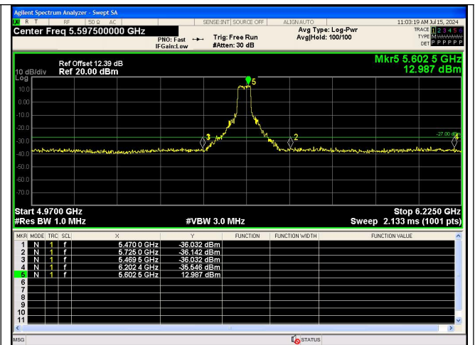
Out Of Band Emission IEEE 802.11n_Channel 118_40MHz_Antenna 0
