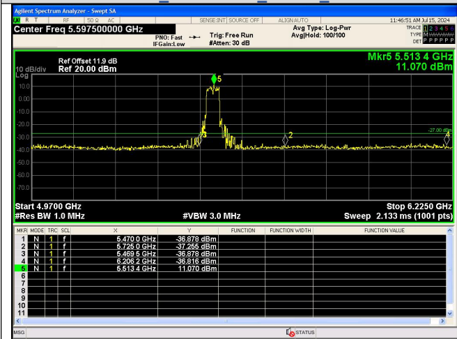
Out Of Band Emission IEEE 802.11n_Channel 102_40MHz_Antenna 0
