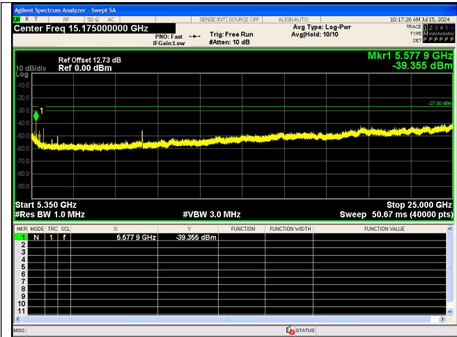
Spurious Emission:5350~25000.0 MHz IEEE 802.11ac_Channel 52_20MHz_Antenna 0
