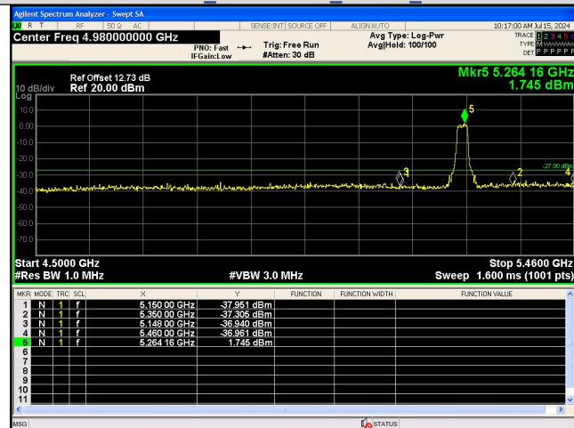
Out Of Band Emission IEEE 802.11ac_Channel 52_20MHz_Antenna 0
