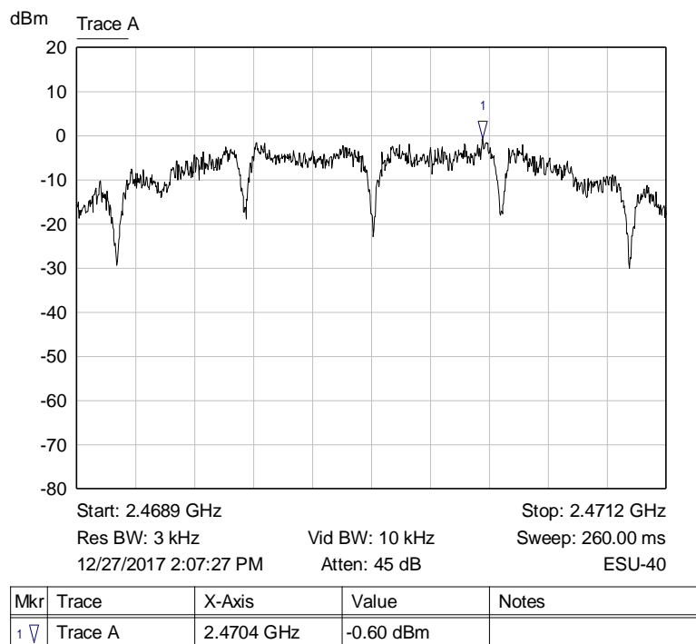
Graph 17: Channel 24 3 kHz PSD Plot (2470 MHz)
