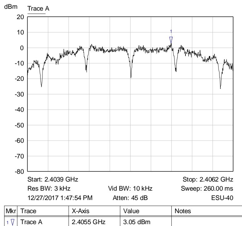
Graph 15: Lowest Channel 3 kHz PSD Plot (2405 MHz)
