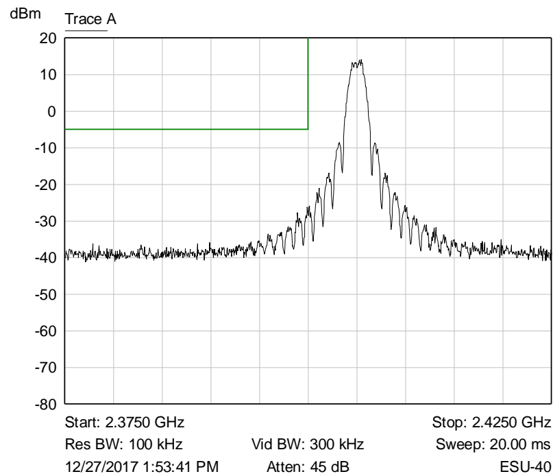
Graph 9: Channel 11 Lower Band Edge Plot (2405 MHz)
