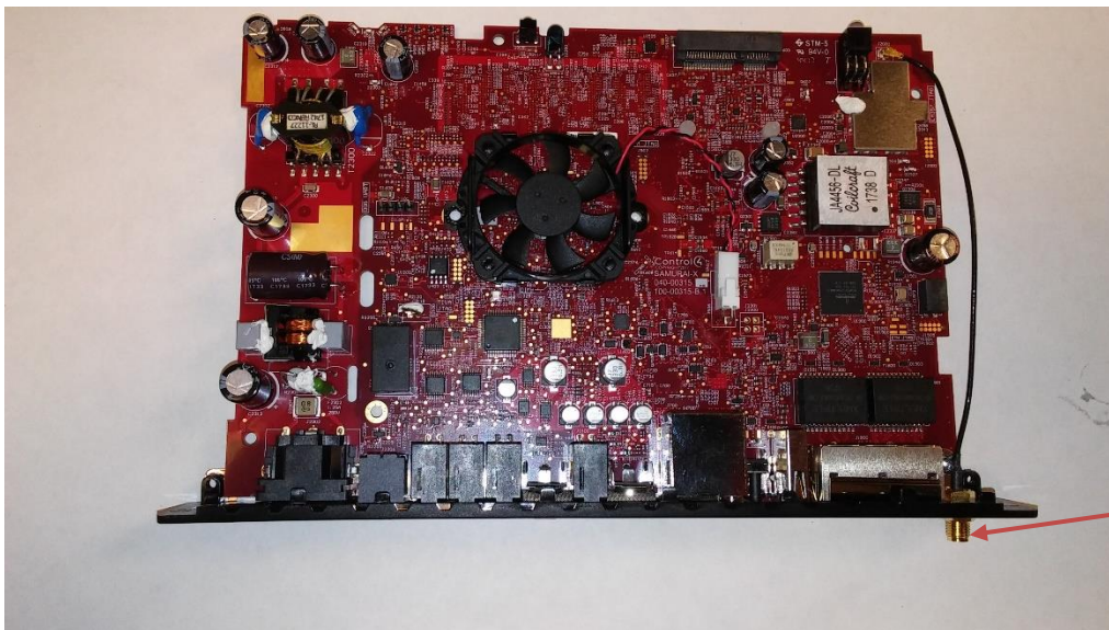
Photograph 12 – Top Side of the PCB with Shield
