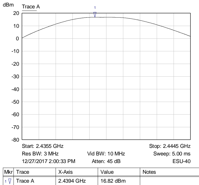
Graph 6: Middle Channel Peak Output Power (2440 MHz)
