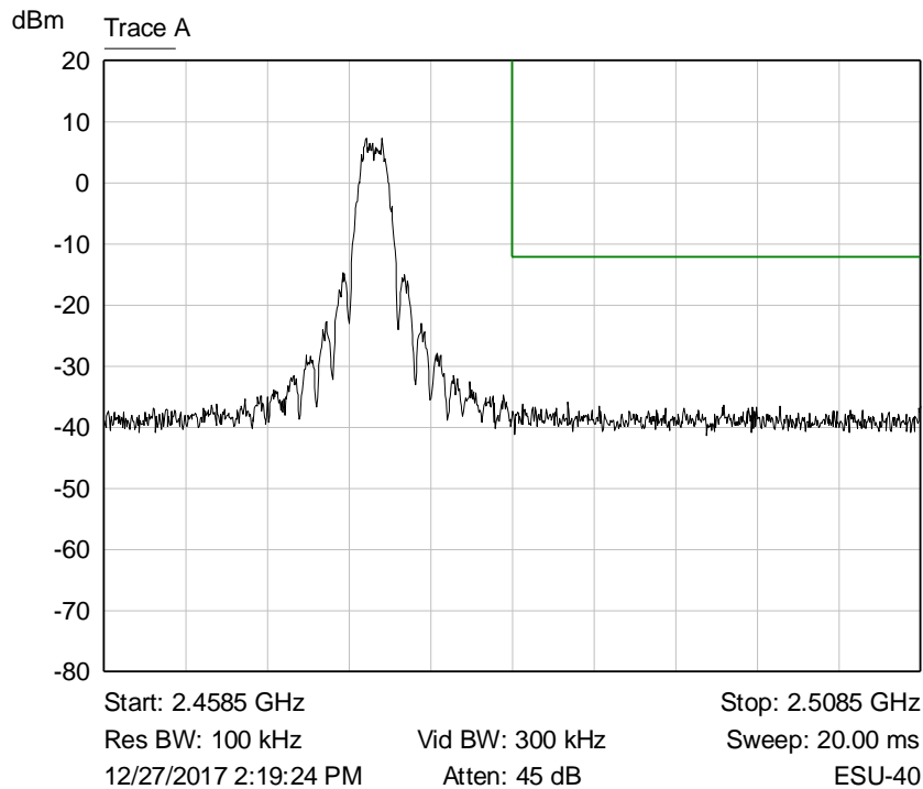
Graph 11: Channel 25 Upper Band Edge Plot (2475 MHz)
