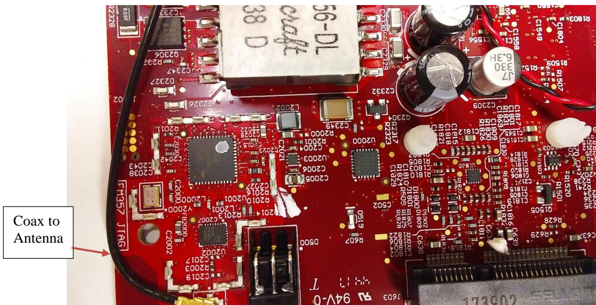
Photograph 13 – Circuitry Under RF Shield
