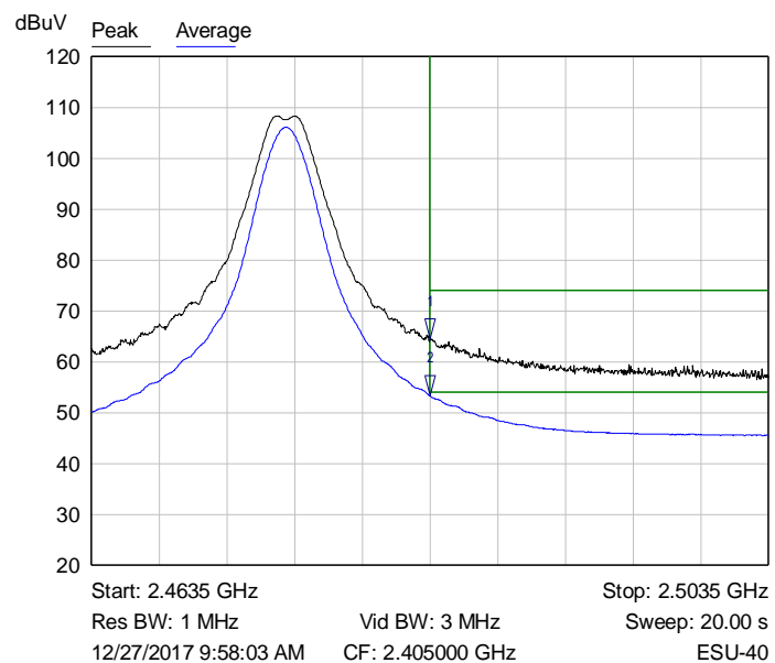
Graph 13: Radiated Channel 24 Upper Band Edge Plot (2470 MHz)
