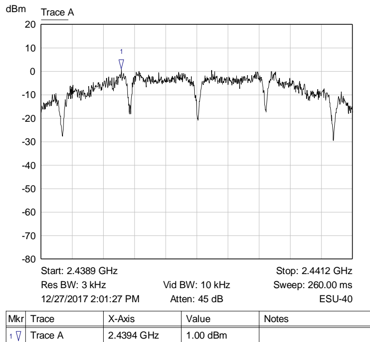
Graph 16: Middle Channel 3 kHz PSD Plot (2440 MHz)
