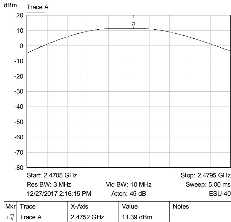
Graph 8: Highest Channel Peak Output Power Plot (2475 MHz)
