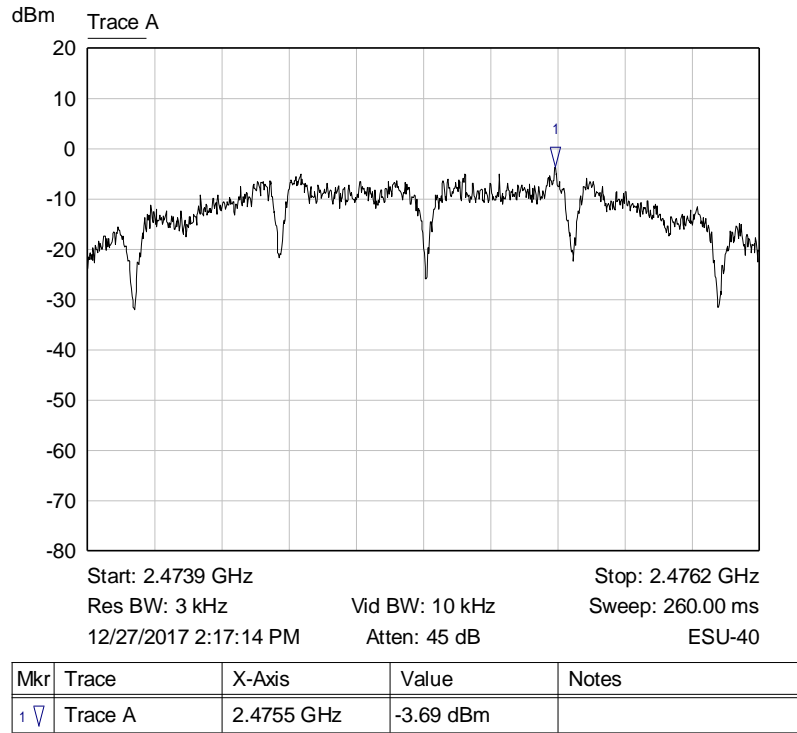
Graph 18: Highest Channel 3 kHz PSD Plot (2475 MHz)
