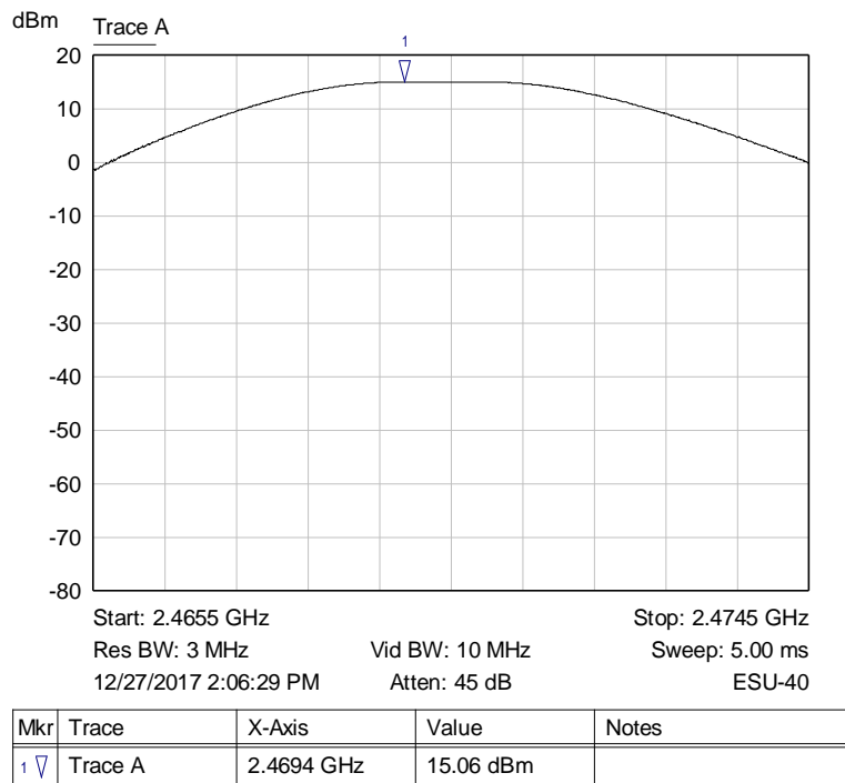
Graph 7: Channel 24 Peak Output Power (2470 MHz)
