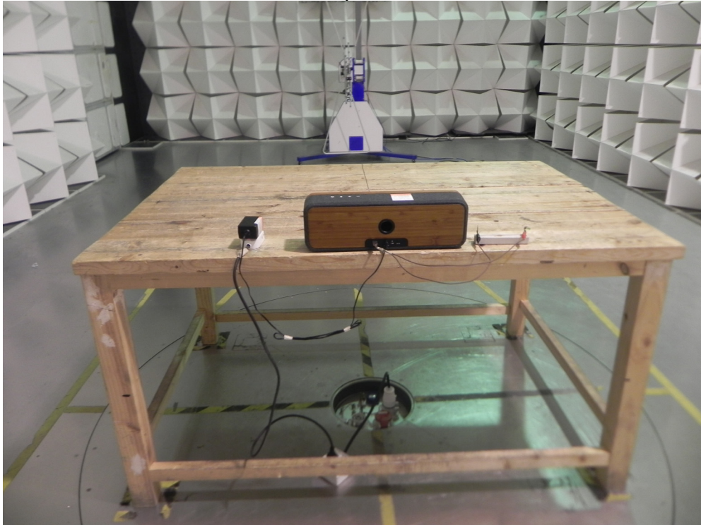
Adapter 2
