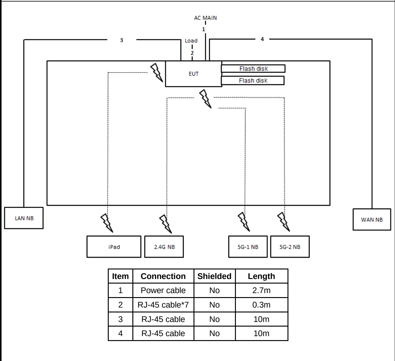
Test Setup Diagram - Radiated Test < 1GHz
