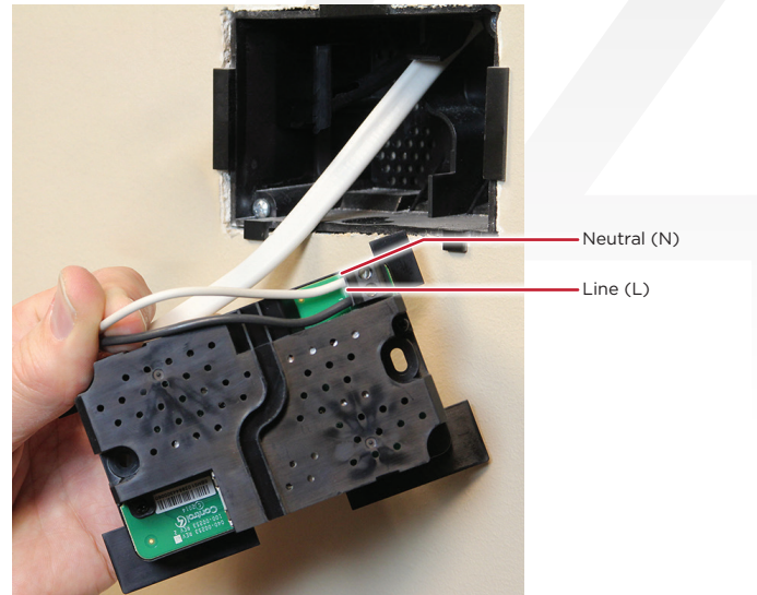
Figure 9: Connect AC power
