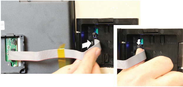
Figure 11: Attach ribbon cable to the power box
