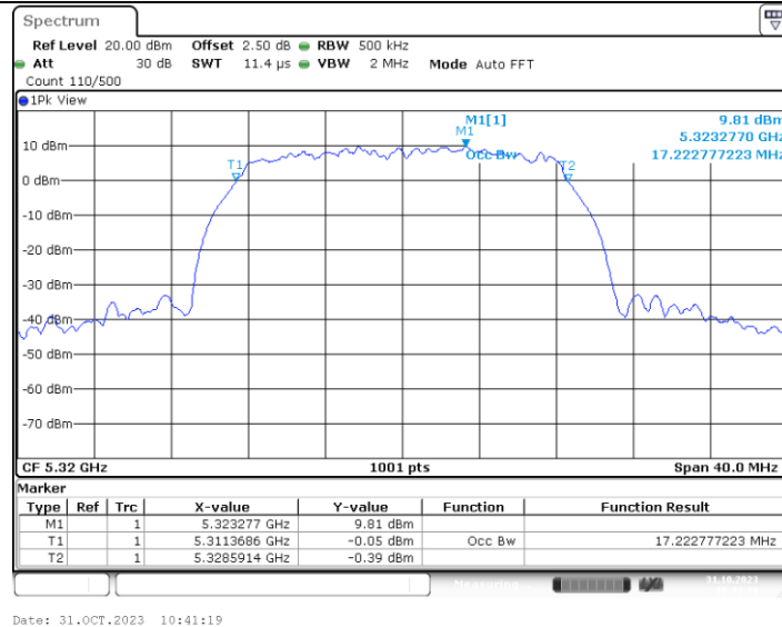
11A_Ant4_5320
