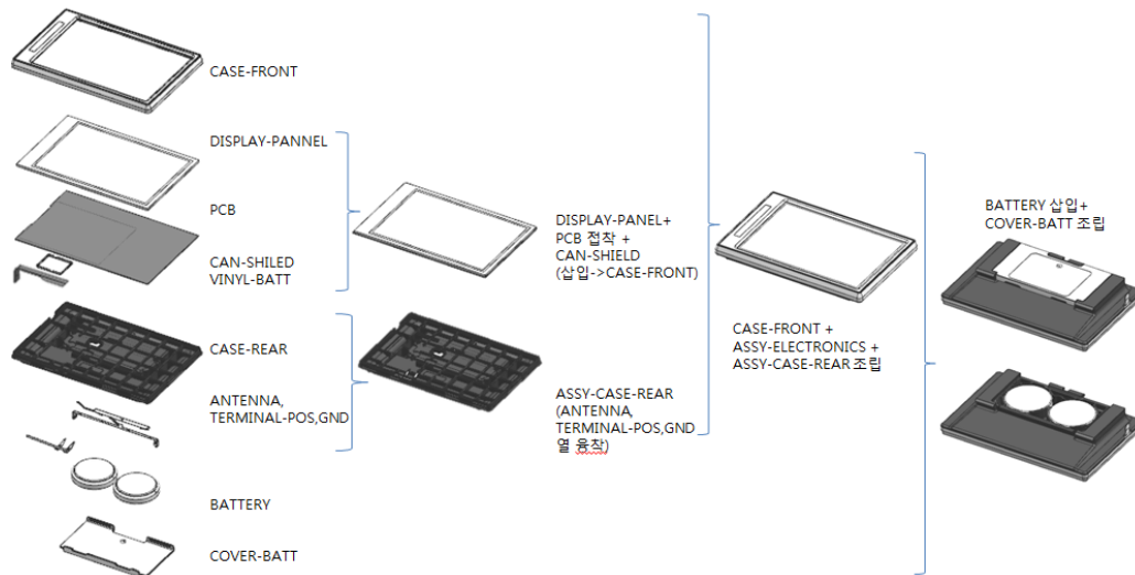
Figure 4 Exploded View
