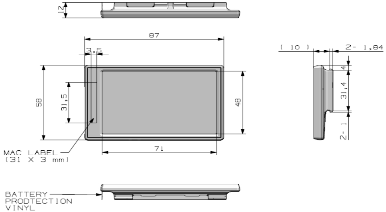
Figure 3 Mechanical Dimension
