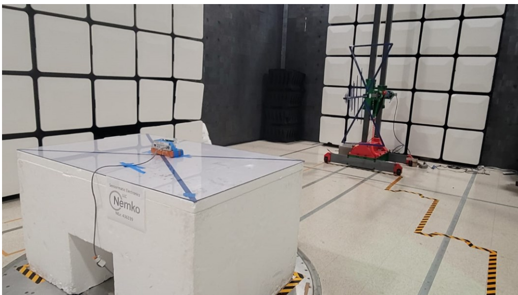
Figure 2 - Radiated emissions below 1 GHz (0.03 – 1 GHz), rear view, 3 meters distance.
