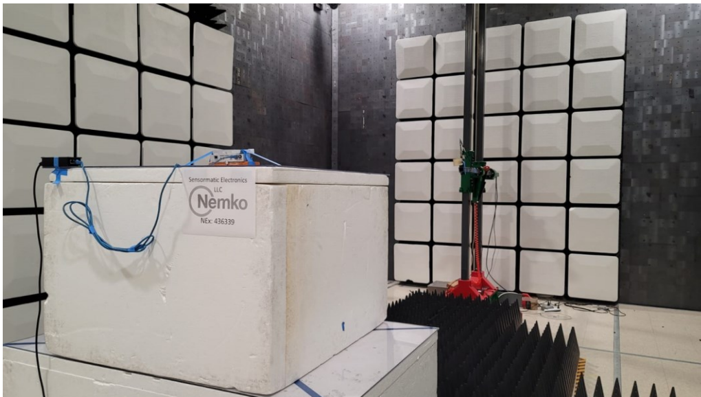
Figure 6 - Radiated emissions above 1 GHz (18 – 26 GHz), rear view, 3 meters distance.
