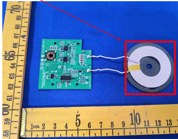
Coil ANT
