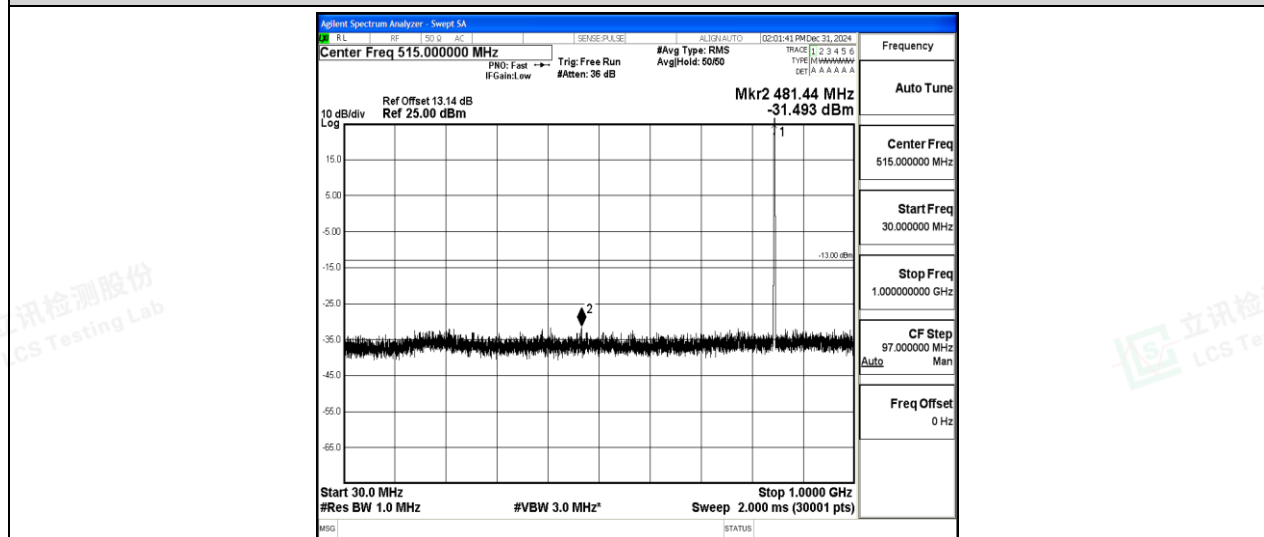
Band5-3MHz-QPSK-20635-1-0-High-30-1000--31.49-PASS
