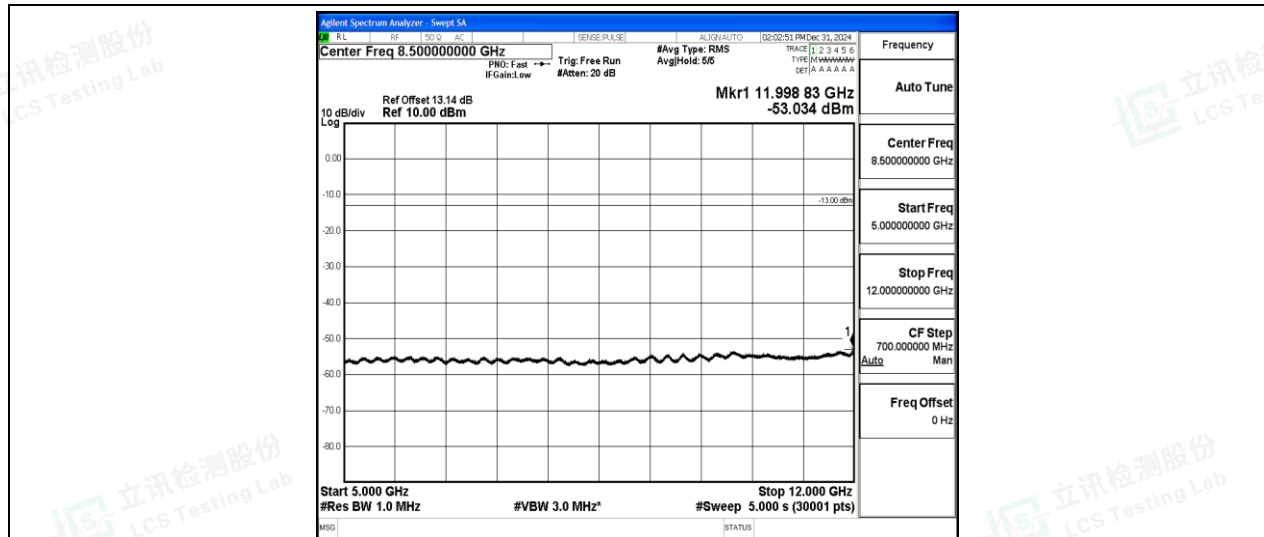
Band5-3MHz-QPSK-20635-1-0-High-5000-12000--53.03-PASS
