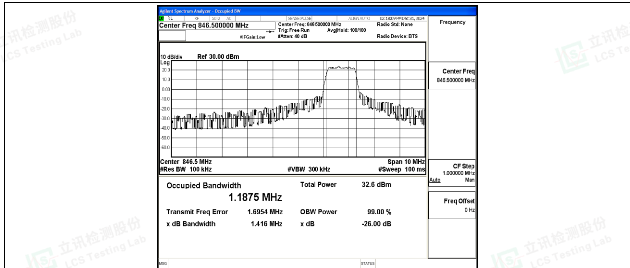
Band5-5MHz-16QAM-20625-6-0-High-1.1875-1.416-PASS
