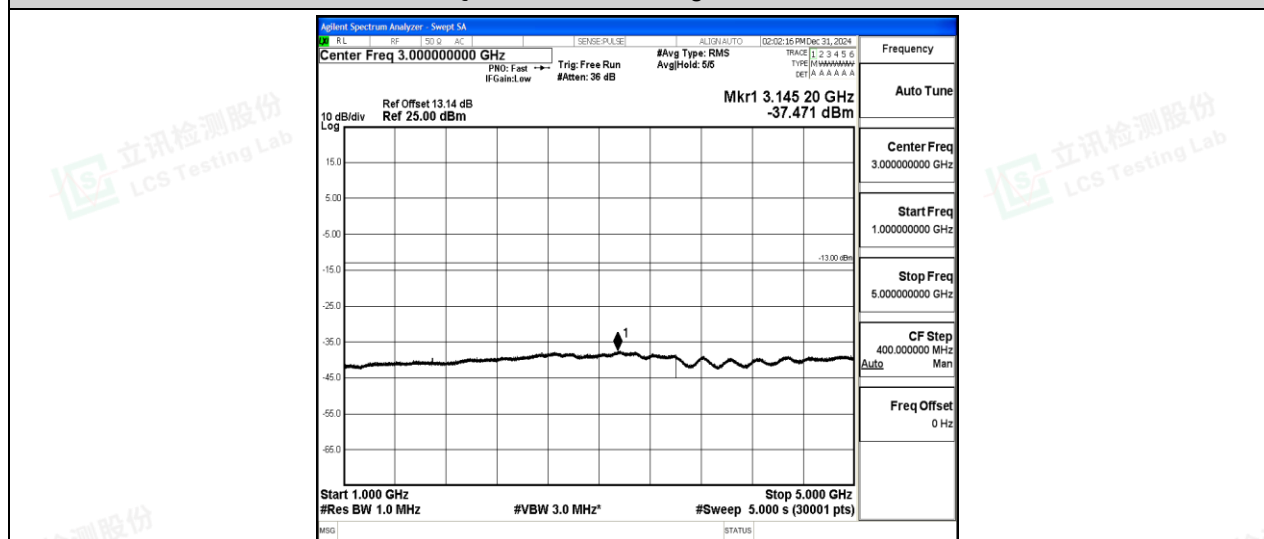
Band5-3MHz-QPSK-20635-1-0-High-1000-5000--37.47-PASS
