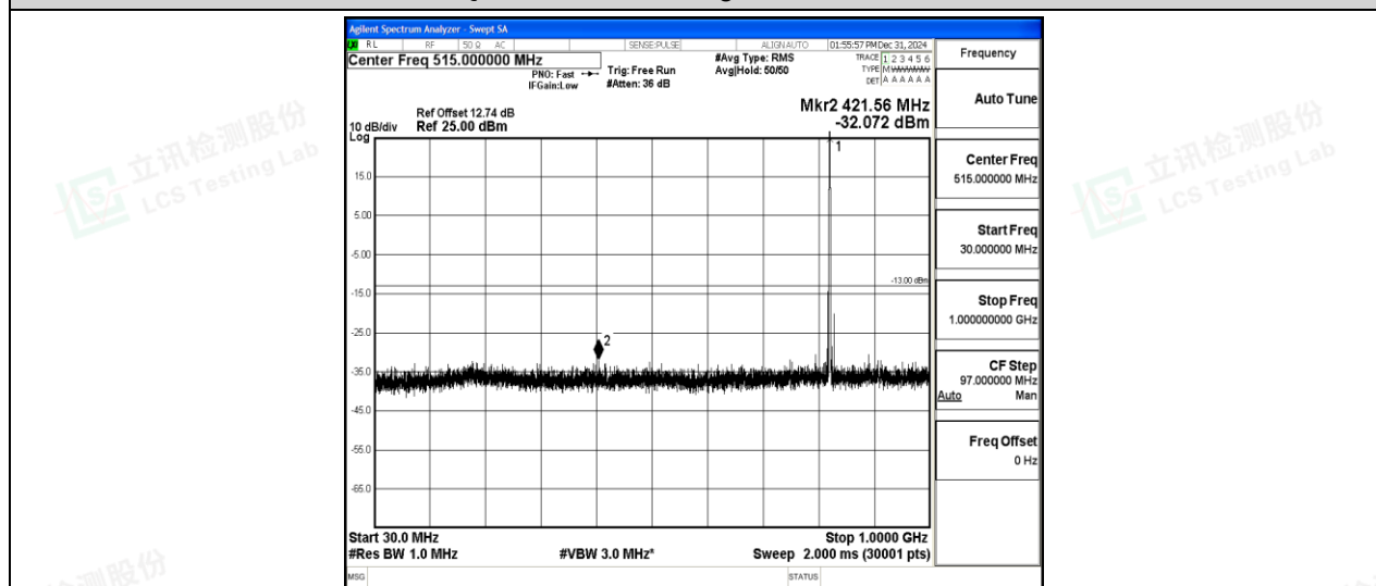
Band5-3MHz-16QAM-20415-1-0-Low-30-1000--32.07-PASS
