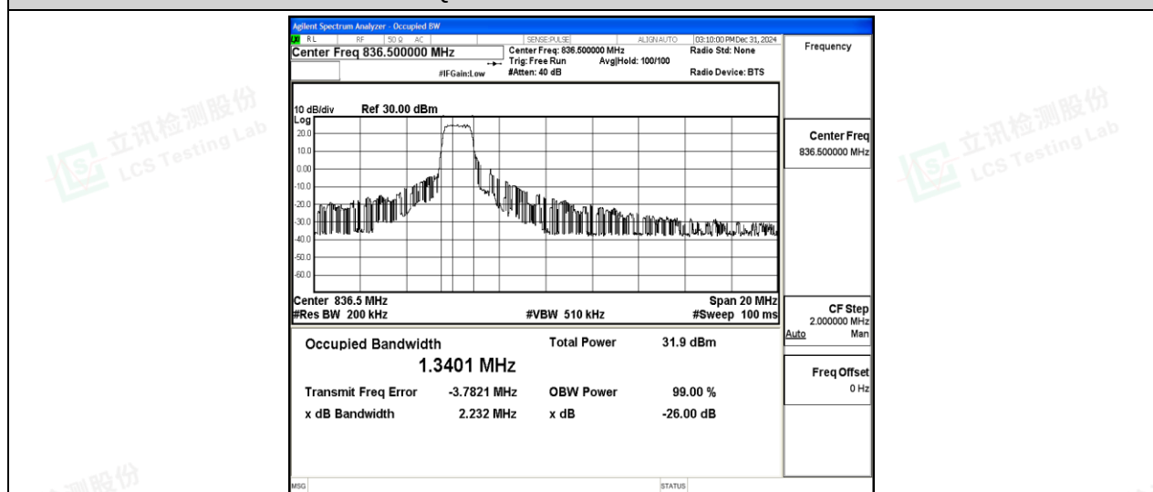
Band5-10MHz-QPSK-20525-6-0-Low-1.3401-2.232-PASS
