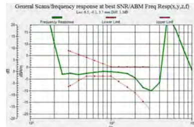
GSM1900, Antenna 1
