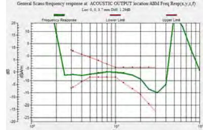
GSM1900, Antenna 1
