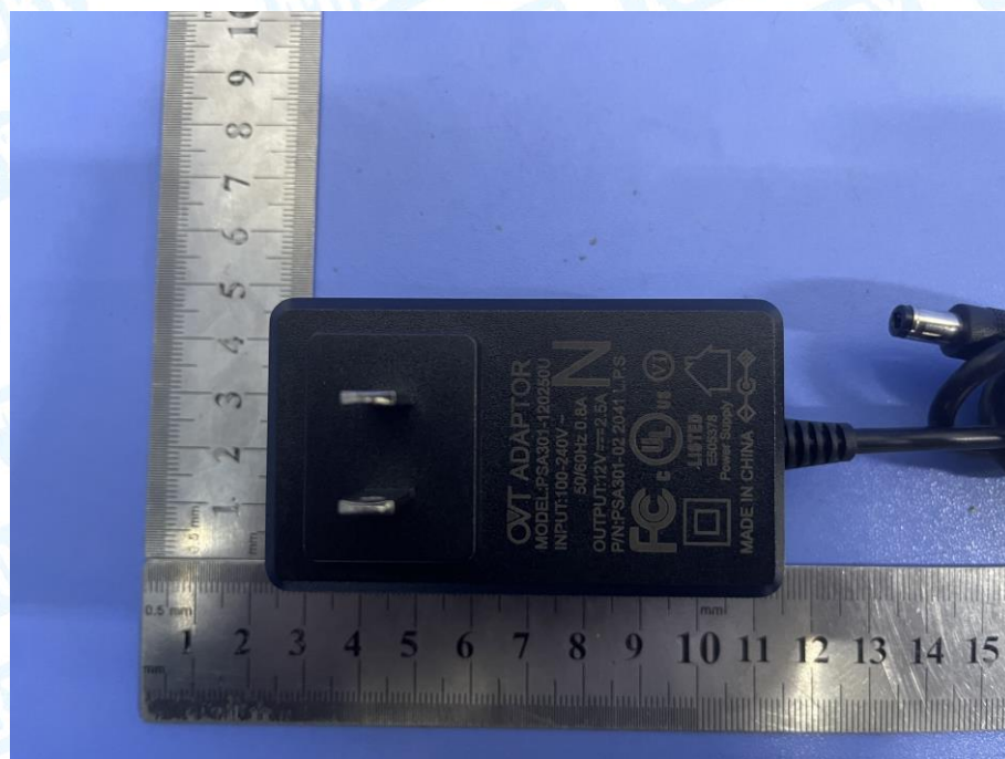
Photo 8 Appearance of Adapter 1#
