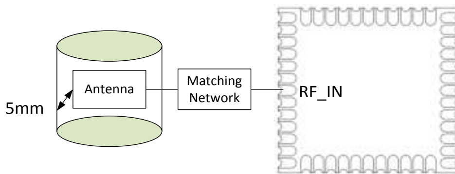
Figure 9: Leave 5mm Clearance Space from the Antenna
