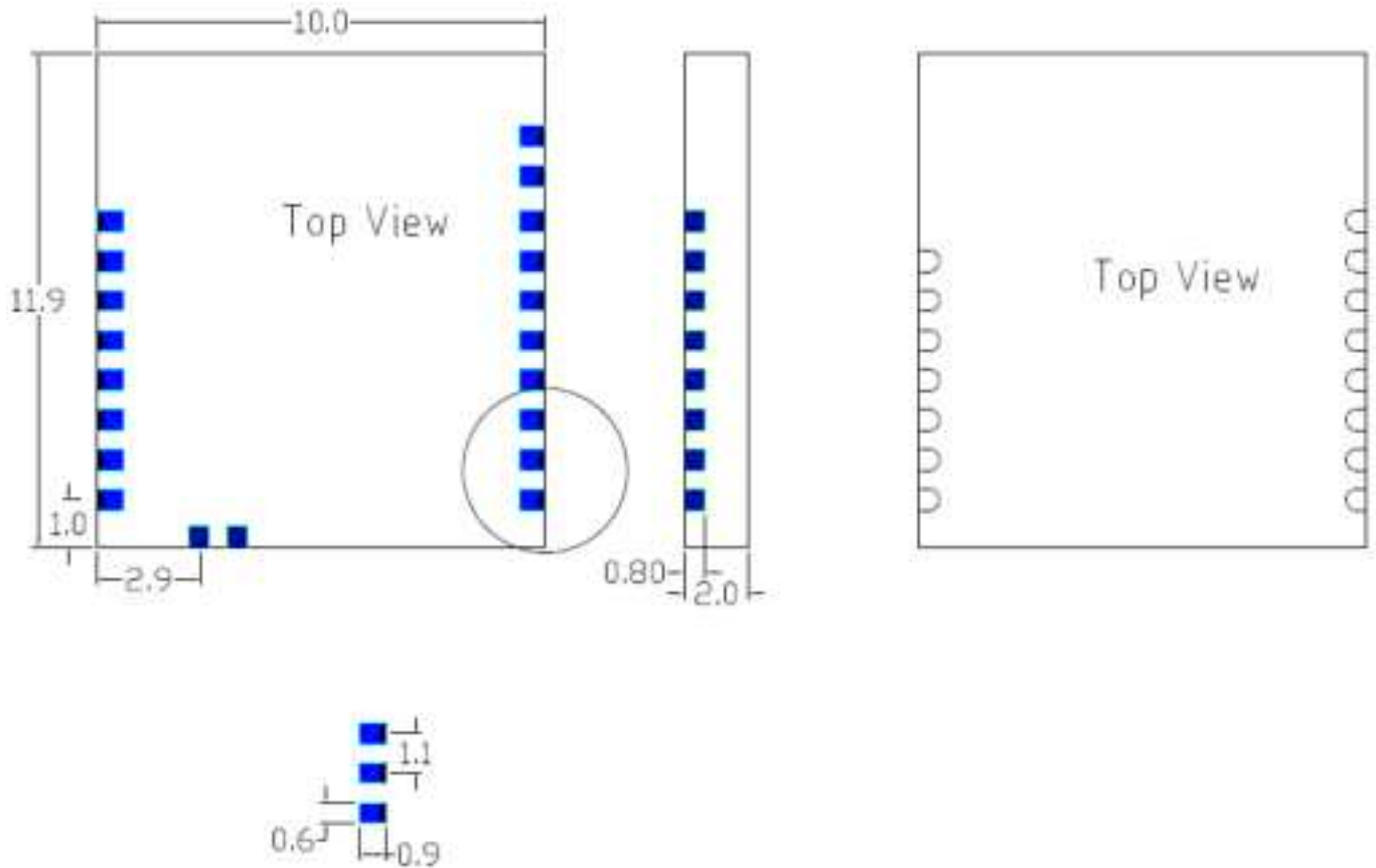
Figure 6: FSC-BT691 footprint
