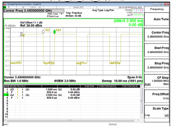
GFSK 1M DH3 2480MHz
