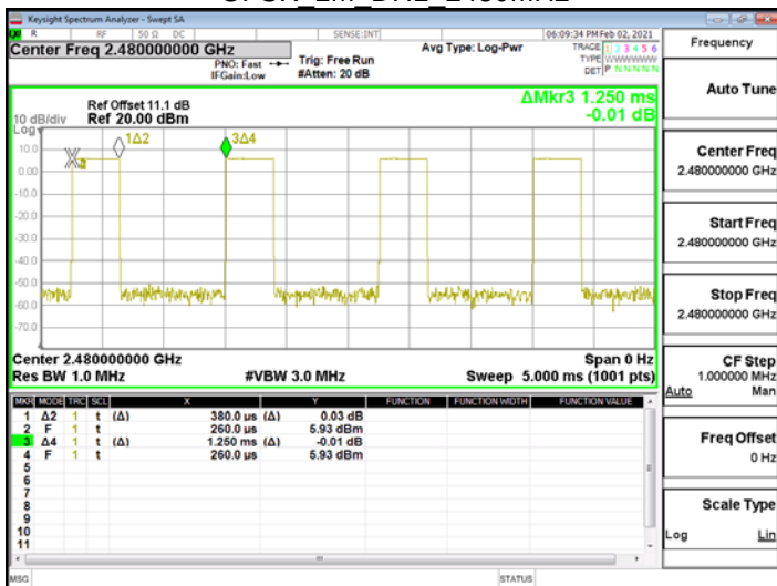
GFSK 1M DH1 2480MHz
