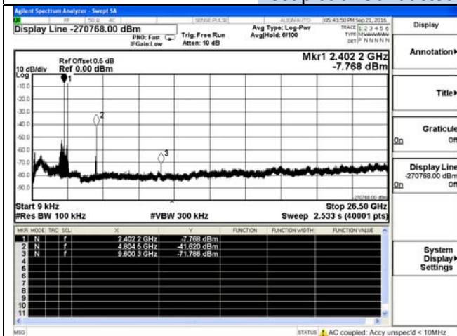
DH1-Low channel
