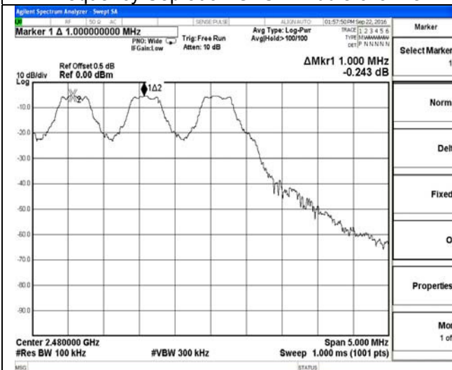
Frequency Separation GFSK-High channel
