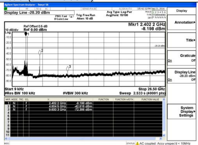
2DH1-Low channel
