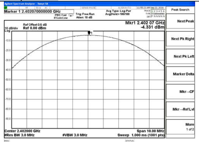
2DH1-Low channel
