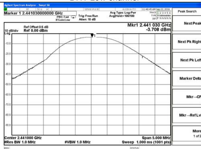
DH1-Middle channel
