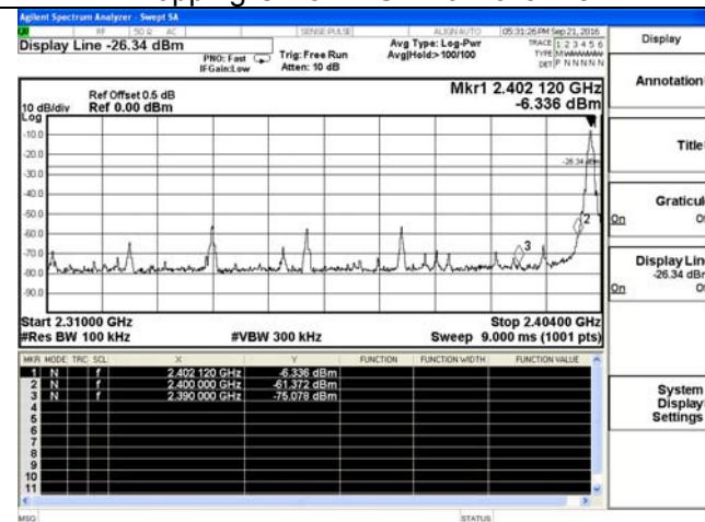
Hopping Off-8-DPSK-Low channel
