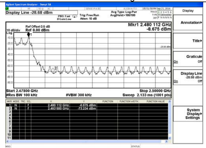
Hopping On-8-DPSK-High channel
