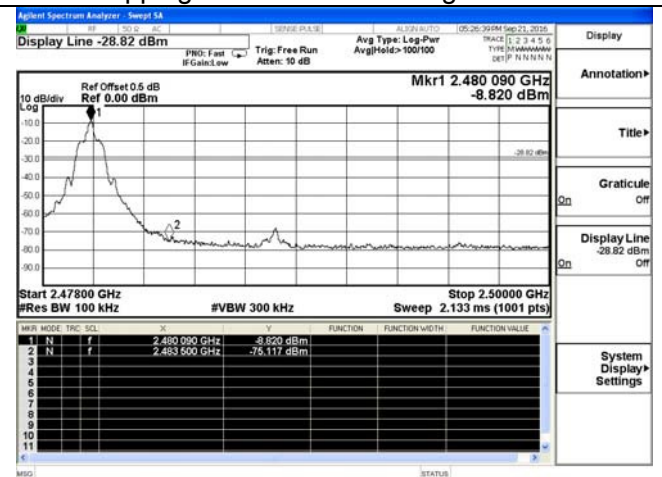
Hopping Off- \pi/4 -DQPSK-High channel
