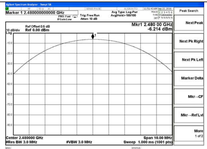
2DH1-High channel
