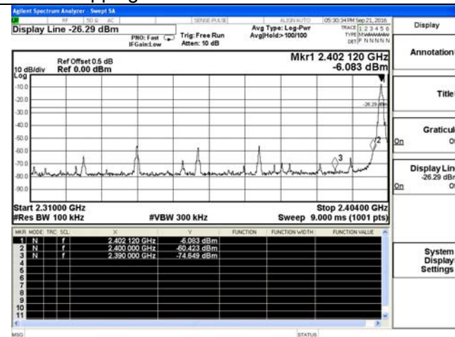
Hopping Off- \pi/4 -DQPSK-Low channel
