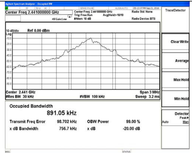
20dB Bandwidth GFSK-Middle channel
