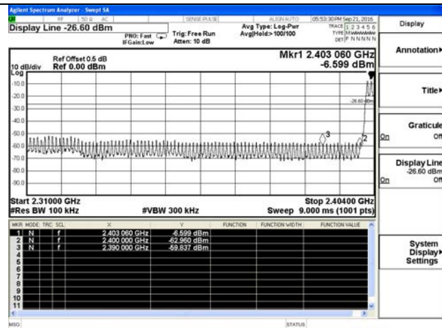
Hopping On-8-DPSK-Low channel
