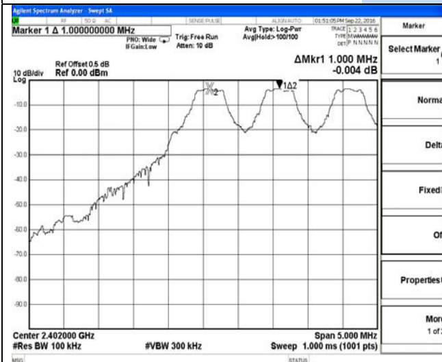
Frequency Separation GFSK-Low channel
