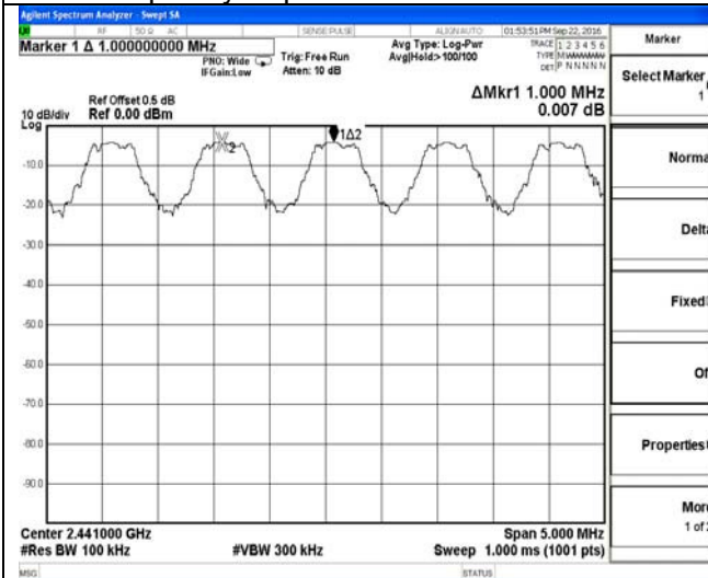
Frequency Separation GFSK-Middle channel
