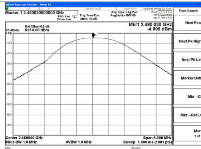
DH1-High channel
