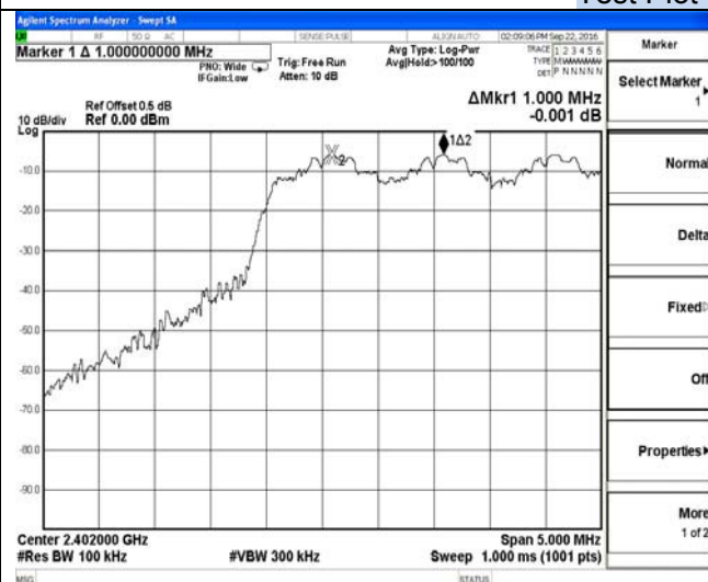
Frequency Separation 8-DPSK-Low channel
