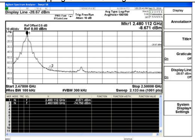
Hopping Off-8-DPSK-High channel
