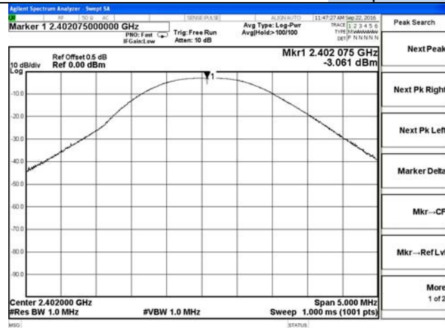
DH1-Low channel
