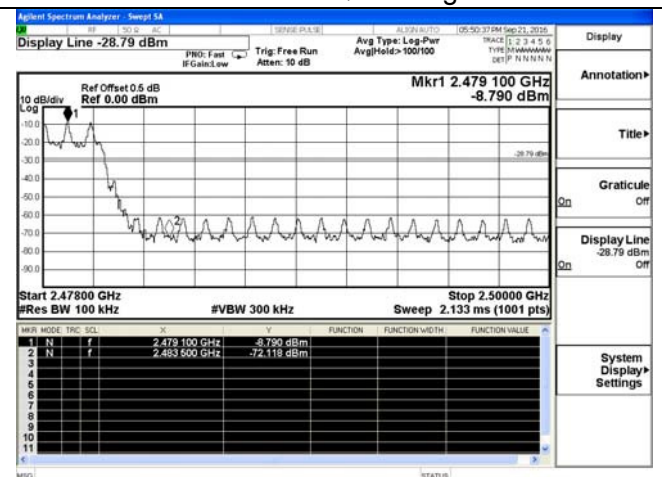
Hopping On- \pi/4 -DQPSK-High channel
