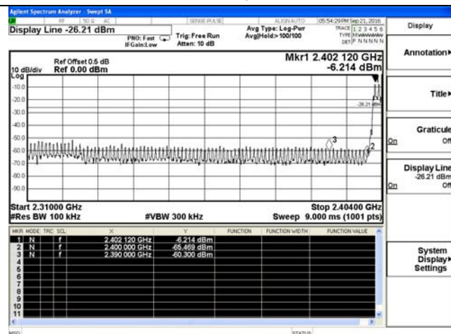
Hopping On- \pi/4 -DQPSK-Low channel
