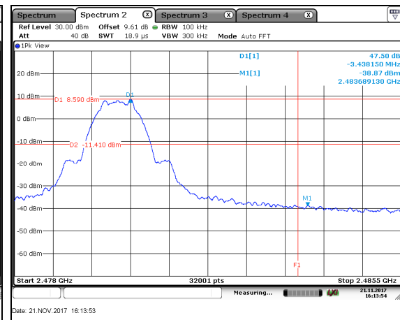
Figure 7.4.1.2-6: Upper Band-edge - HCH
