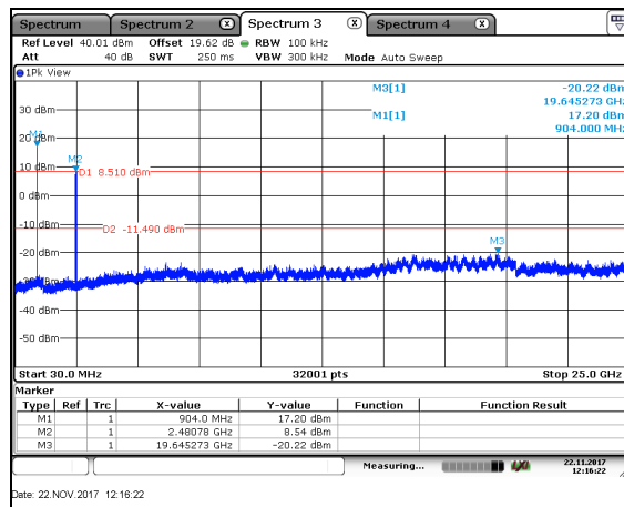
Figure 7.4.1.2-4: Cond. Emissions – Simultaneous Tx
